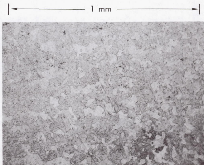
1100-0 ALUMINUM
