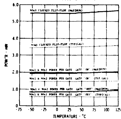
POWER CHARACTERISTICS V_{CC} = 5V EMITTER FOLLOWER PULL UP
