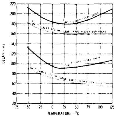
TYPICAL DELAY CHARACTERISTICS LPDT \mu L 9040
