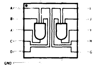
FLAT PACKAGE LAYOUT
