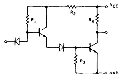
SCHEMATIC DIAGRAM — ONE INVERTER ONLY DT μ L 9936 • DT μ L 9937
