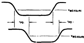
WAVE FORMS
