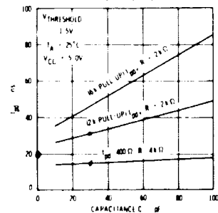
TIME DELAY VERSUS CAPACITIVE LOADS
