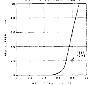
FORWARD VOLTAGE VERSUS FORWARD CURRENT +25°C
