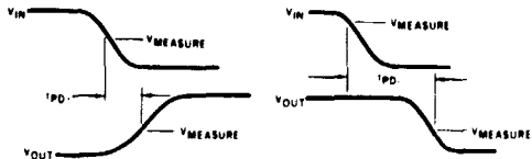
WAVE FORMS
