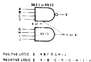
LOGIC EXAMPLE
