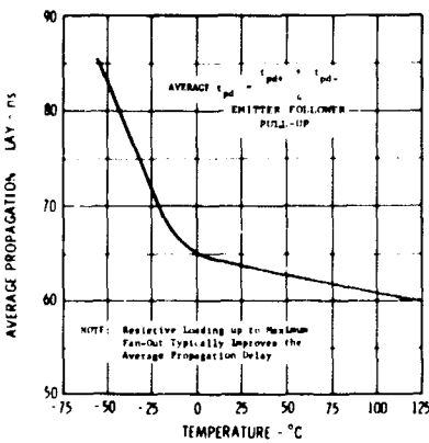
TYPICAL AVERAGE PROPAGATION DELAY LPDT \mu L 9041-9042
