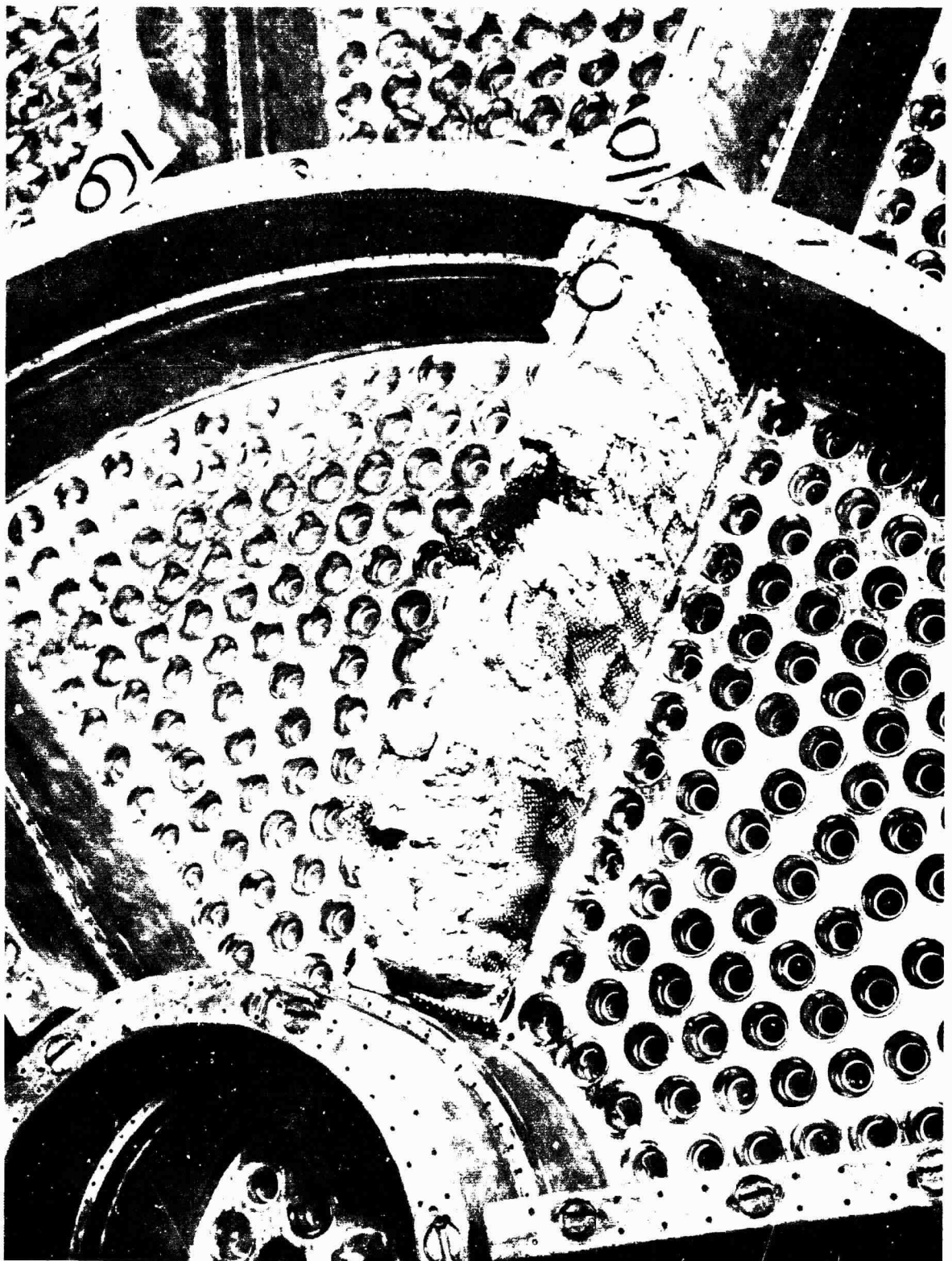
Figure 16. Inner Ablative Buff Erosion After 132 sec. of Steady-State Testing.
