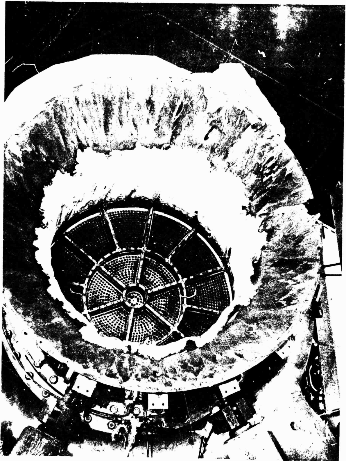
Figure 15. Damage to Nozzle Steel Shell Following Test No. 1198-D01-0C-020
