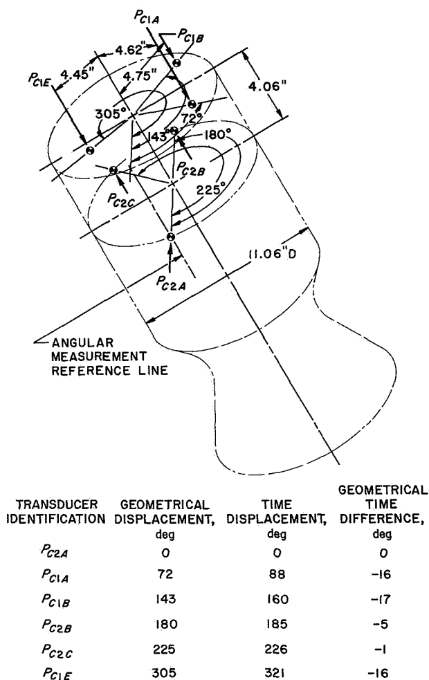
Fig. 15. Phase measurements for resonant combustion for RMIR Injector 7 with N_2O_4 and N_2H_4 as propellants
