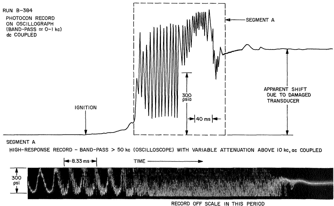
Fig. 1. Typical high-response records of resonant mode obtained in early RMIR injector experiments
