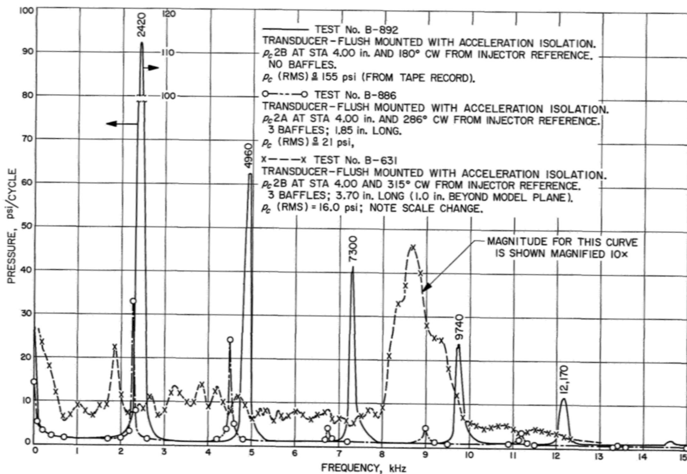
Fig. 11. Spectrum analysis for RMIR Injector 7 with N_2O_4 + N_2H_4 with and without baffles
