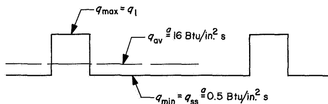
Fig. 19. Idealized wave form
