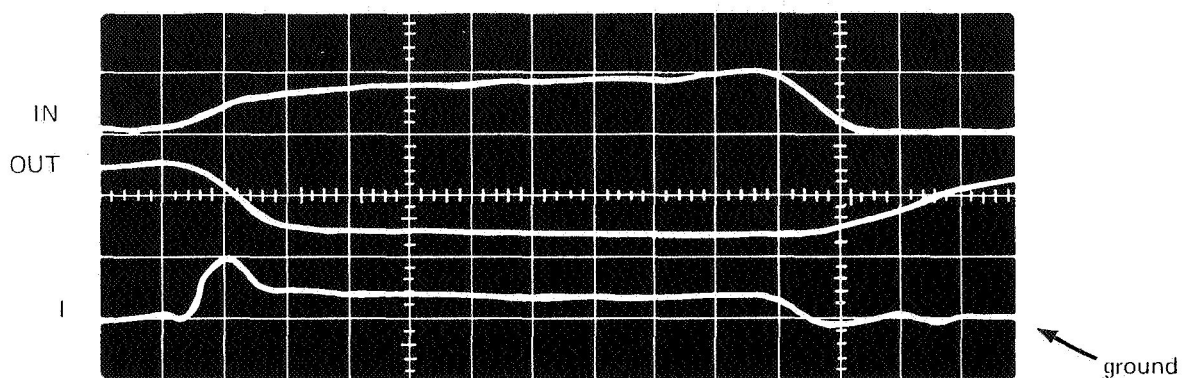
2N 4351 N-channel
