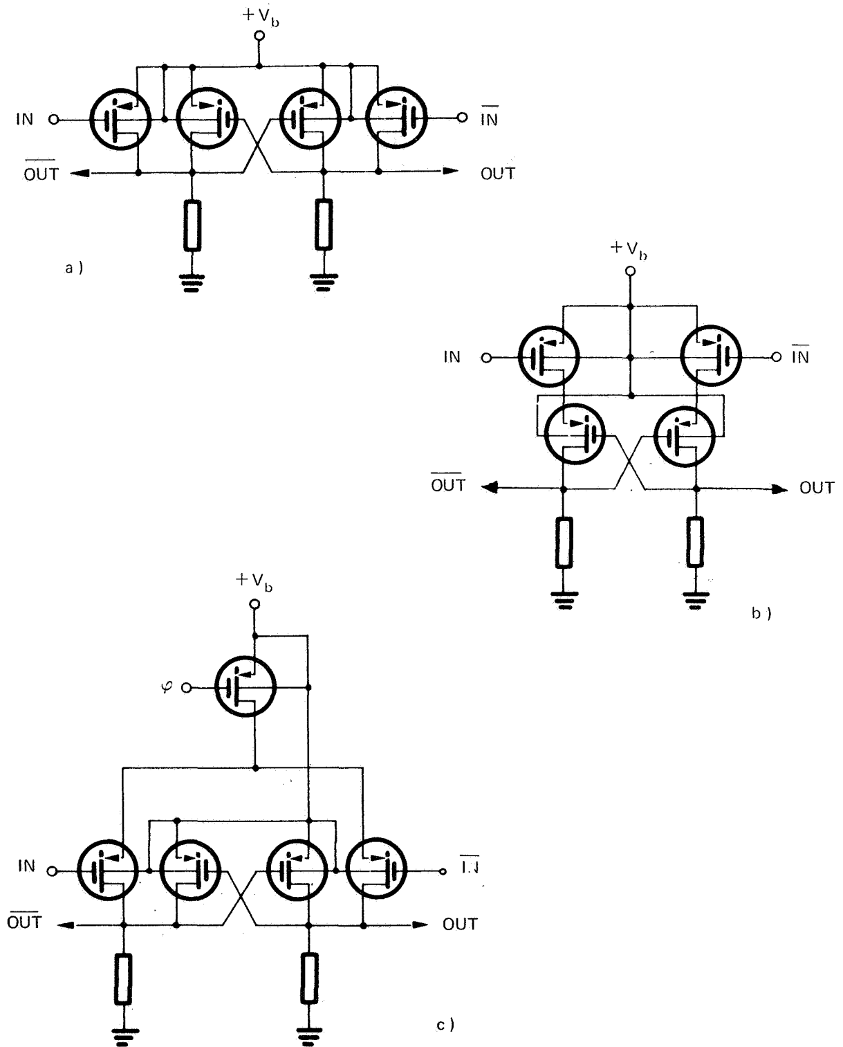
Figure 12.- a and b : R-S-flip-flop; c : D-Type flip-flop.
