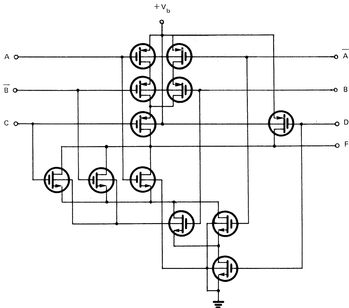
Figure 11. - Implementation of the function F with complementary MOSFETs.
