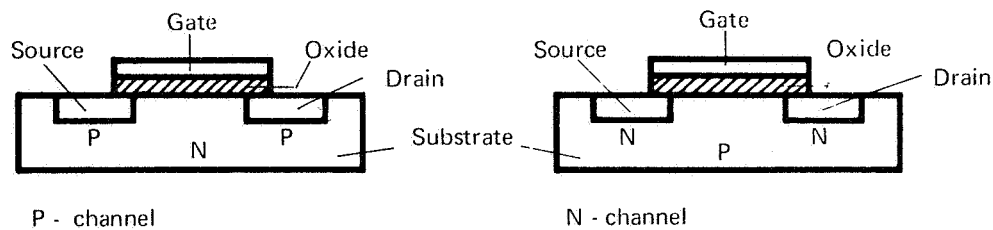
Figure 2.- MOSFET structure.
