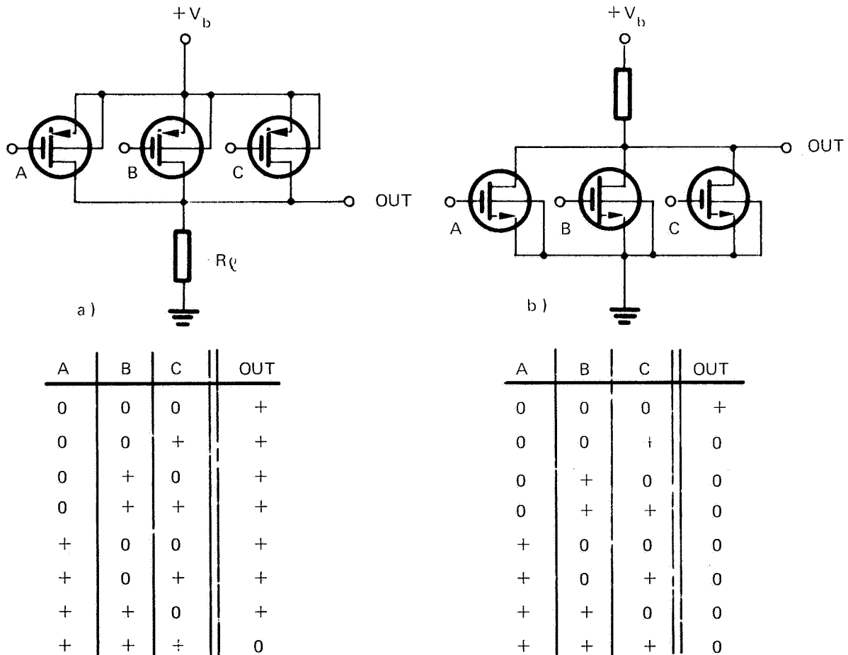
Figure 6.- Parallel connection and truth tables for, a : P-channel ; b : N-channel MOSFETs.
