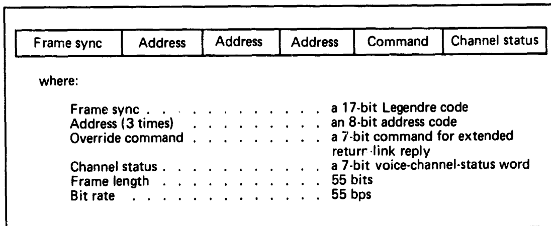
(a) Forward link
