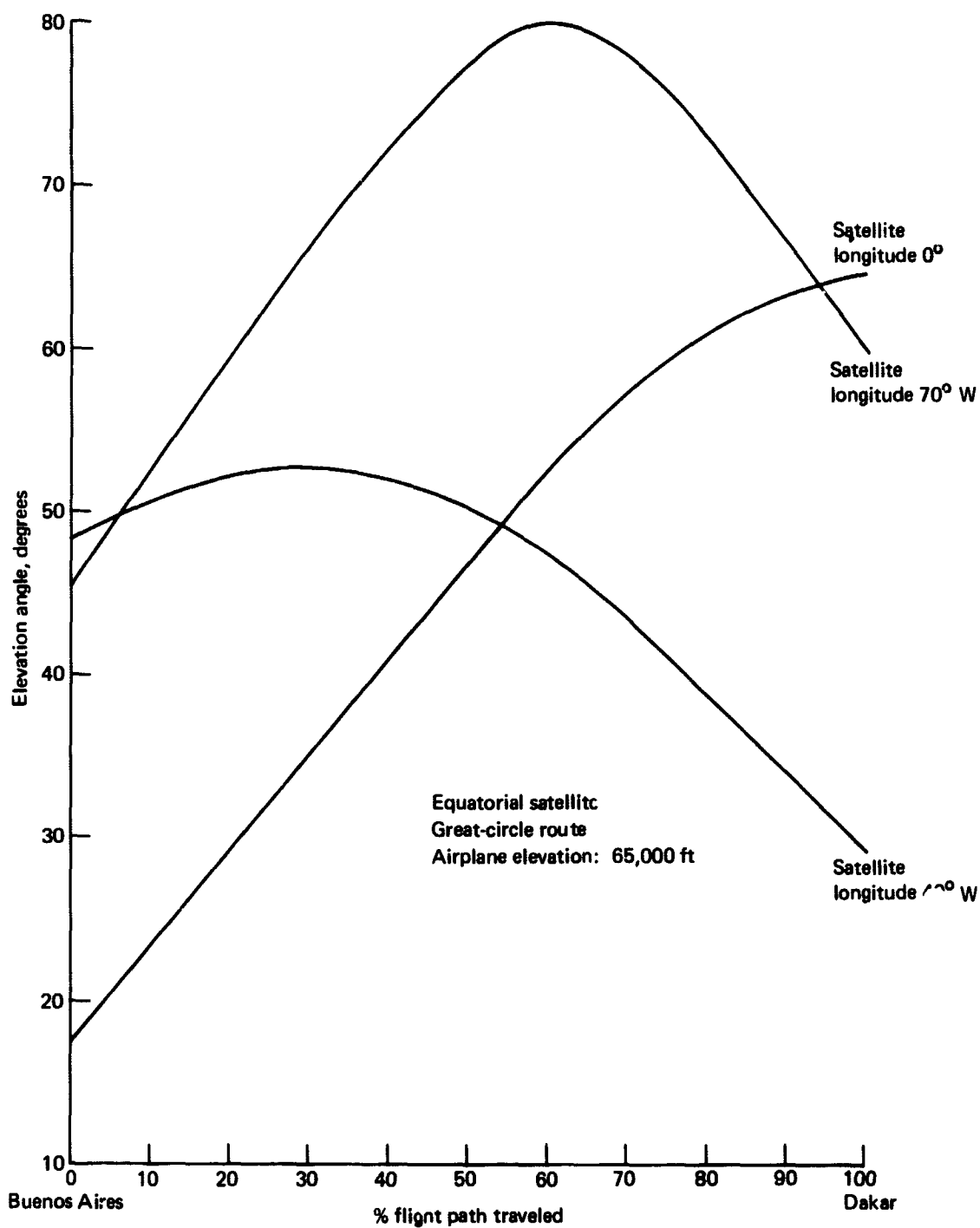
FIGURE 5.— ELEVATION ANGLE TO SATELLITE: BUENOS AIRES-DAKAR
