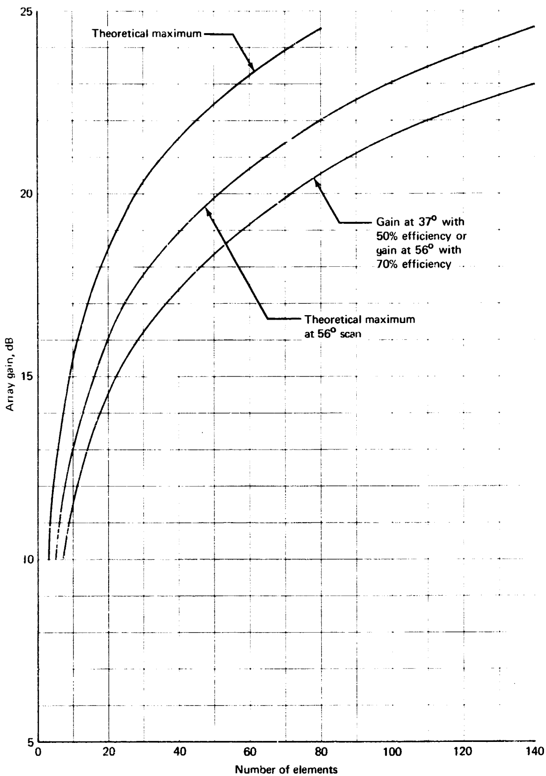
FIGURE 24.— ARRAY GAIN
