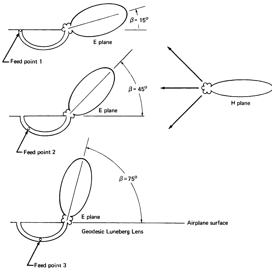
FIGURE 19.— GEODESIC-LENS BEAM POSITIONING BY FEED SWITCHING
