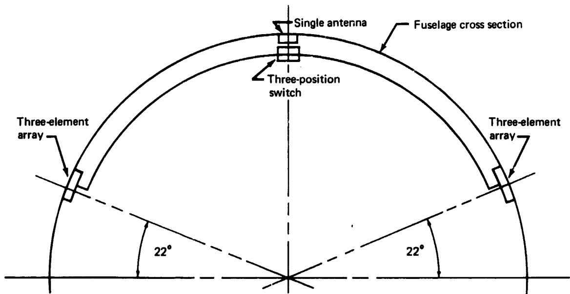
FIGURE 40.— SWITCHED THREE-ANTENNA OPERATIONAL CONFIGURATION
