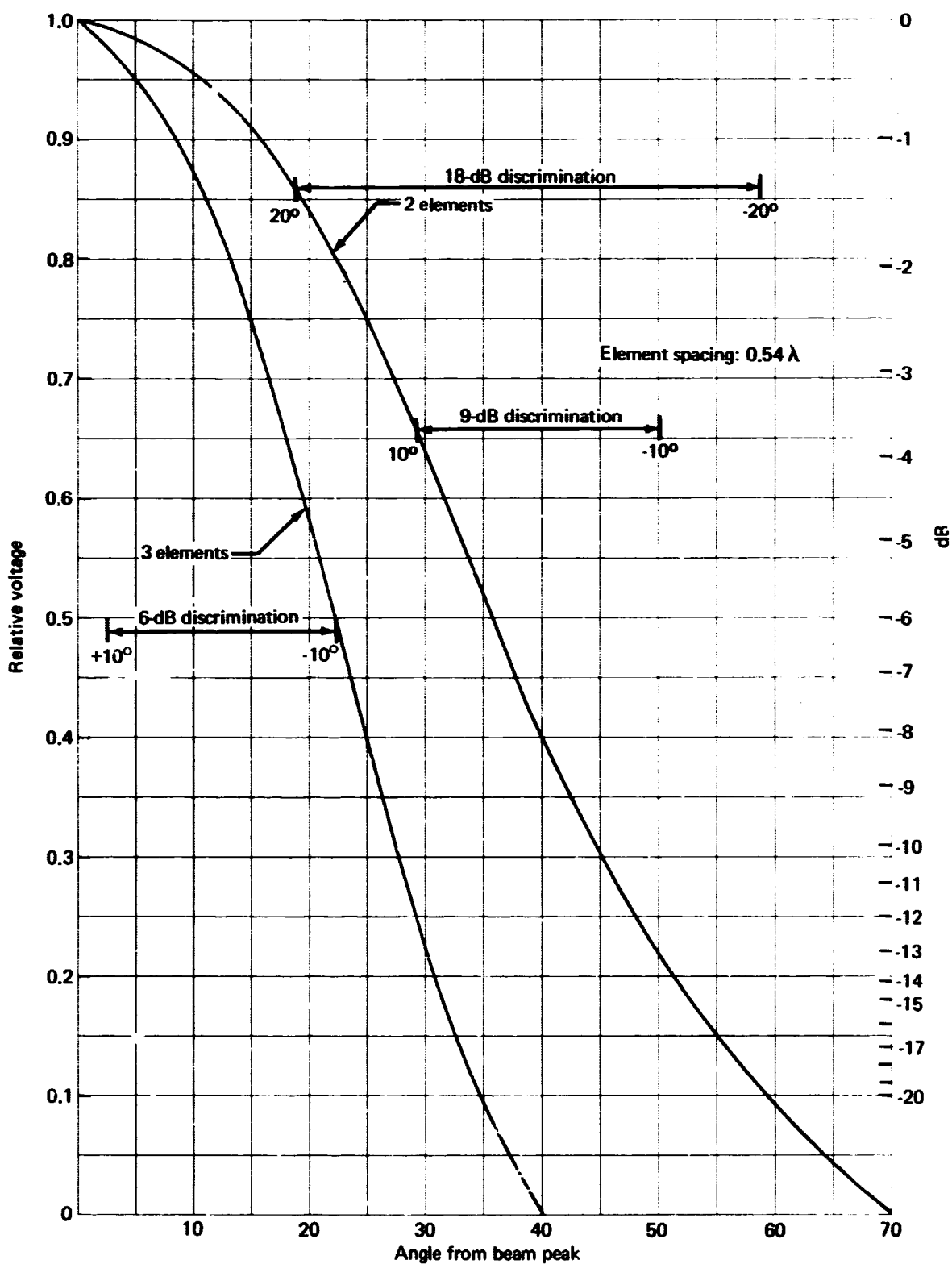
FIGURE 35.— ELEVATION PATTERNS OF TWO- AND THREE-ELEMENT ARRAYS
