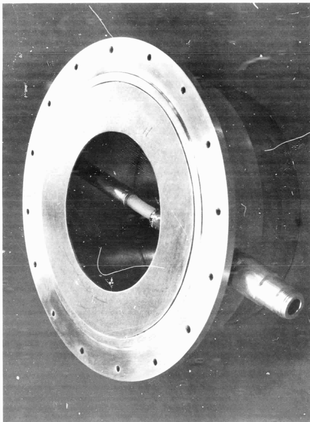
FIGURE 12.— ORTHOGONAL-MODE-CAVITY ANTENNA
