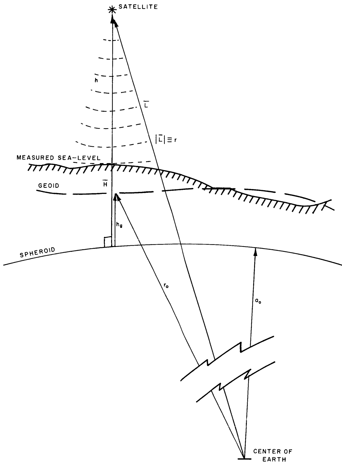
Figure 2-7 Geometric Relationships for Error Analysis
