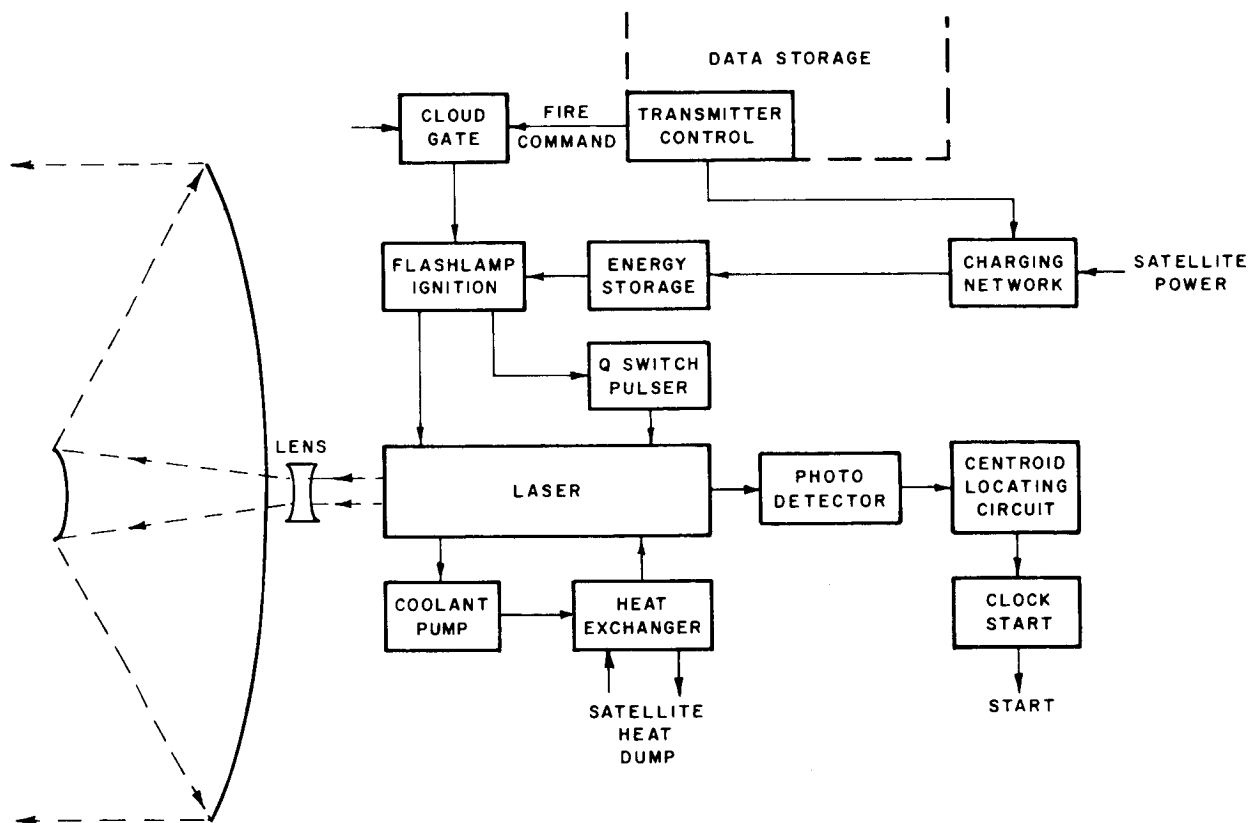
Figure 3-2 Transmitter Block Diagram
