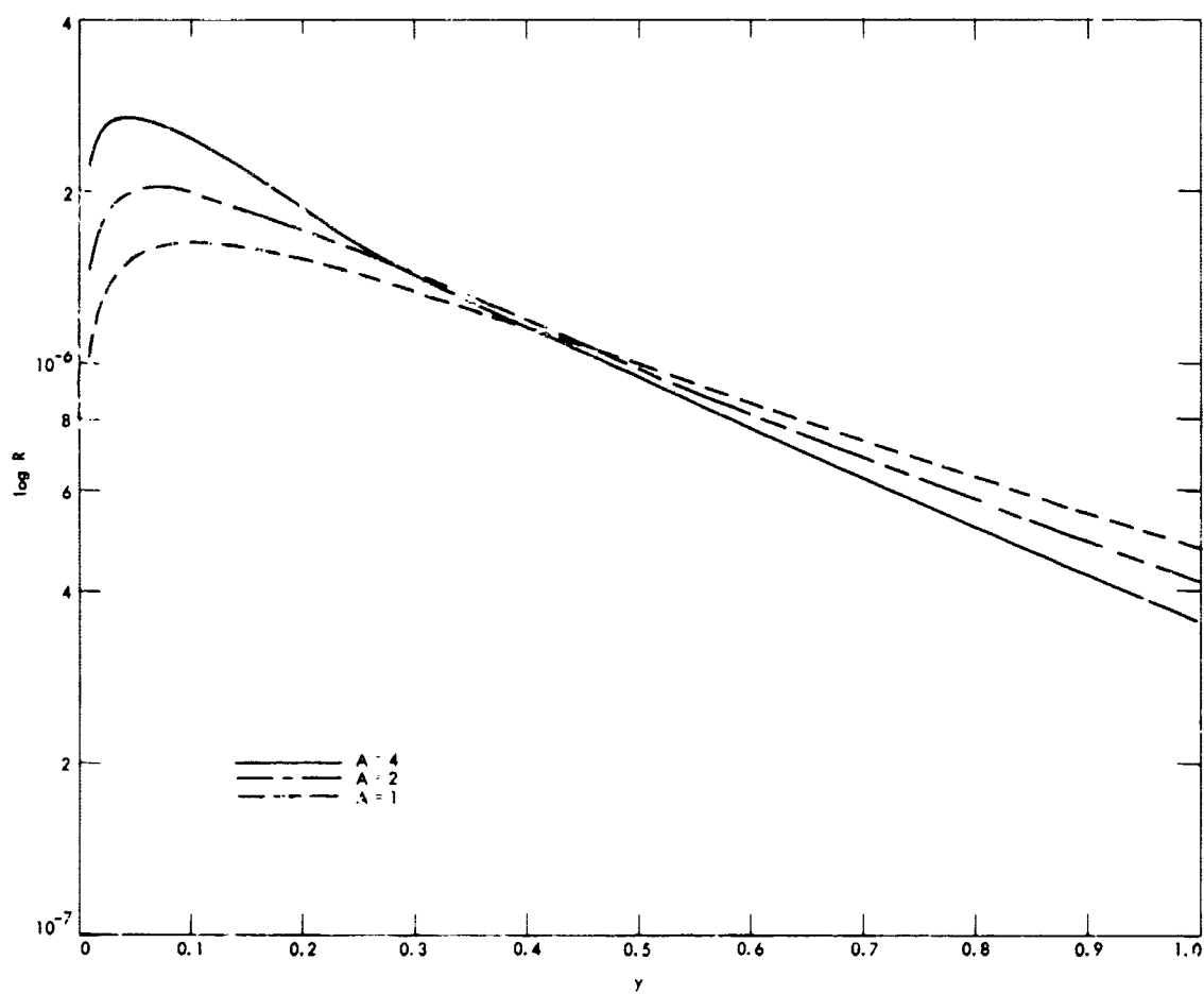
Fig. 2. Calculated excitation rate dependence on parameter \gamma = U_{p,q}/kT , high-temperature behavior ( A = 1, 2, 4 )
