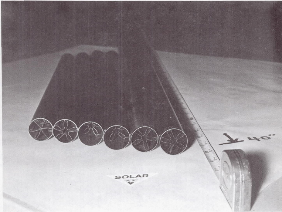
FIGURE 38. END VIEWS OF FOUR 18-INCH AND TWO 36-INCH HEAT RECEIVER TUBES; Post-Brazing
