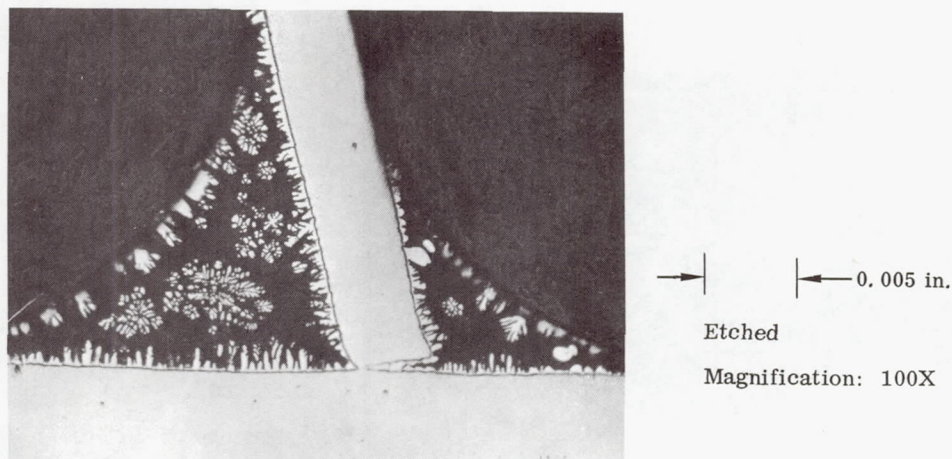
FIGURE 10. Cb-1Zr T-JOINT BRAZED WITH Ti-46.5Zr-4V-3Be; As-Brazed Condition
