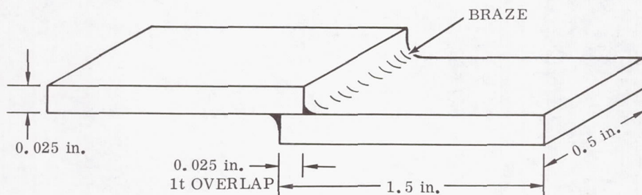
FIGURE 5. BRAZED SINGLE-LAP SHEAR SPECIMEN
