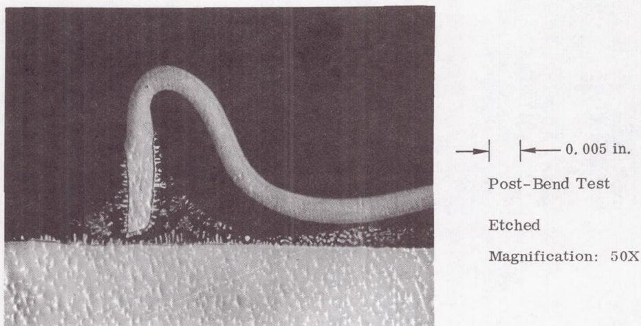
FIGURE 9. Cb-1Zr T-JOINT BRAZED WITH Ti-48Zr-4Be; As-Brazed Condition
