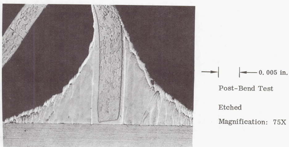
FIGURE 8. Cb-1Zr T-JOINT BRAZED WITH PURE GOLD FOIL; As-Brazed Condition
