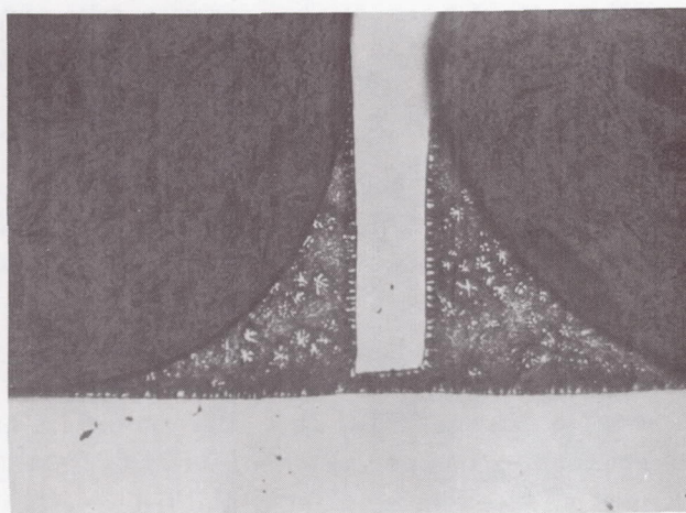
FIGURE 12. Cb-1Zr T-JOINT BRAZED WITH Zr-19Cb-6V-3Be; As-Brazed Condition
