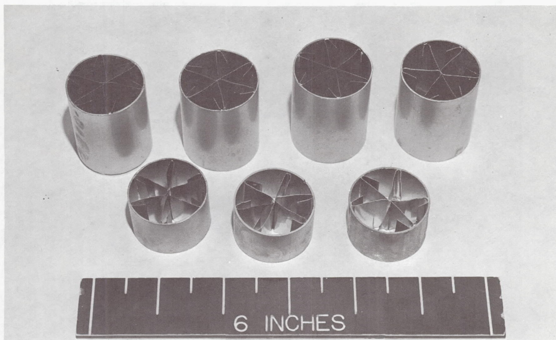
FIGURE 39. TYPICAL HEAT RECEIVER TUBE SECTIONS; Brazed and Prepared for Long-Term Aging
