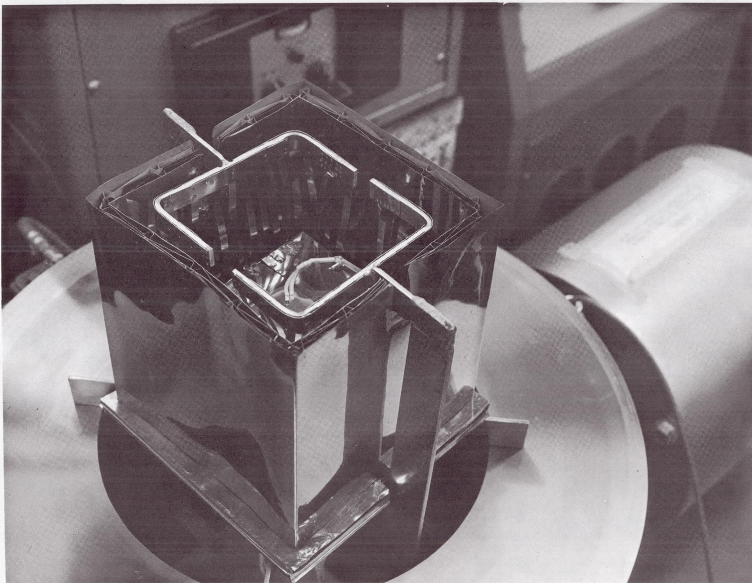
FIGURE 20. VACUUM AGING FURNACE HOT ZONE; Internal View Showing Specimen Pack
