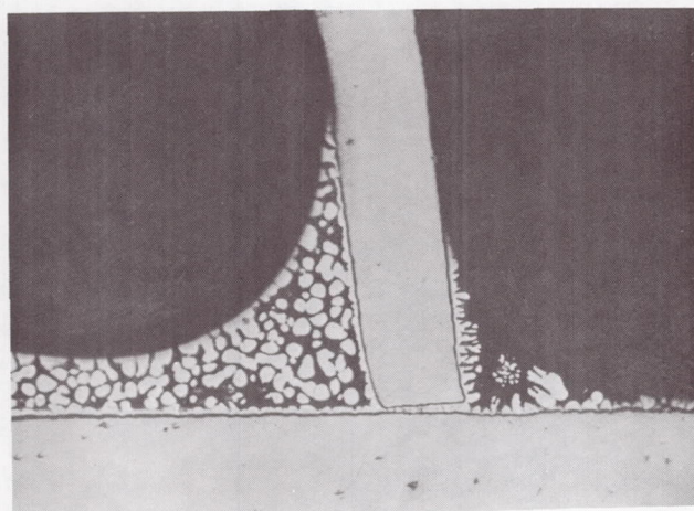
FIGURE 11. Cb-1Zr T-JOINT BRAZED WITH Ti-45Zr-7Cb-3Be; As-Brazed Condition
