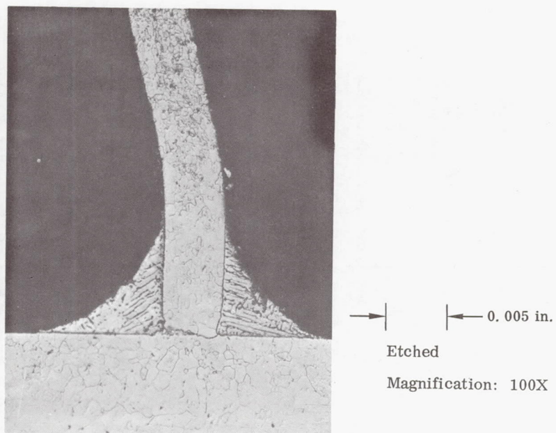
FIGURE 7. Cb-1Zr T-JOINT BRAZED WITH Cu-2Ni; As-Brazed Condition
