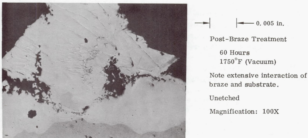
FIGURE 15. Cb-1Zr T-JOINT BRAZED WITH GOLD
