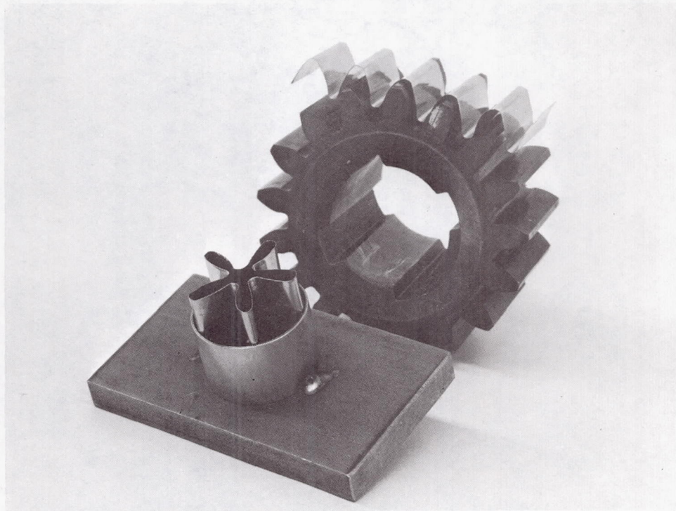
FIGURE 35. CORRUGATING GEAR AND SIZING FIXTURE FOR FABRICATING DESIGN B FIN MODULES
