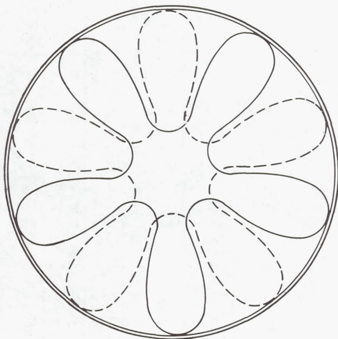
FIGURE 34. SCHEMATIC OF SECOND FIN REDESIGN; Design B
