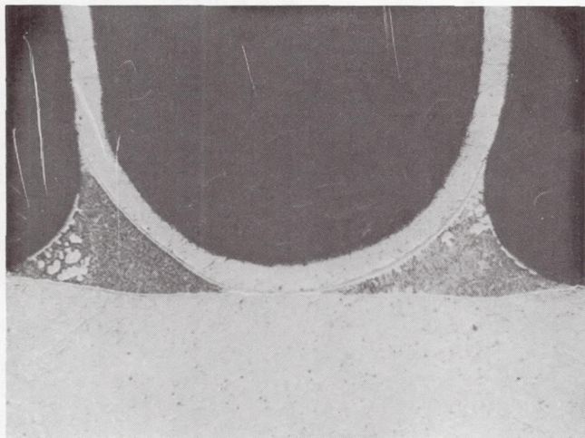
As-Brazed Condition
