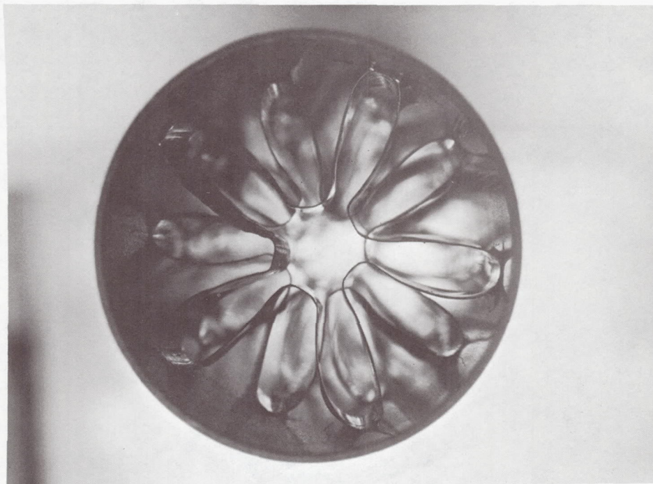
FIGURE 36. INTERNAL VIEW OF 18-INCH HEAT RECEIVER TUBE (1.25 in. Major Dia. ); Design B Fin Modules Brazed in Position
