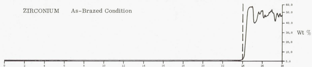
ZIRCONIUM Vacuum Aged (1000 hr at 1750°F)
