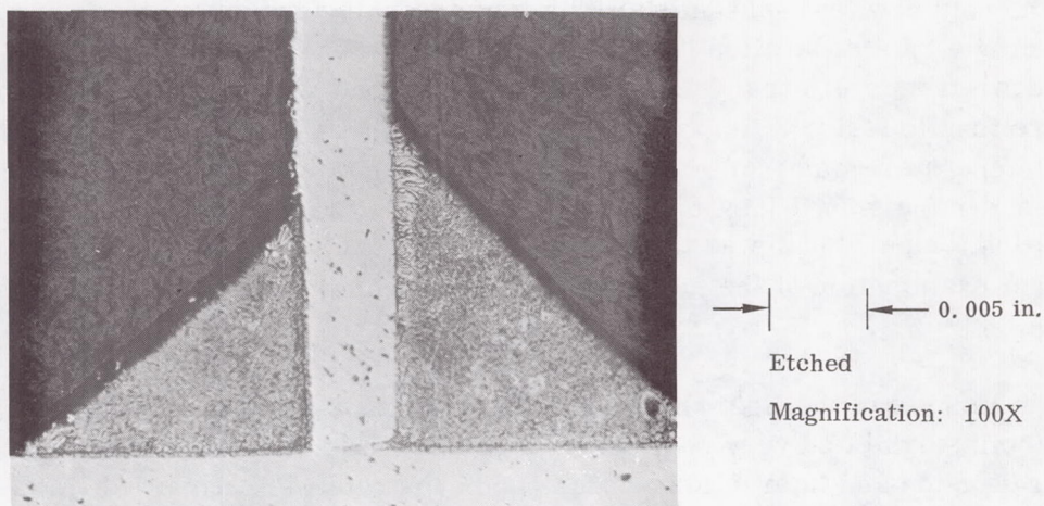
FIGURE 14. Cb-1Zr T-JOINT BRAZED WITH Zr-28V-16Ti-0.1Be; As-Brazed Condition
