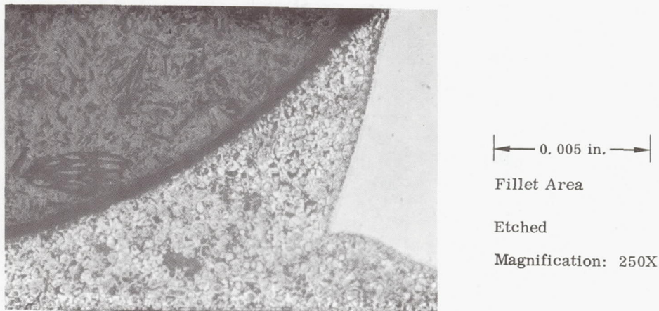
FIGURE 13. Cb-1Zr T-JOINT BRAZED WITH Zr-28V-16Ti; As-Brazed Condition
