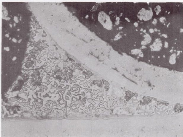
FIGURE 42. TRANSVERSE SECTIONS THROUGH TUBE/FIN BRAZEMENTS MADE WITH Zr-28V-16Ti BRAZE ALLOY; Fin Design A
