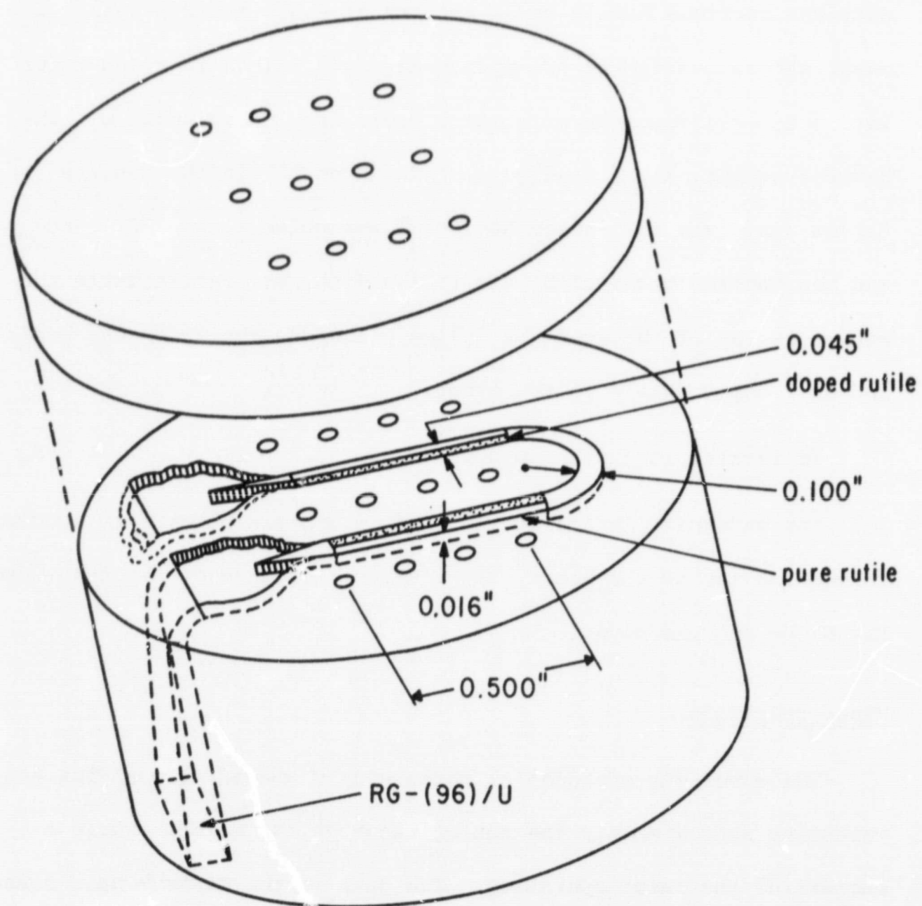
Figure 14 - 36 GHz Maser
