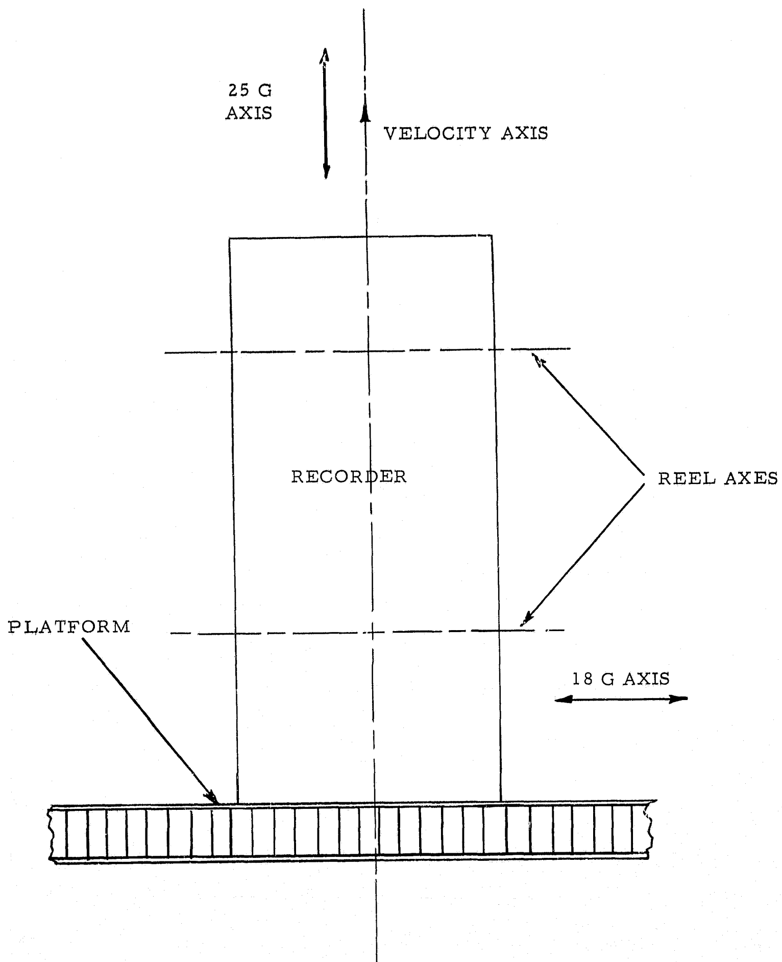
FIGURE 21 . TAPE RECORDER MOUNT DETAIL
