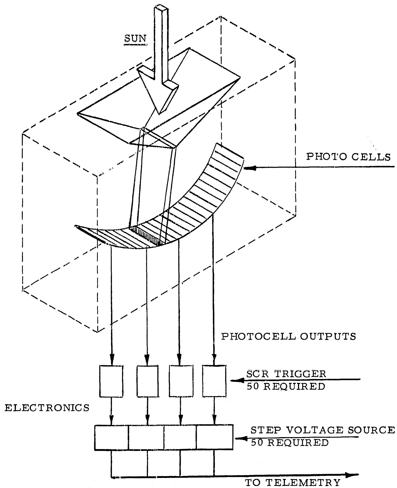
FIGURE 12 . ANGULAR DETERMINATION SUN SENSOR
