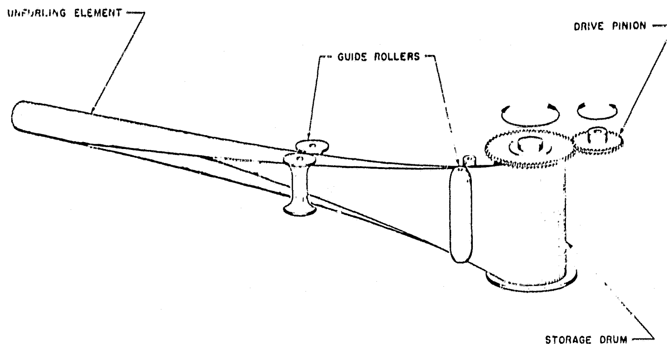
FIGURE 9. THE STEM PRINCIPLE
