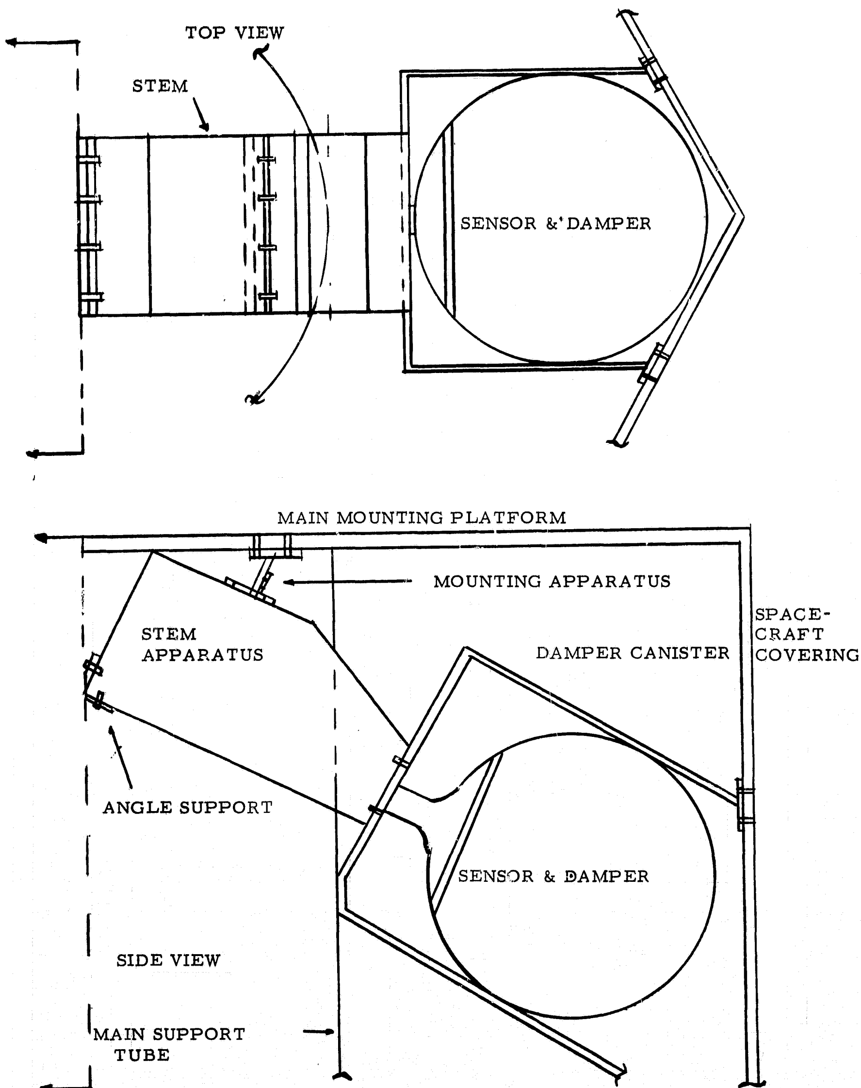
FIGURE 31 . MOUNTING OF CANISTERS
