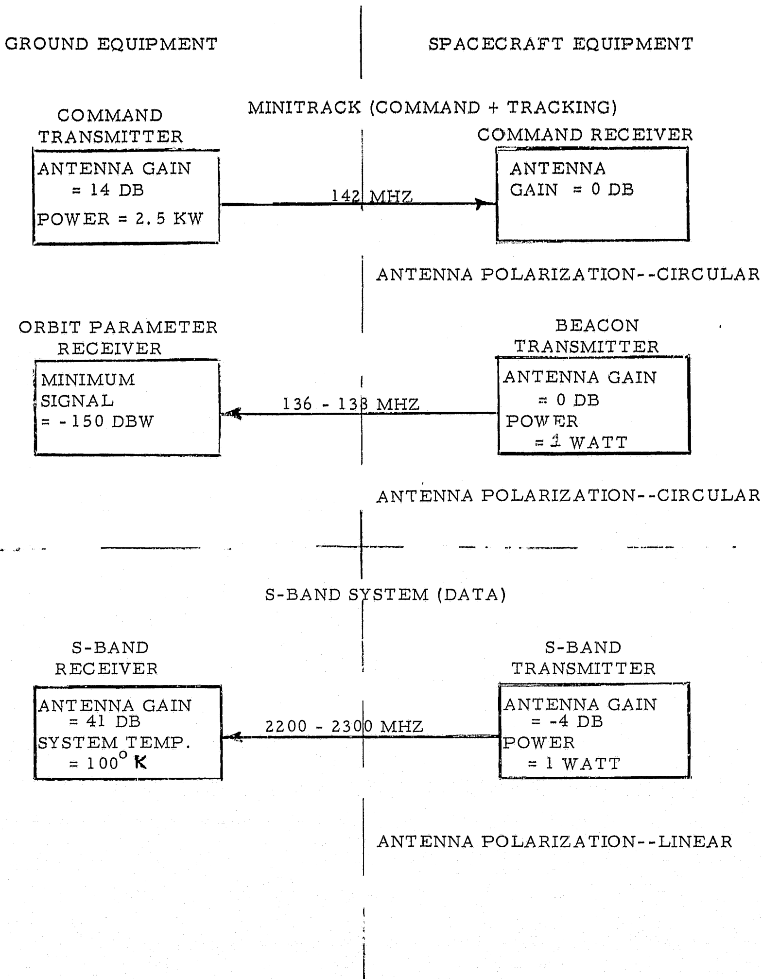
FIGURE 22. PROPOSED COMMUNICATION LINKS
