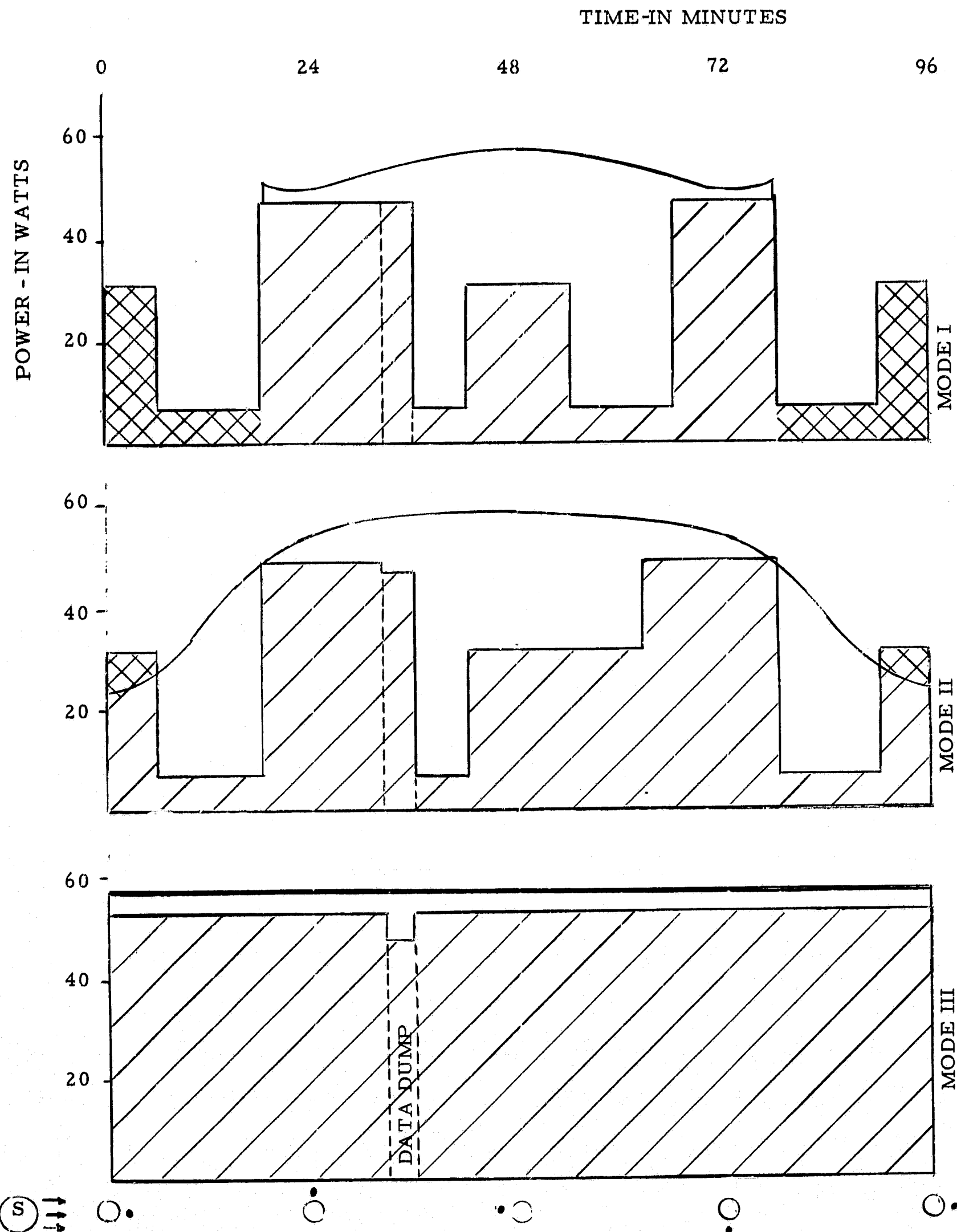
FIGURE 14 . POWER HISTOGRAM
