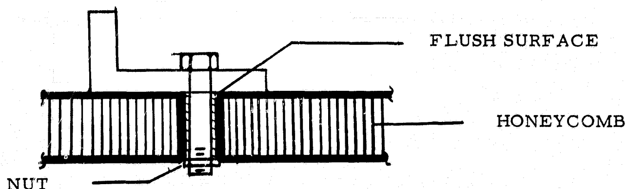
FIGURE 28. HONEYCOMB FASTENING TECHNIQUE
