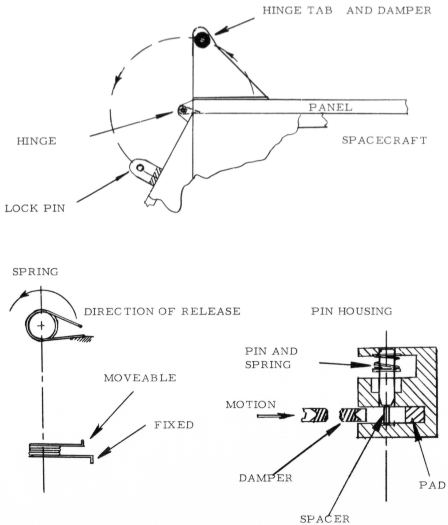
FIGURE 15 . PANEL HINGE MECHANISM
