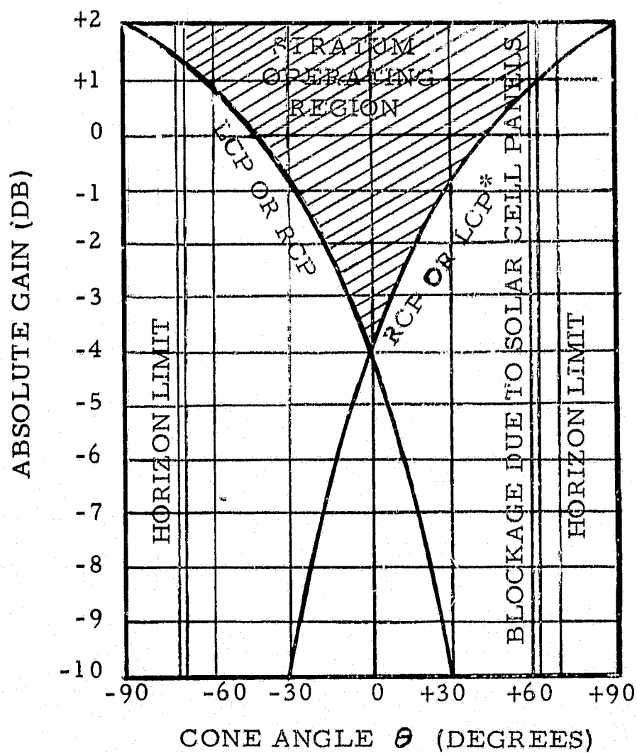
FIGURE 26 . VHF ANTENNA
