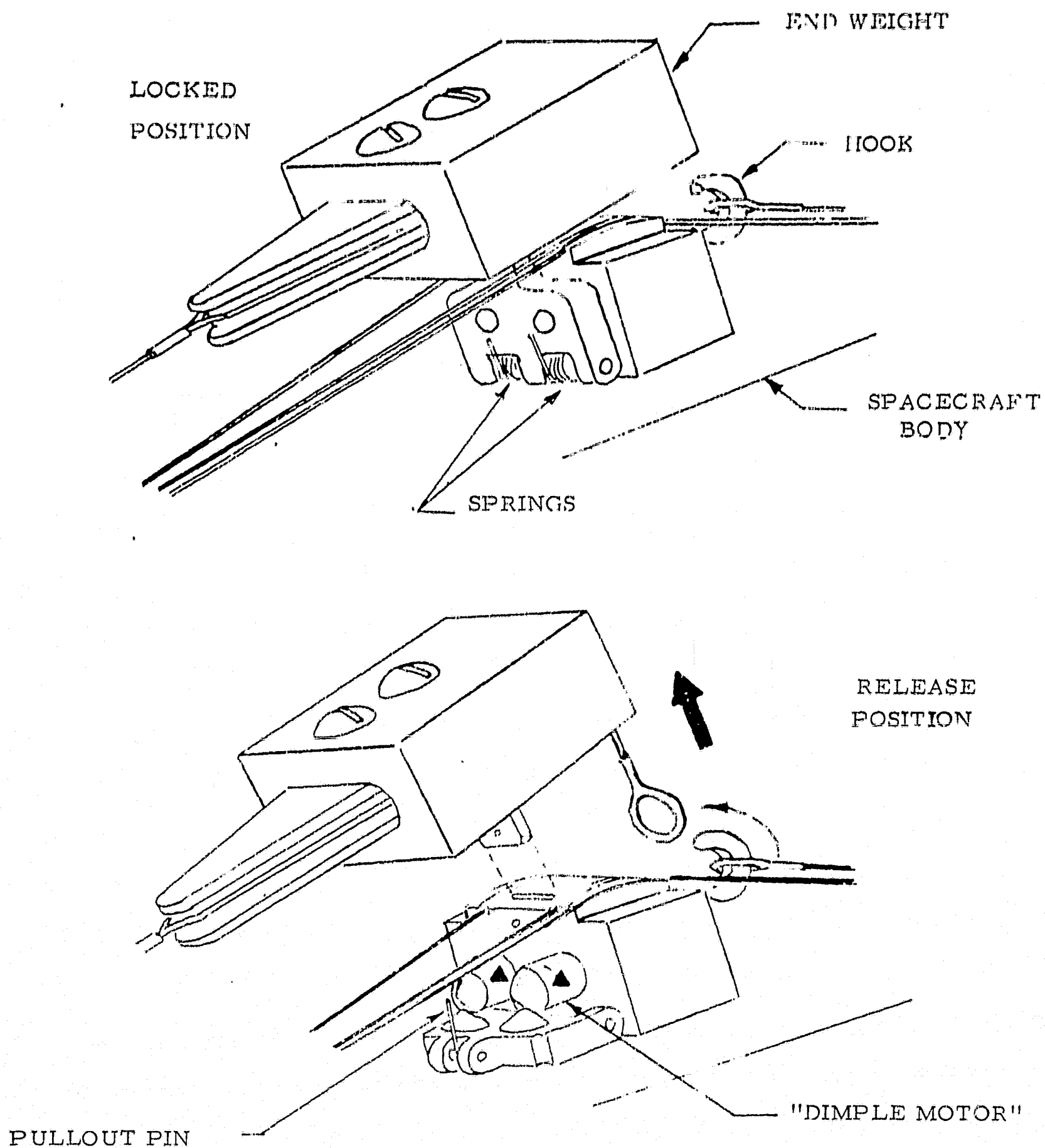
FIGURE 39. DESPIN WEIGHT RELEASE MECHANISM
