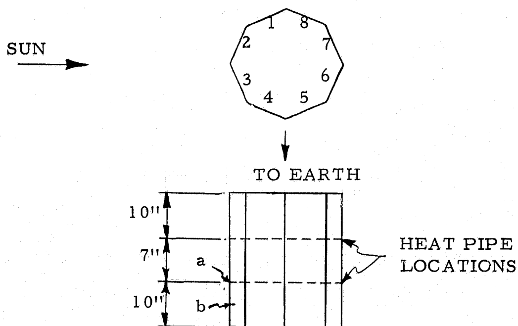
FIGURE 42 . SATELLITE MAIN BODY CONFIGURATION AND NUMBERING SYSTEM USED IN THERMAL CONTROL CALCULATIONS.
