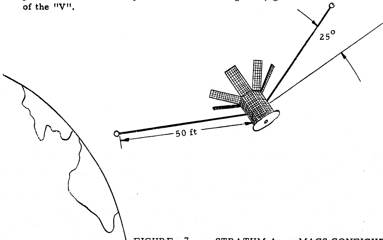
FIGURE 7 . STRATUM Aero-MAGS CONFIGURATION
