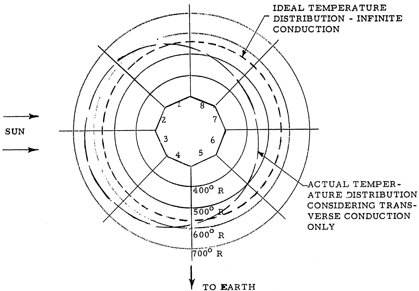
FIGURE 17. TEMPERATURE DISTRIBUTION AROUND THE SATELLITE
