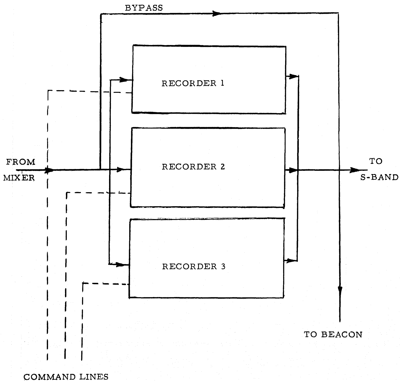
FIGURE 20 . STORAGE SYSTEM DIAGRAM
