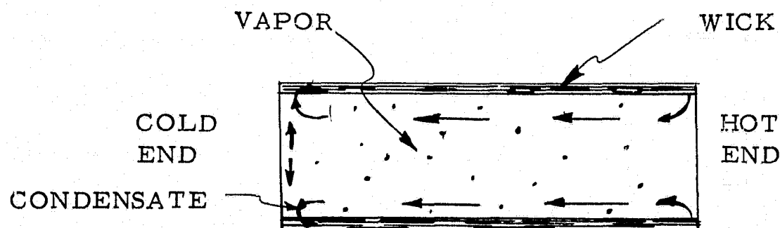
FIGURE 16. HEAT PIPE
