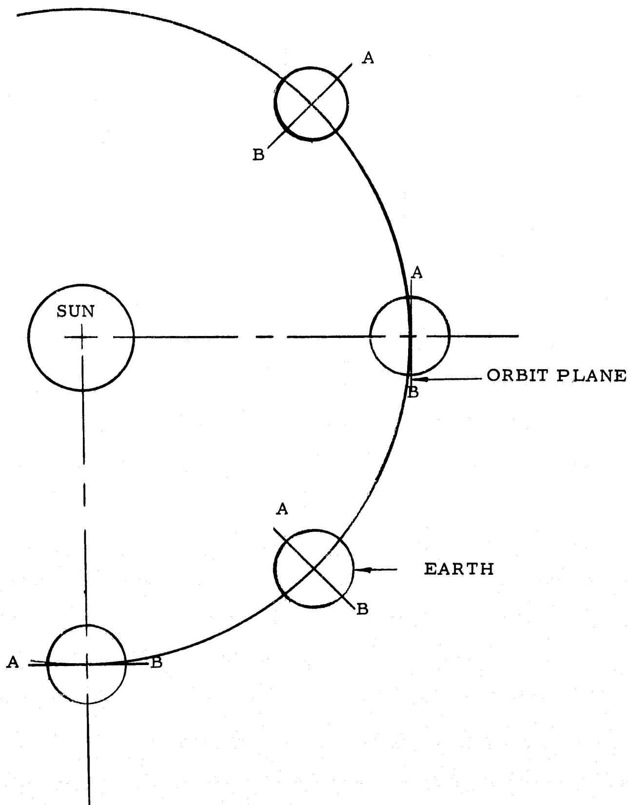
FIGURE 1 . ORBIT PRECESSION
