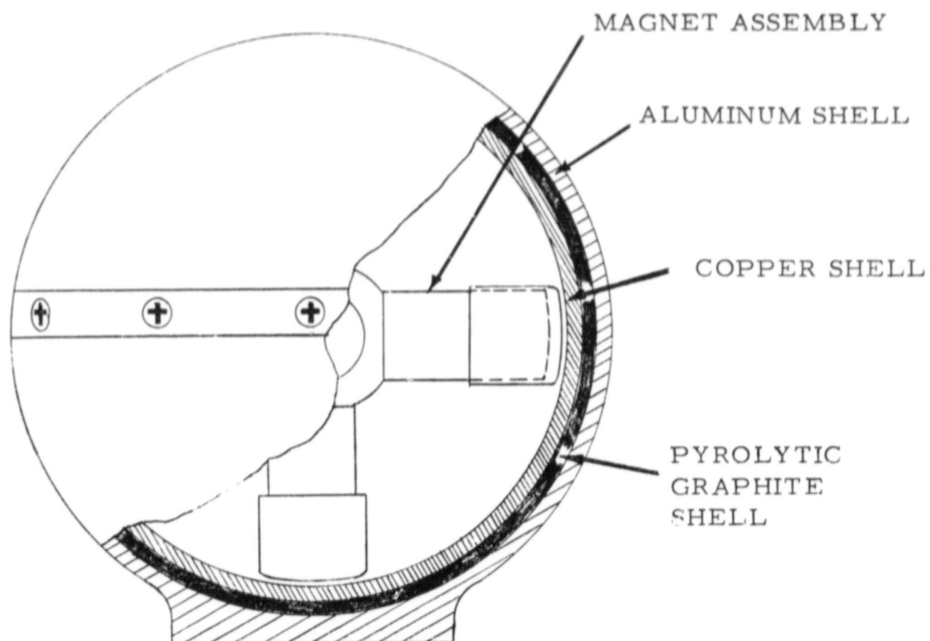
FIGURE 10 . MAGNETICALLY ANCHORED EDDY CURRENT DAMPER
