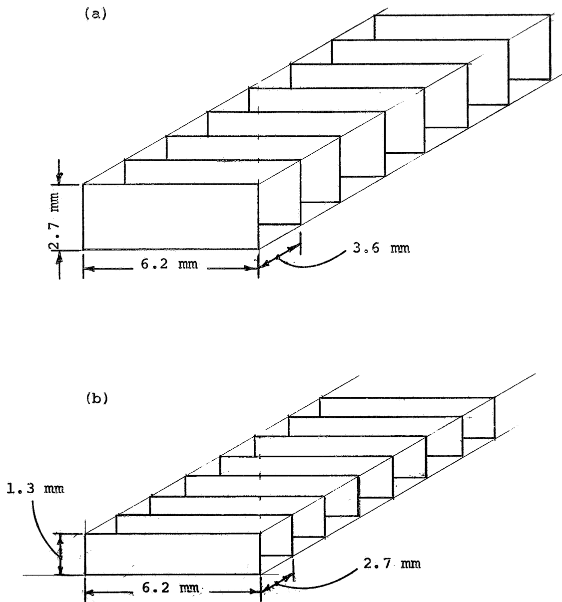
Fig. 7 Geometries of the strip structures
