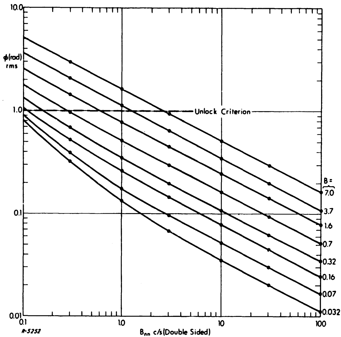
Fig. 3 Carrier Lock Error for A = 0.02 0.032 < B < 7
