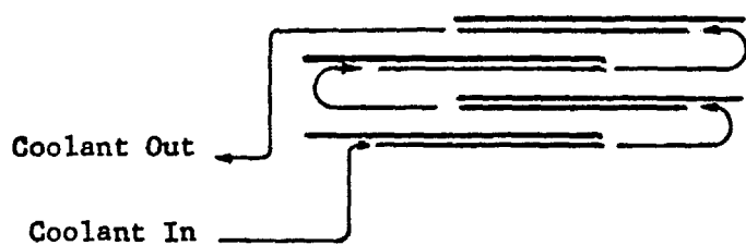
Elevation View
