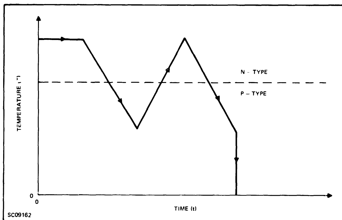
Figure 6. Growth Cycle for Fabrication on P-N-P-N Layers
