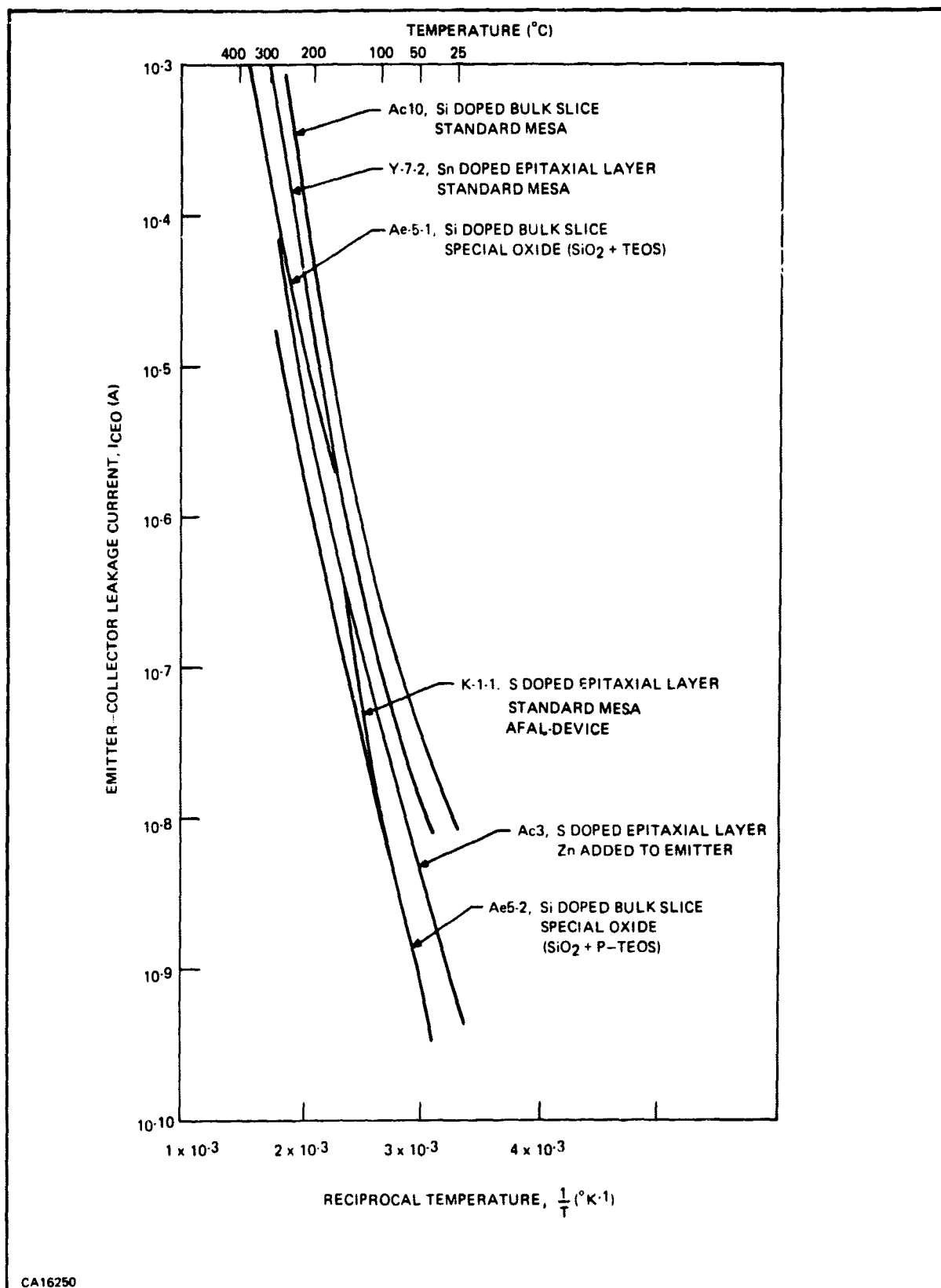
Figure 28. I_{CEO} versus Reciprocal Temperature for Various GaAs NPN Transistors Using Different Crystal Materials and Technologies. (The Collector-Junction Area is 90 \text{ mils}^2 for Device Y-7-2 and 56 \text{ mils}^2 for all Other Devices)
