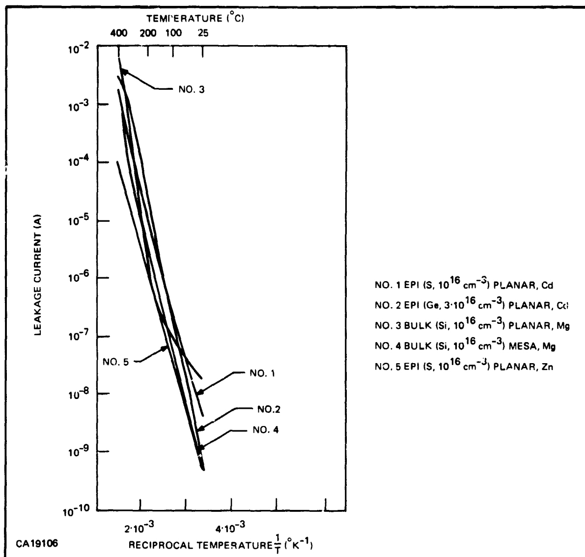
Figure 20. Reverse Leakage Current of Various Diodes versus Reciprocal Temperature (Junction Area 78 \text{ mils}^2 )
