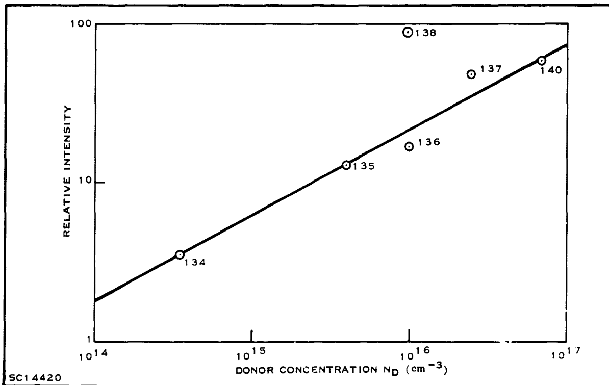
Figure 15. Cathodoluminescence Intensity versus Donor Concentration
