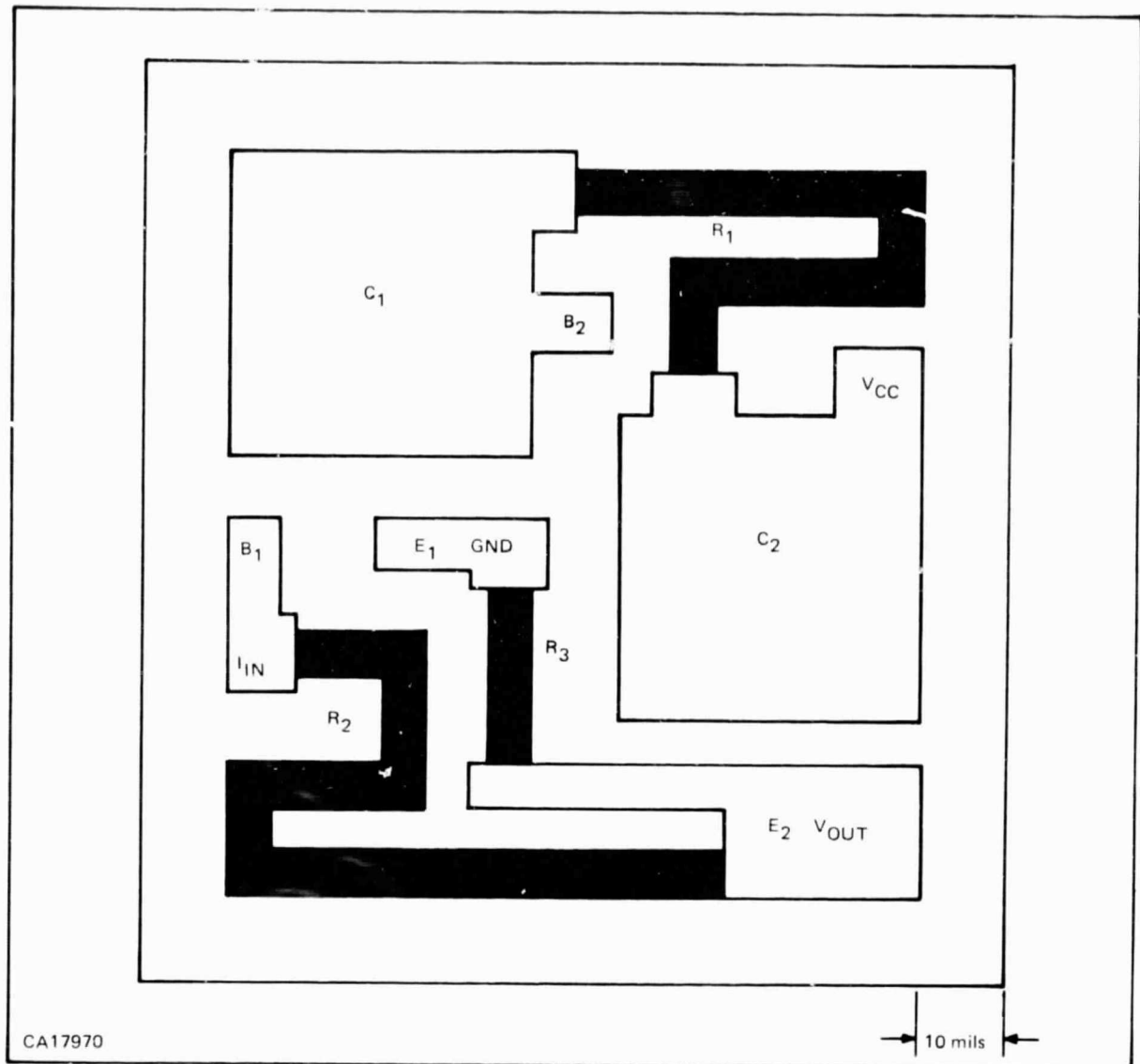
Figure 48. Thin-Film Layout for Feedback-Pair Amplifier
