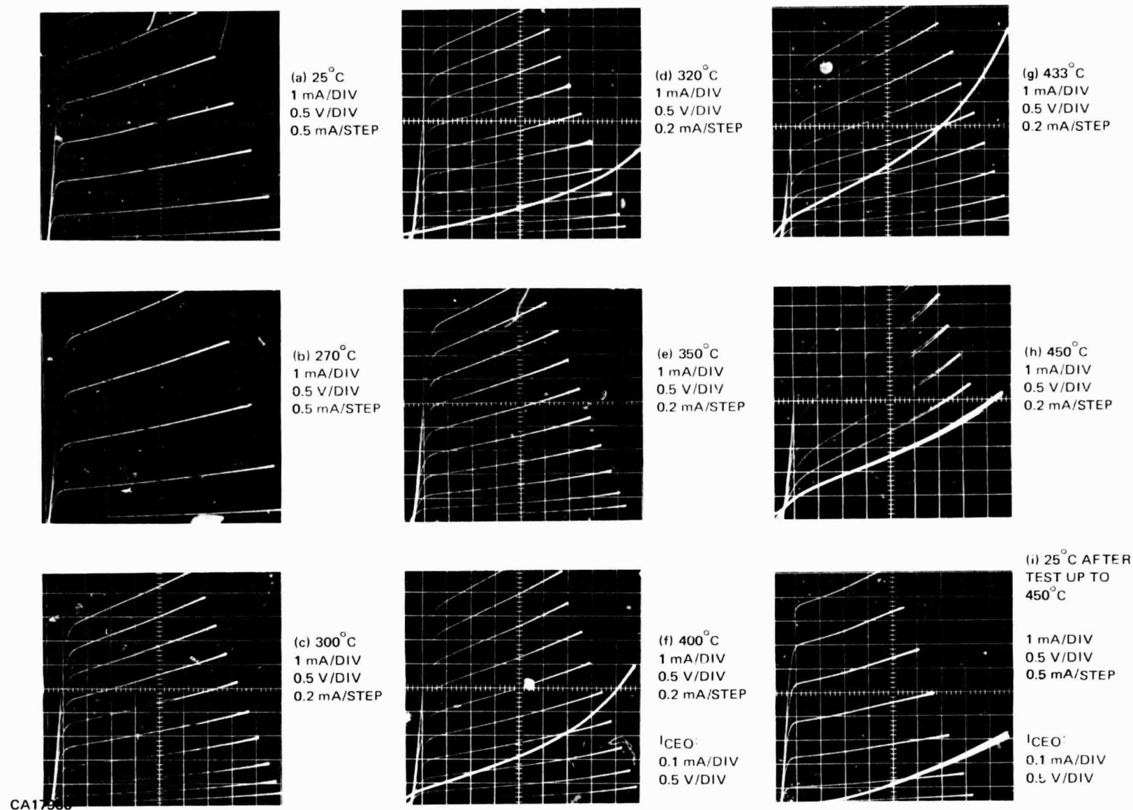
Figure 31. Performance of a PNP GaAs Transistor at Different Temperatures
