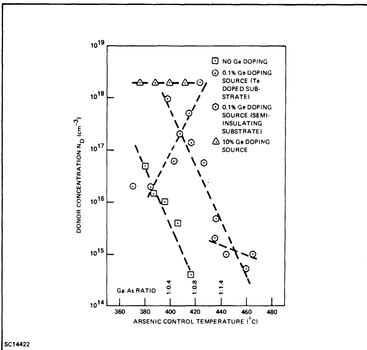
Figure 4. Donor Concentration versus Arsenic Control Temperature
