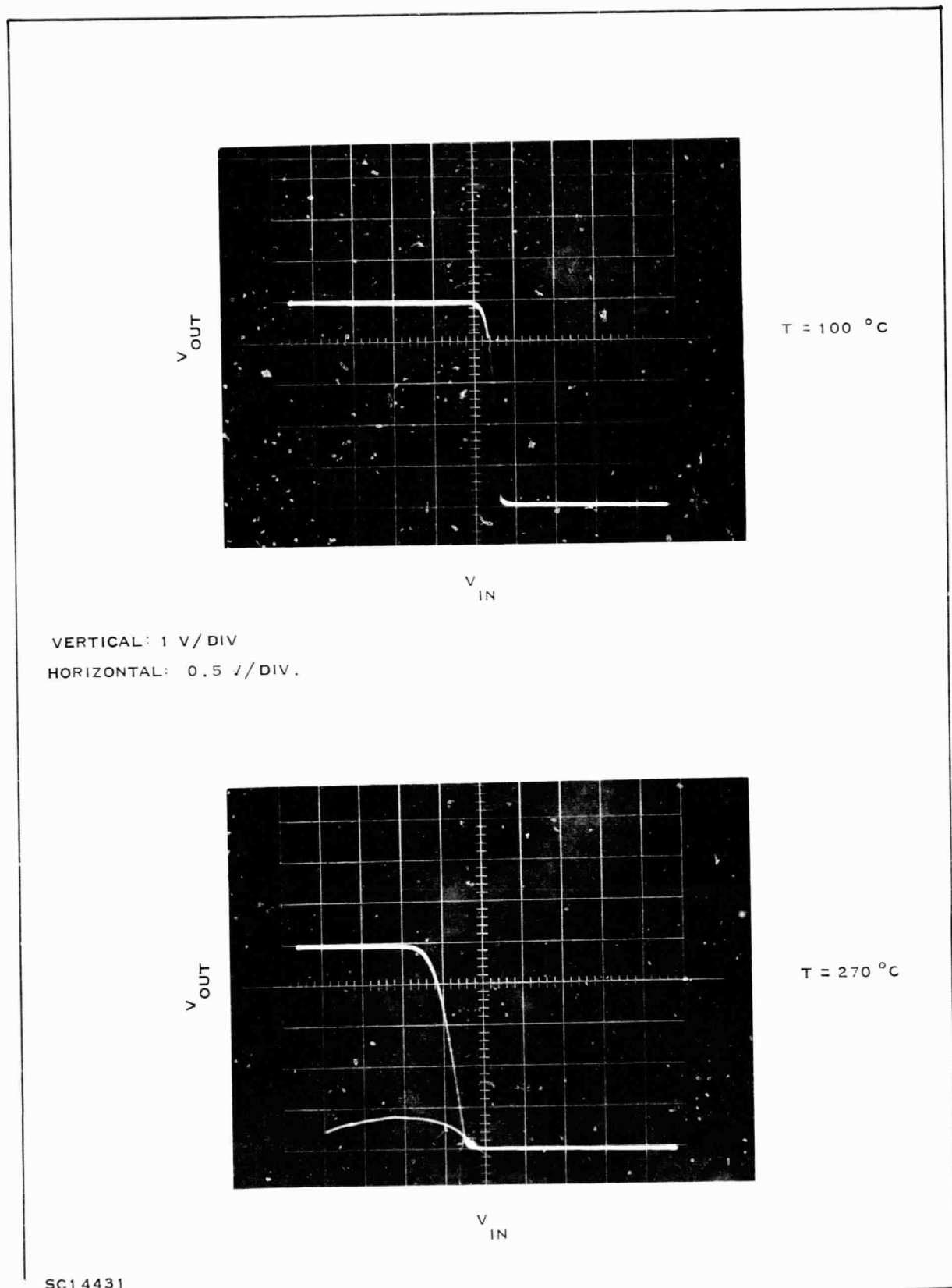
Figure 44. Characteristics of Modified NAND Gate
