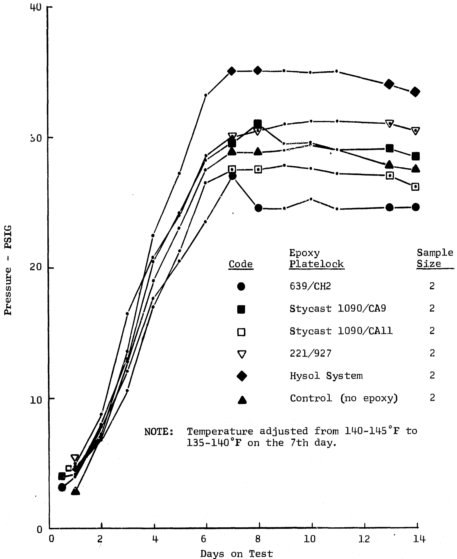
FIGURE 1 (Continued) PRESSURE GENERATED DURING 140 \pm 5^\circ\text{F} STORAGE OF MODEL 257 MONOBLOCKS WITH DIFFERENT EPOXY PLATELOCKS
