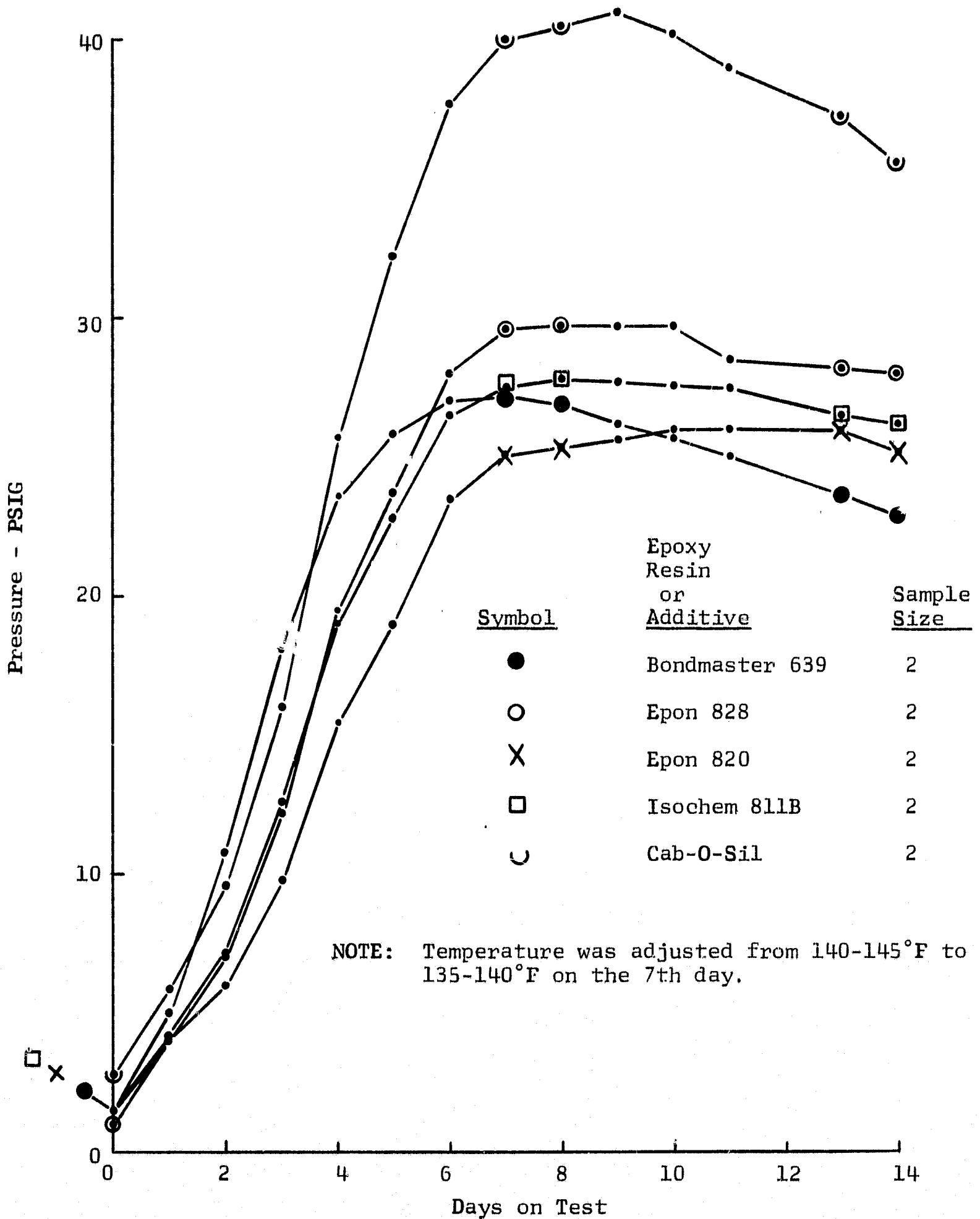
FIGURE 3 PRESSURE GENERATED DURING 140 \pm 5°F STORAGE OF MODFL 257 MONOBLOCKS CONTAMINATED WITH EPOXY RESINS OR ADDITIVES
