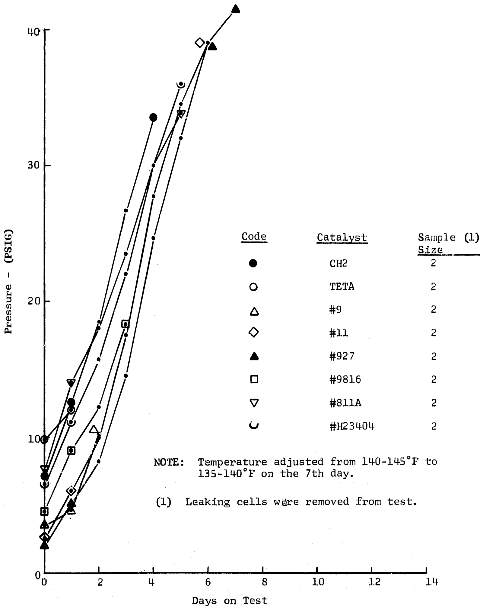
FIGURE 2 PRESSURE GENERATED DURING 140 \pm 5°F STORAGE OF MODEL 257 MONOBLOCKS CONTAMINATED WITH EPOXY CATALYSTS
