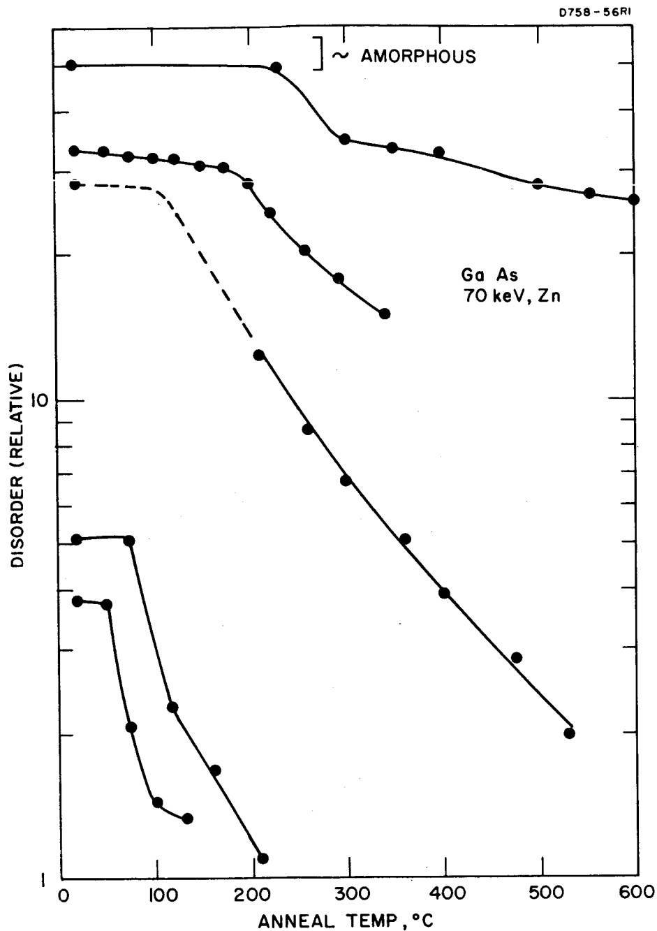
Fig. 20. Dependence of lattice disorder on annealing for zinc implanted GaAs (curves are shown for increasing ion doses from approximately 10^{14} to above 10^{16}/\text{cm}^2 ).
