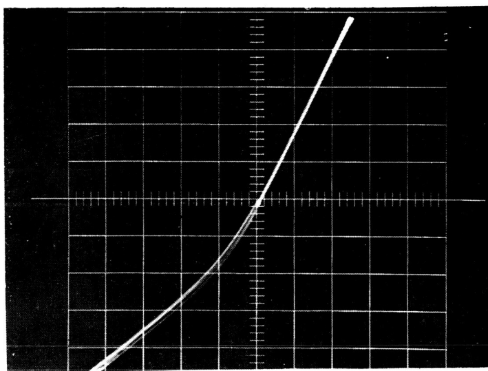
Fig. 9. I versus V measured between gold probe point contacts to an annealed sulfur implanted layer. (a) Directly touching layer (vertical = 10 \mu\text{A}/\text{div} ; horizontal = 10 \text{ V}/\text{div} ). (b) Touching layer through room temperature implanted "pads" (vertical = 10 \mu\text{A}/\text{div} ; horizontal = 0.2 \text{ V}/\text{div} ).
