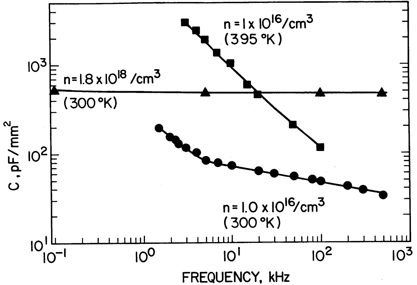
Fig. 15. Frequency dependence of zinc implanted diode junction capacitance.
