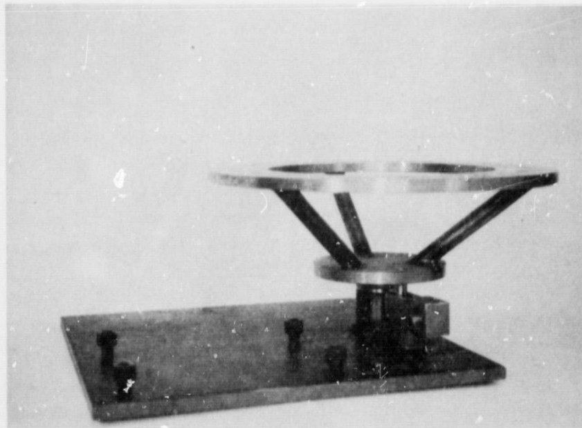
Figure 6 Vertical Twist Rig (P/N X318134)
