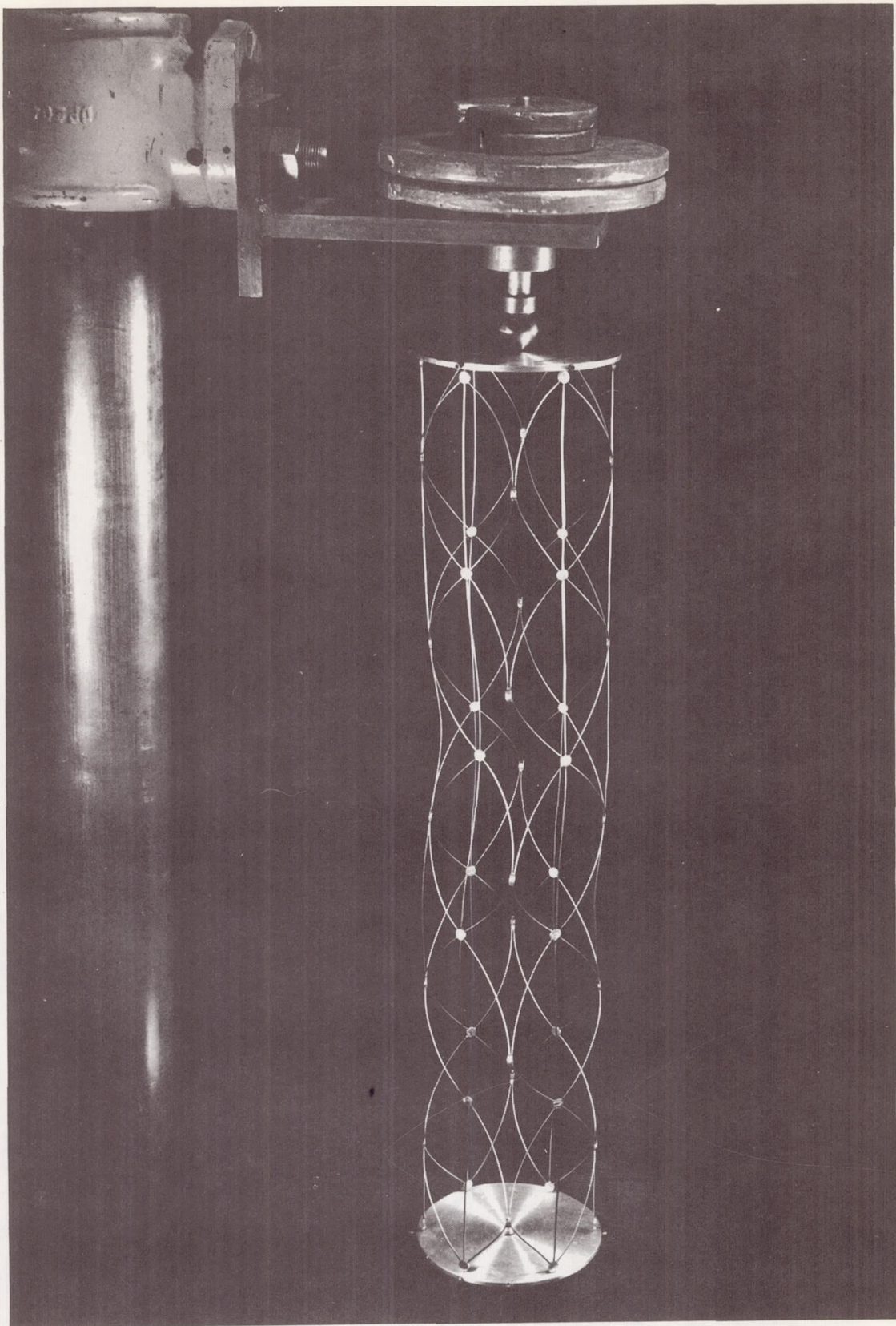
Figure 6. Test Segment as Buckled by Axial Compression
