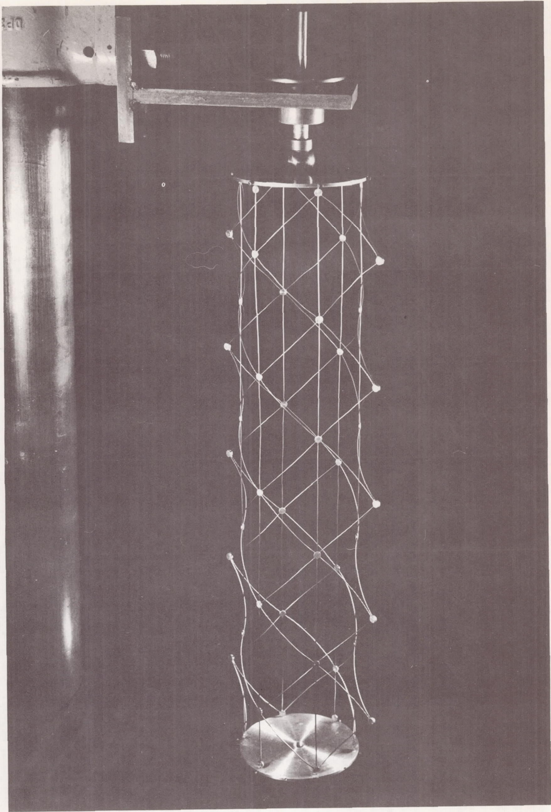
Figure 2. Test Segment of a Coilable Lattice Column
