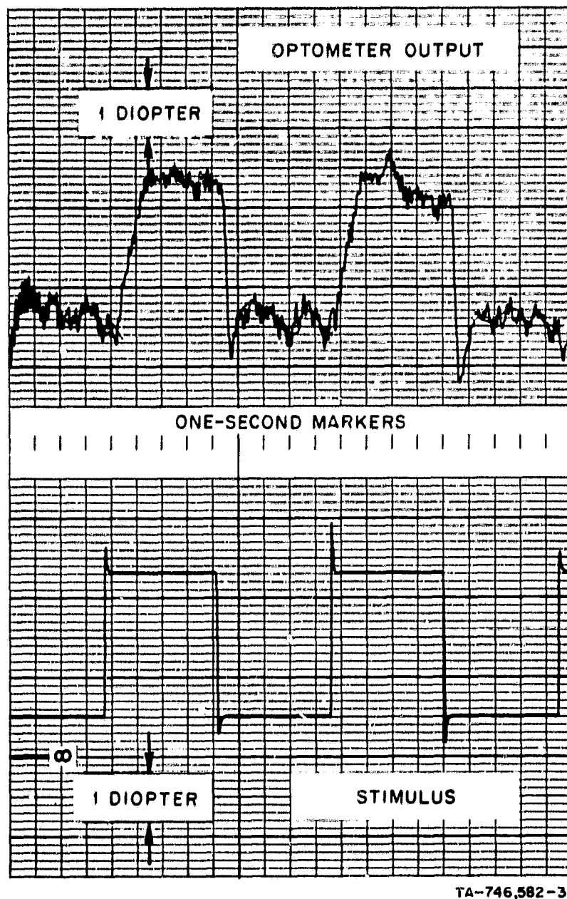
FIG. 1 A TYPICAL SET OF RESPONSES TO STEP DISPLACEMENTS OF THE TARGET
