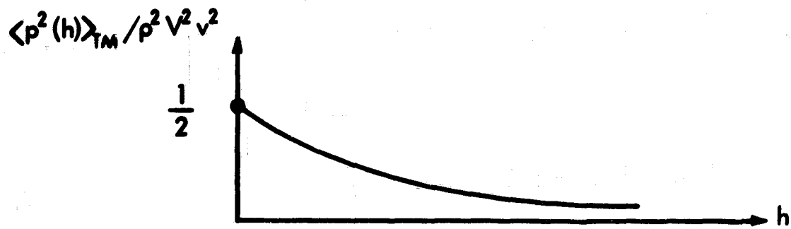
Fig. 1. Normalized mean-square pressure fluctuation due to turbulence-mean shear interaction vs. distance from shear layer (isotropic turbulence).
