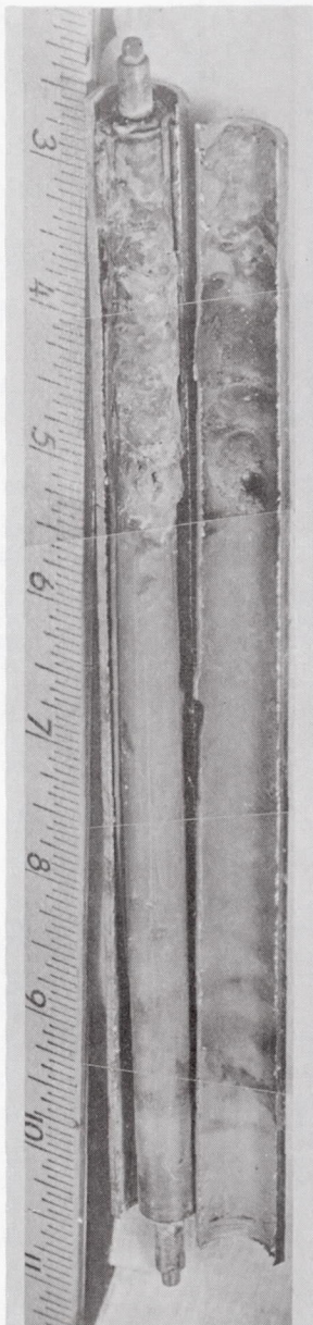
Figure 1. Failed \text{UO}_2 Fuel Pin 11A-3.
