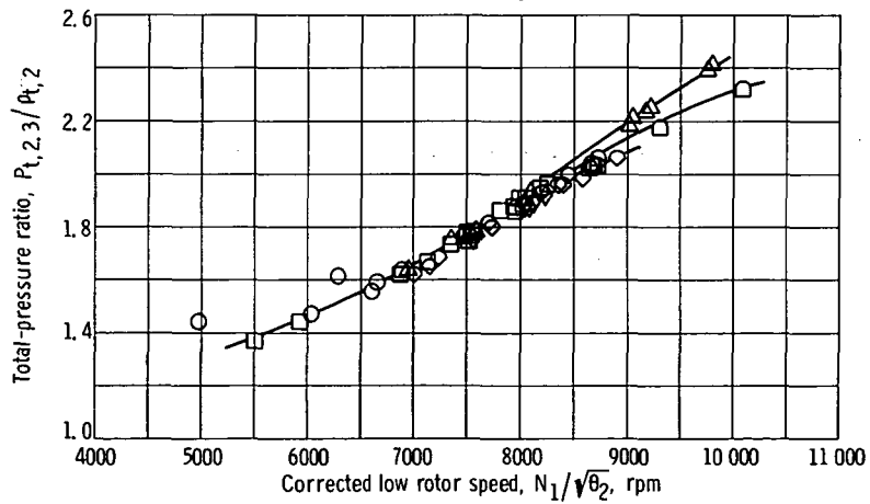
(c) Total-pressure ratio.
