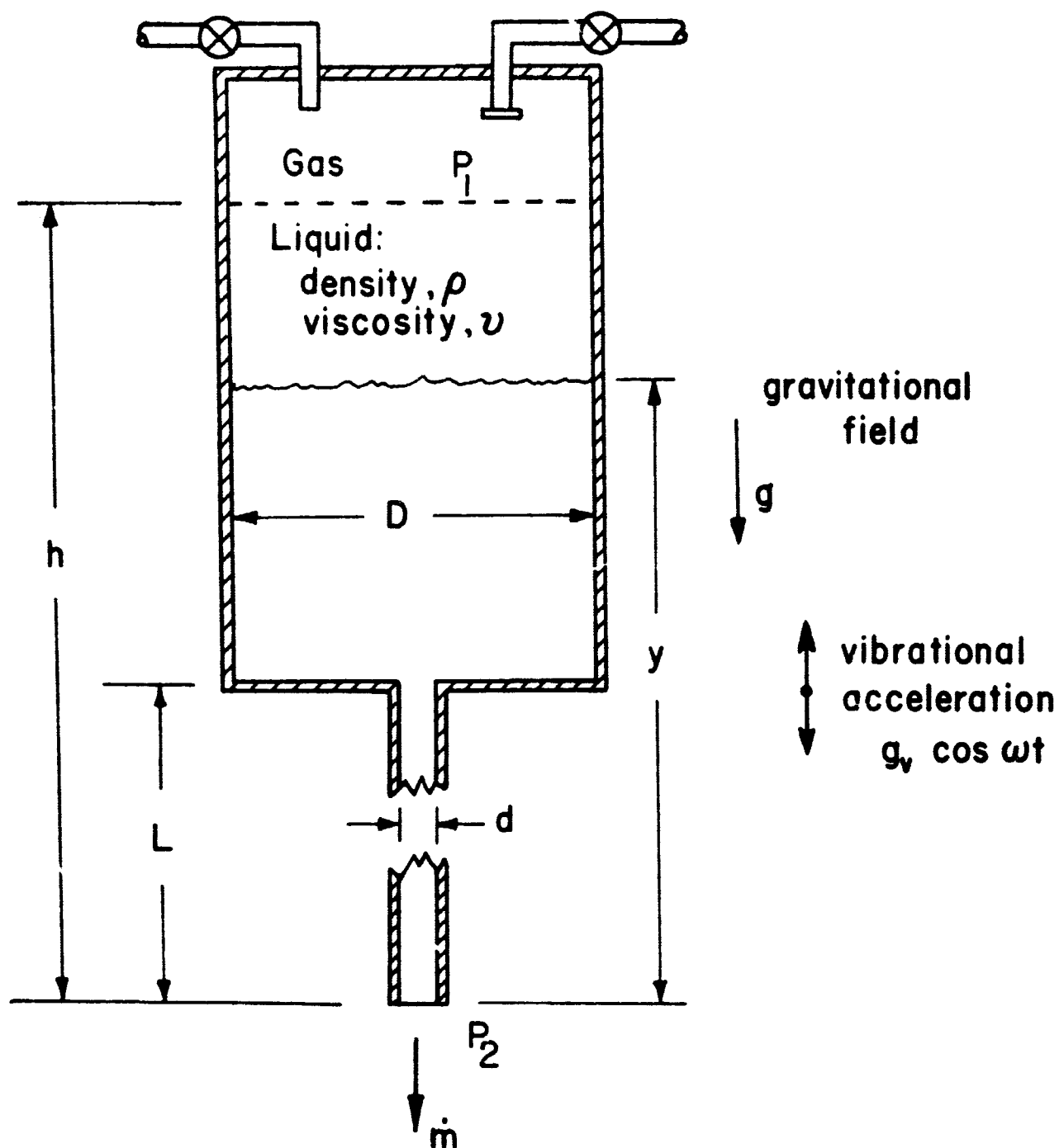
Figure 1. Discharge of Liquid From A Container Subjected to Longitudinal Vibration
