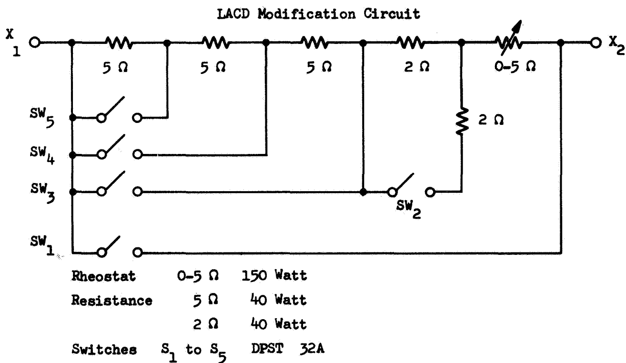
Figure 1. Schematic of LACD Modification
