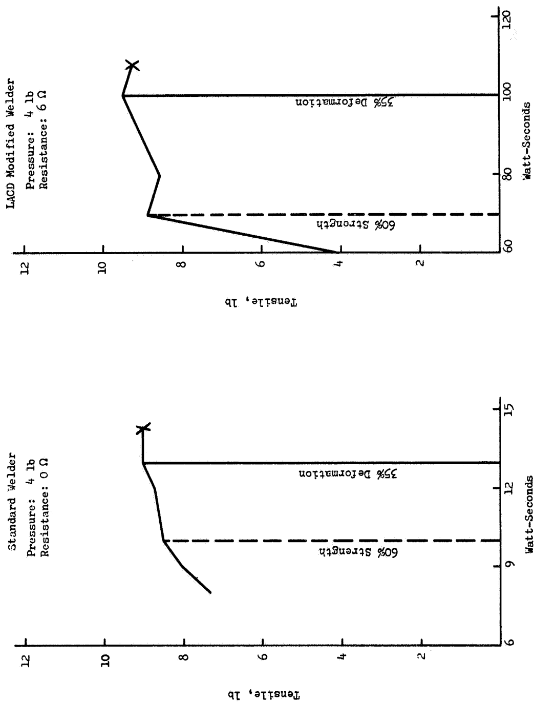
Figure 9. Isostrength Data - 0.020 OFHC Cu (Au) to 0.025 Ni200
