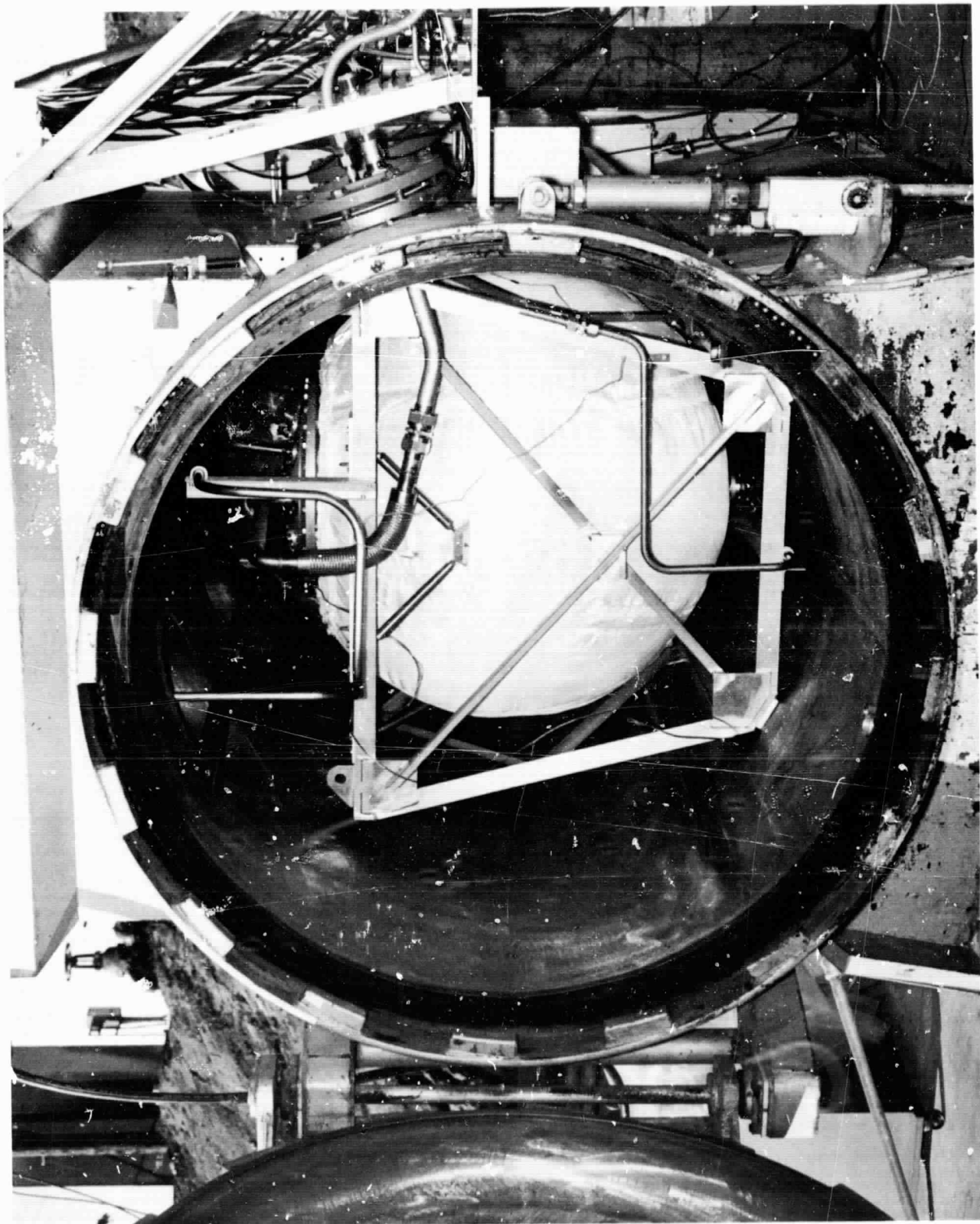
Fig. 13. Cryogenic Test Vessel Installed in Vacuum Chamber
