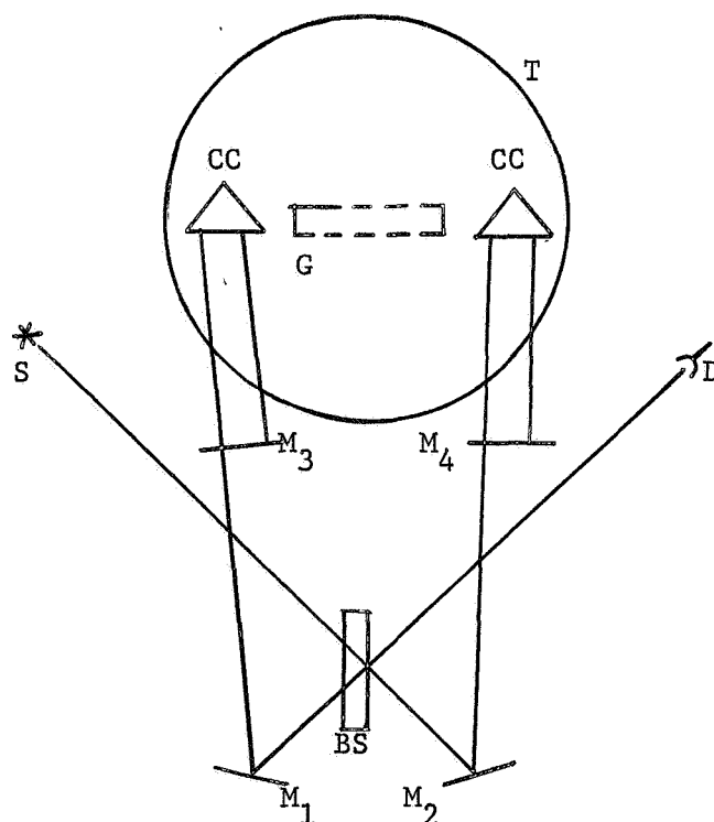
Figure 10. Asymmetric optical layout.
