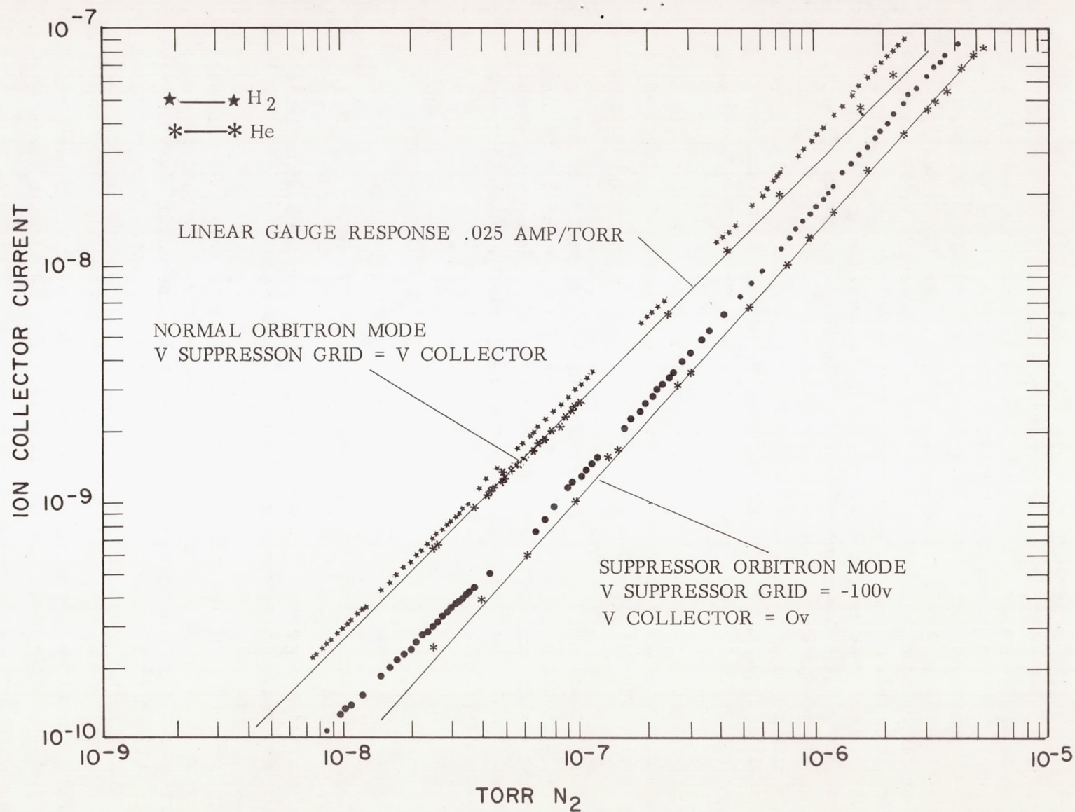
Figure 18 - Comparison of the Relative Response of the SGOG to a UHV-12 for Helium and Hydrogen. The SGOG was operated in two modes, i.e., standard orbitron mode similar to the COG (cathode potential equal ion collector potential) and the suppressor mode (cathode potential less than ion collector potential).
