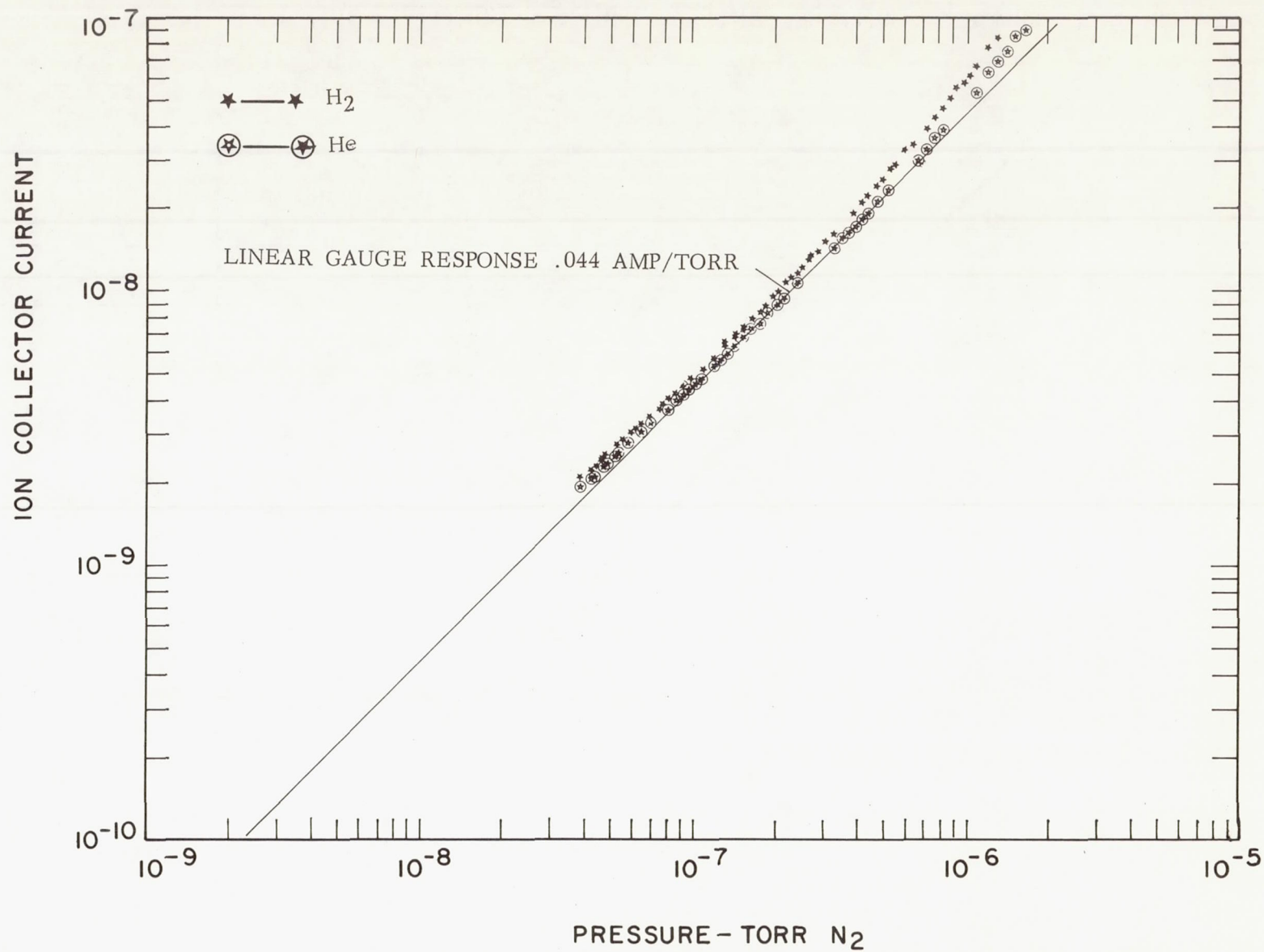
Figure 17 - Comparison of the Relative Response of the RAICOG to a UHV-12 for Helium and Hydrogen
