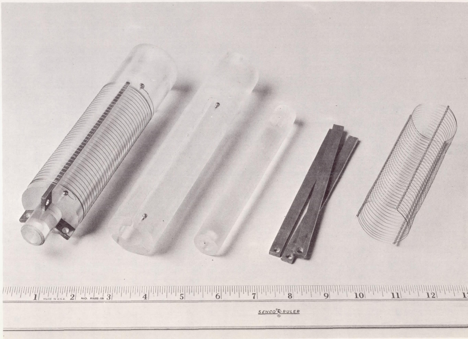
Figure 9 - Plexiglas Winding Mandrels for Fabrication of Helical Coils. Tantalum wire (0.010 in. dia.) is wound onto one of the mandrels. The coils are held in position permanently by spot welding three stainless steel rods to each turn of the coil at 120° intervals.
