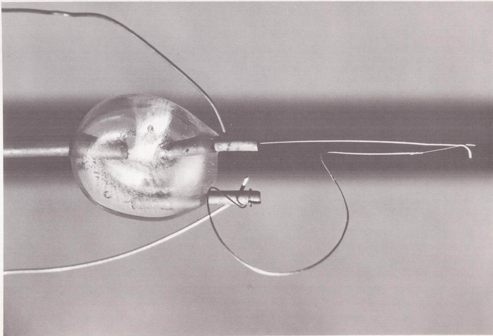
Figure 10 - Filament Mounting Unit. A tungsten filament (0.001 in. dia.) is mounted between two 0.005 in. dia. tantalum support rods. The support on the right has been shaped into a single loop spring in order to maintain tension on the filament.
