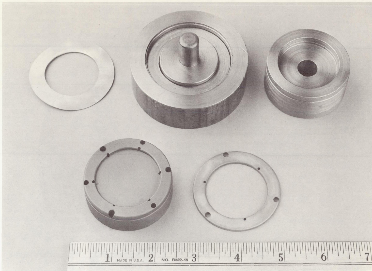
Figure 8 - Stamping Die and Drill Jig Used to Fabricate Support Ring Units. Stainless Steel blanks (0.015 in. thick) are precut and stamped. Required holes are drilled using a simple jig (lower left). Finished support ring shown at lower right.
