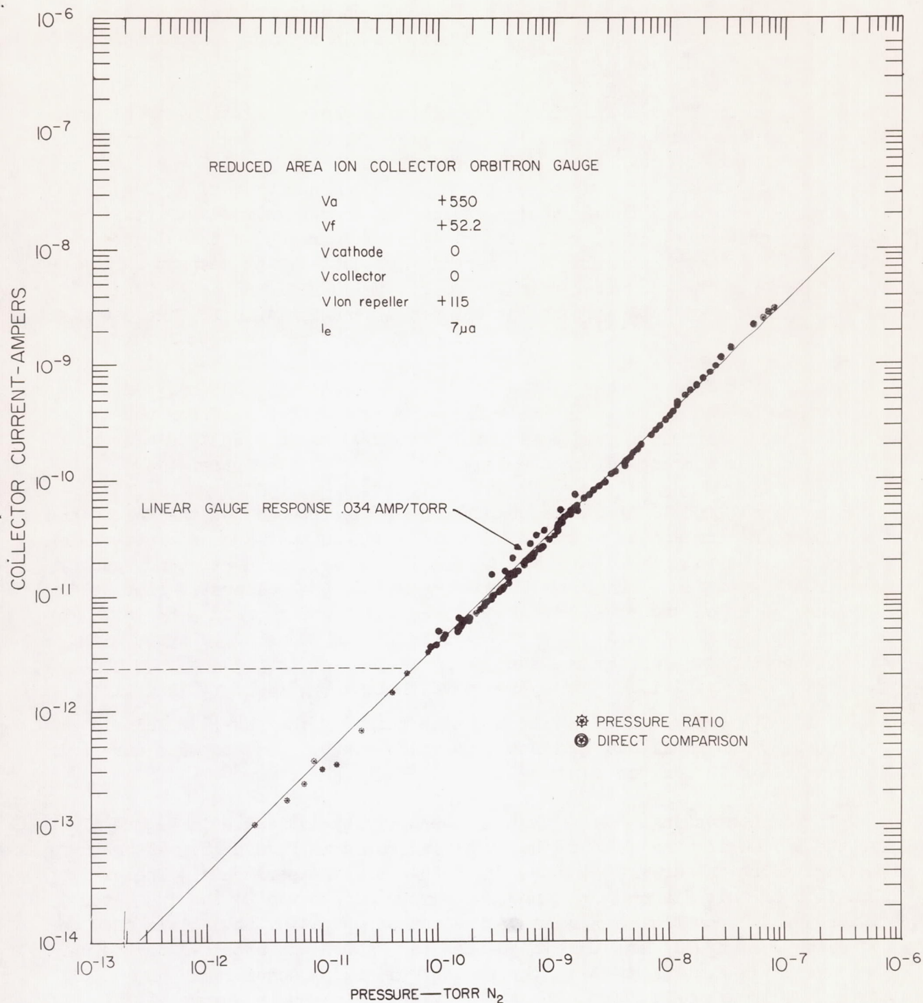
Figure 15 - Reduced Area Ion Collector Orbitron Response Curve for 7.0\mu A Emission. Ultra low pressure values plotted on the abscissa were determined by the pressure ratio technique. The dashed horizontal line represents the level of a zero suppression signal which was supplied to the electrometer during the RAICOG tests.
