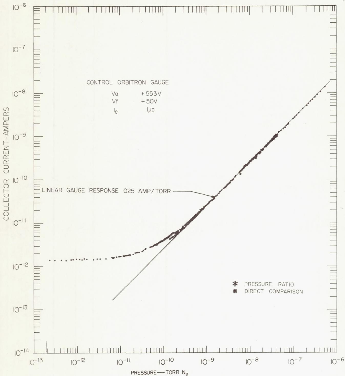
Figure 14 - Control Orbitron Response Curve for 1.0\ \mu A Emission. Ultra low pressure values plotted on the abscissa were determined by the pressure ratio technique.
