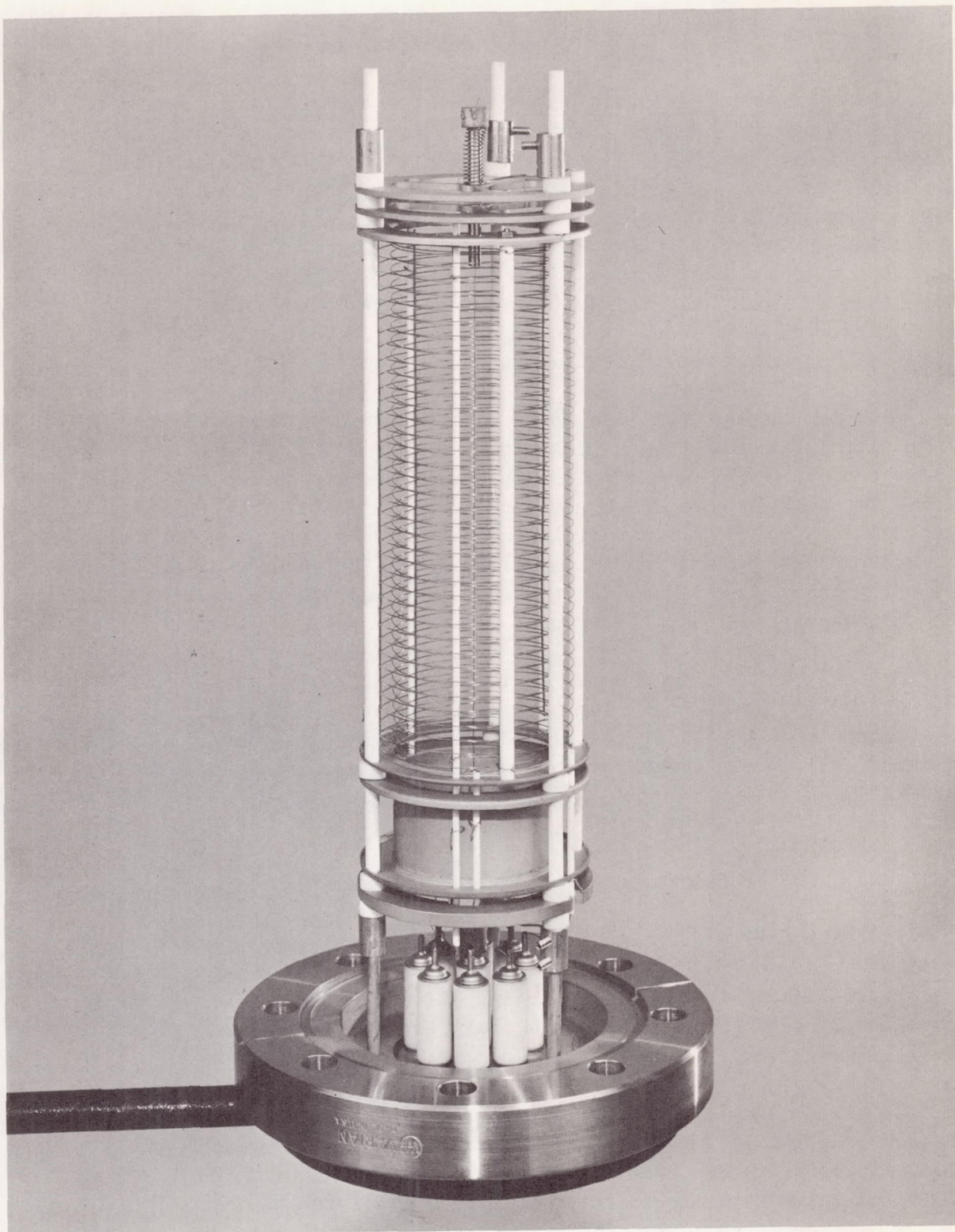
Figure 6 - Reduced Area Ion Collector Orbitron Gauge with Ion Focusing Grid (RAICOG). The outer helical coil is used to focus ion onto the inner helical coil (ion collector).
