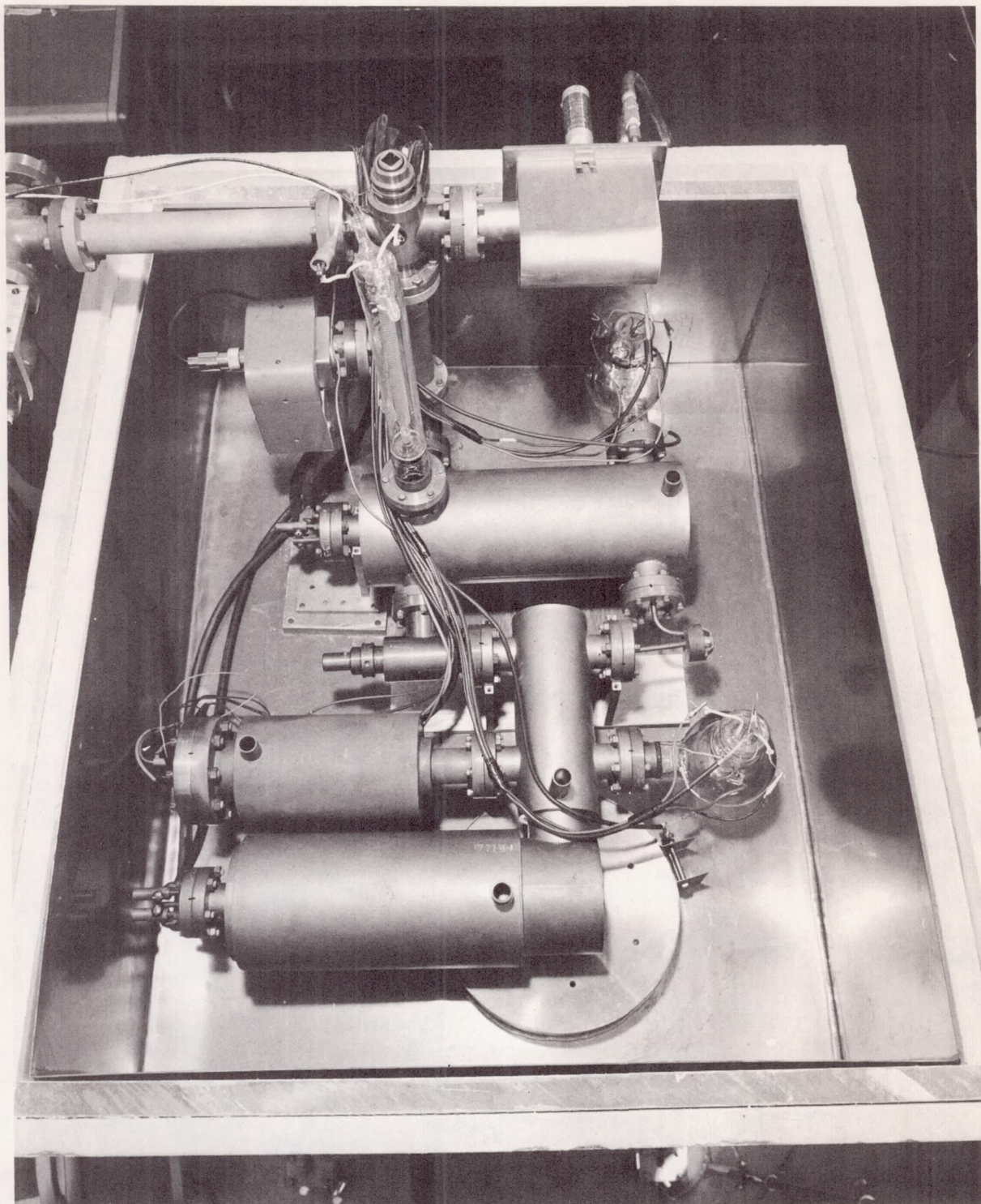
Figure 12 - UHV Pressure Ratio System. The pressure ratio system is mounted within an insulated stainless steel tank. During low pressure tests \text{LN}_2 is circulated through the doubled walled vacuum vessels and exhausted into the stainless steel tank.
