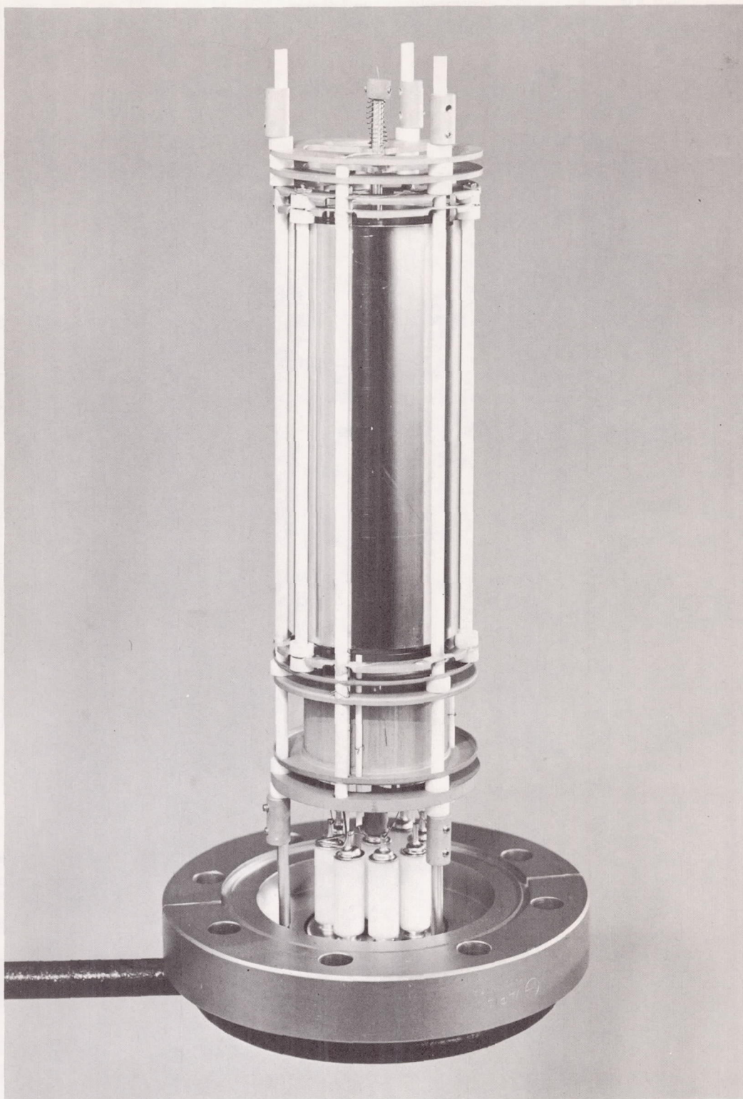
Figure 7 - Suppressor Grid Orbitron Gauge. An inner helical coil is used to suppress secondary electron emission from the solid cylindrical ion collector. Also guard ring electrodes are used to shield the ion collector.
