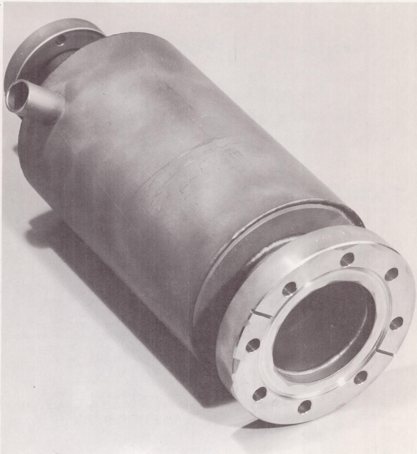
Figure 13 - Test Chamber for Orbitron Gauges. The chamber is fabricated from stainless steel and is equipped with a double wall. \text{LN}_2 is circulated through the double walled region during ultra low pressure tests.
