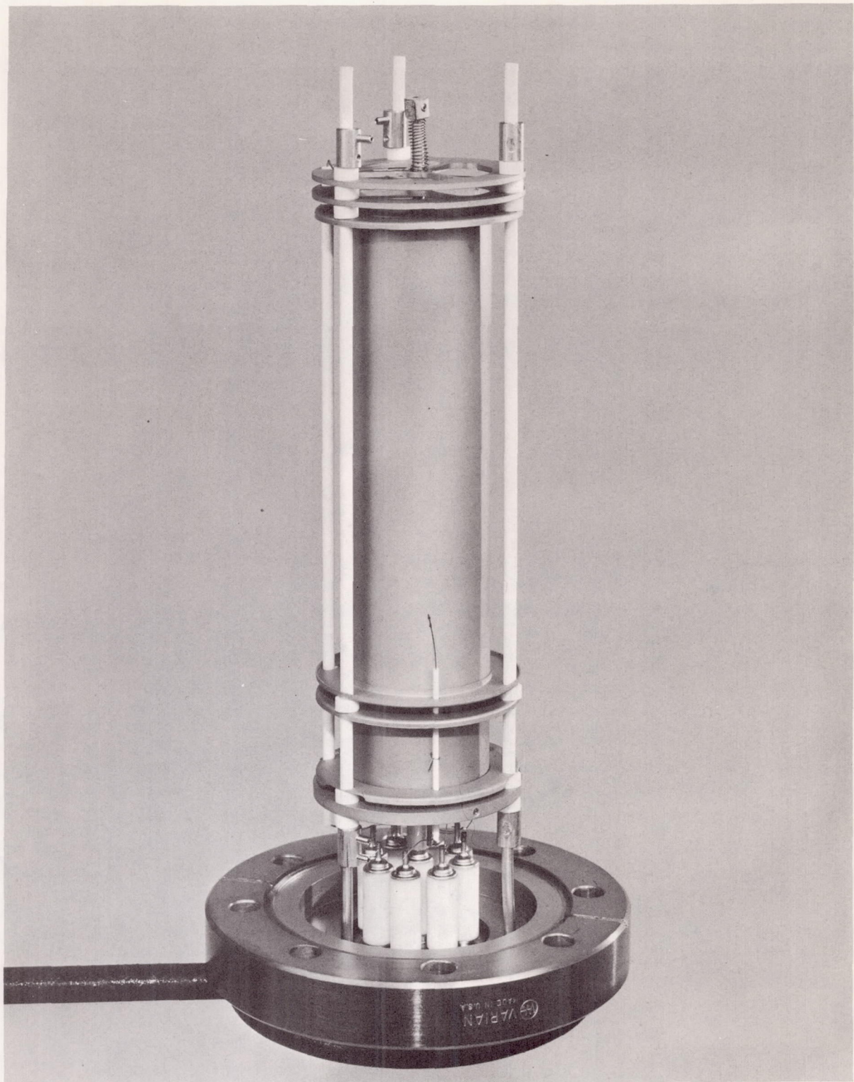
Figure 3 - Control Orbitron Gauge (COG). The cathodes are mounted on three ceramic rods. Location of the elements is established by 1/8 in. thick ceramic spacers threaded onto the ceramic support rods.
