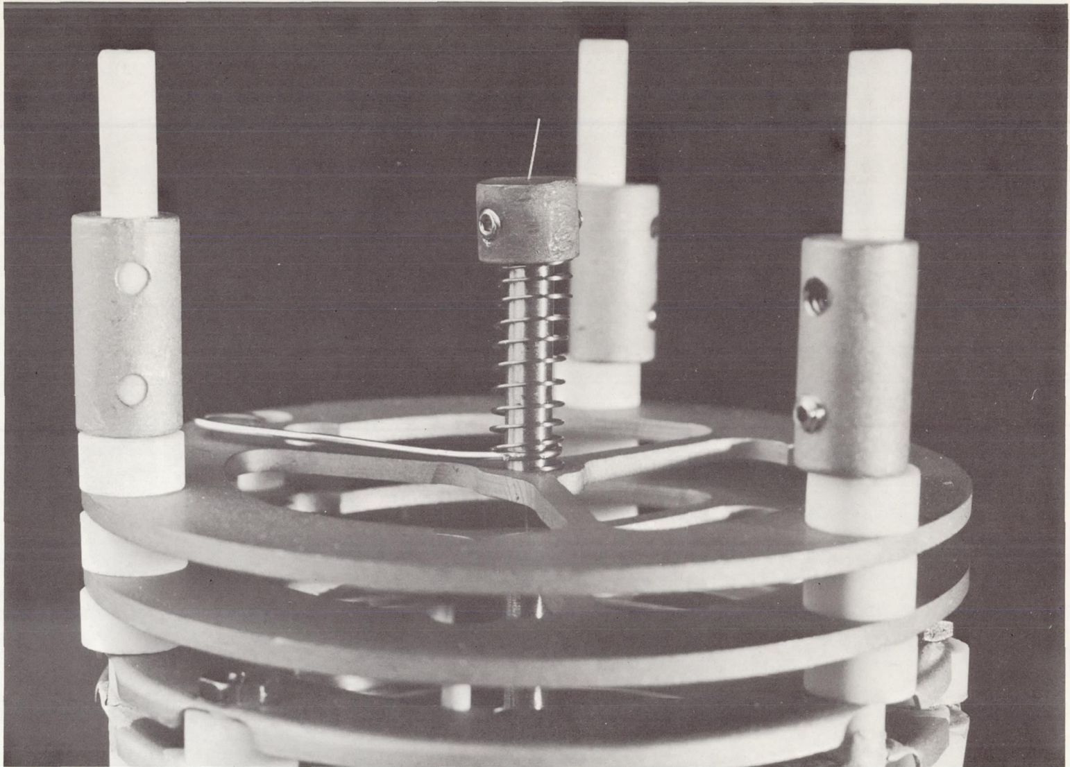
Figure 4 - Spring Loading Anode Support Assembly. The 0.005 in. dia. anode passes out of the electron orbiting region through a 1/8 in. O.D. x 0.010 in. (wall thickness) x 1/2 in. long tube and is attached to a circular clamp. This clamp is spring loaded by means of a tungsten helical spring.
