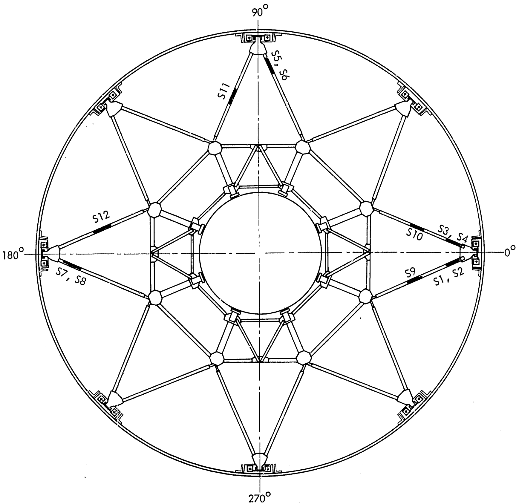
Figure 2. Sectional View of the Experimental Shroud-Payload Structure and Locations of Strain Gage Transducers
