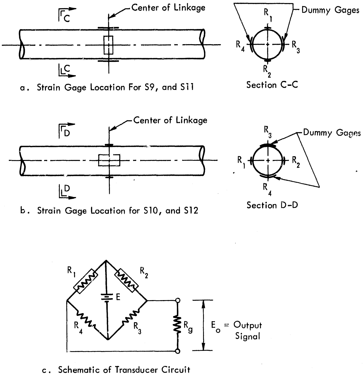
Figure 7. Arrangement of Strain Gage Transducers for Measuring Lateral Load and Schematic of the Transducer Circuit
