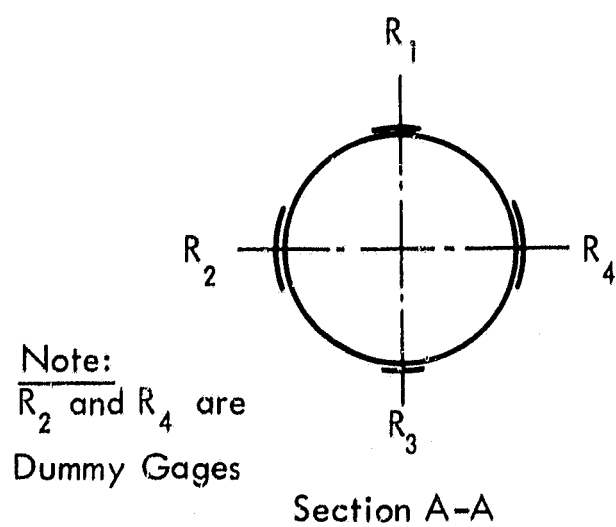
a. Strain Gage Location
