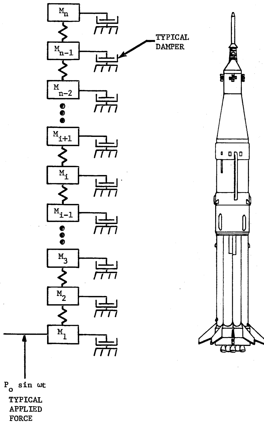
FIGURE 2. STRUCTURAL MODEL OF THE SATURN I-B
