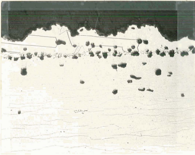
Coated TD-Ni Sample 118 140 hours
