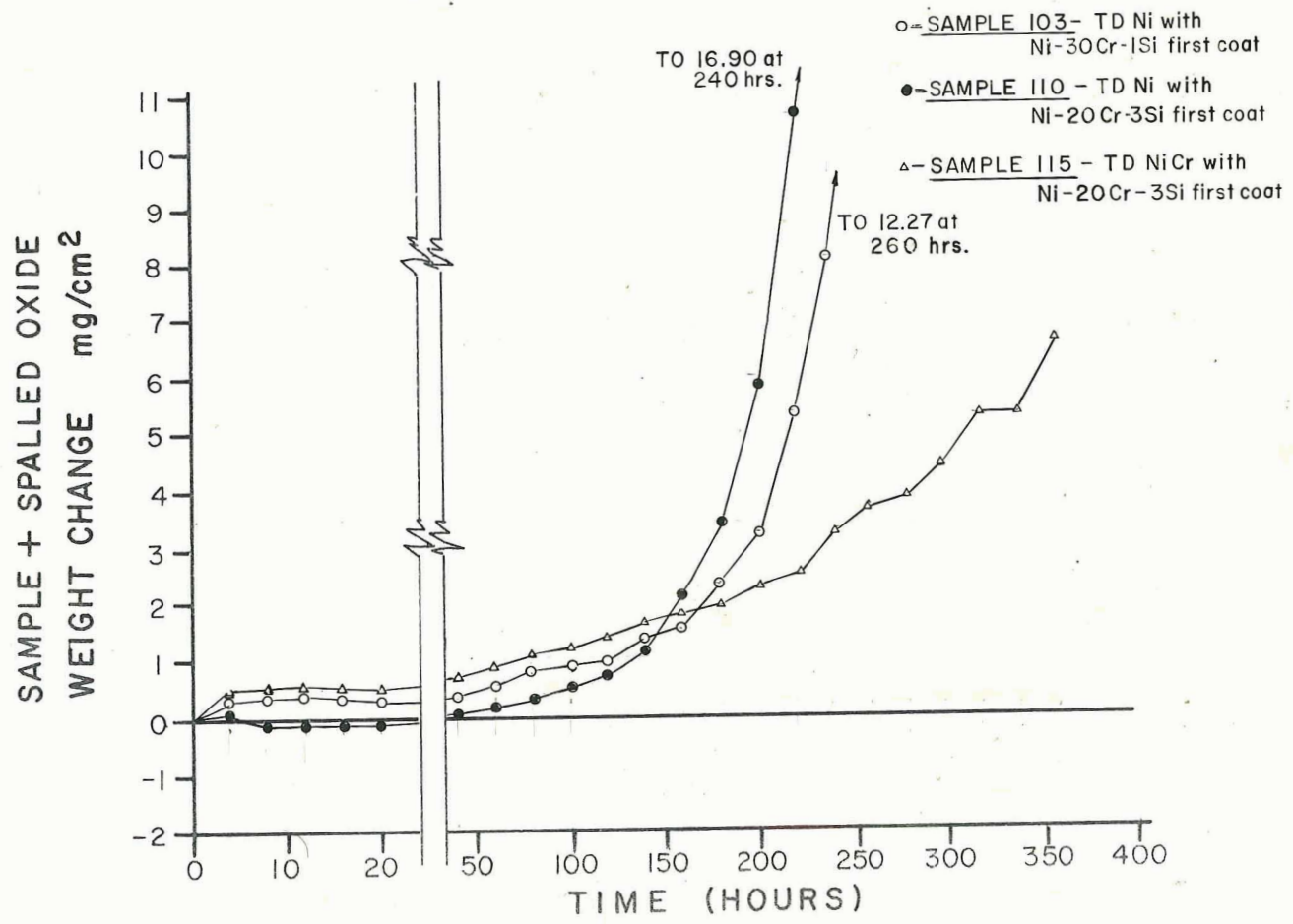
Figure 51. Oxidation behavior in Standard Test at 2300°F. All samples with 10 mg/cm 2 Al-20Co second coat and #5 diffusion treatment.
