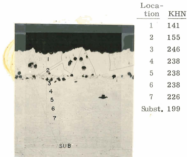
Oxidized - 100 hours Sample 105
