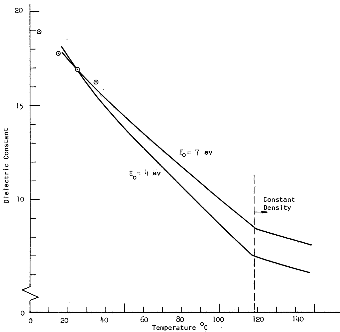
Figure 3. Estimated Dielectric Constants for Liquid and Dense Gaseous \text{NH}_3 . Circled points are measurements of Grubb, et al. (8)
