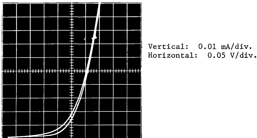
Figure 22. An Oscillogram of the Forward Characteristics of PT#14 with \Delta P = 0
