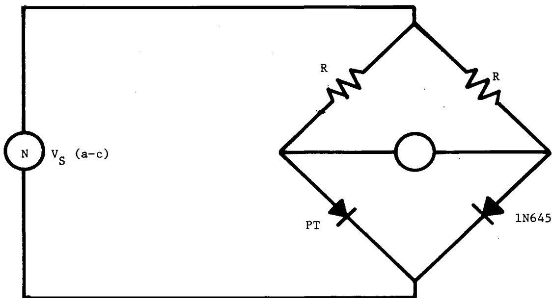
Figure 37. A Diode-Resistor Bridge Read-out Circuit
