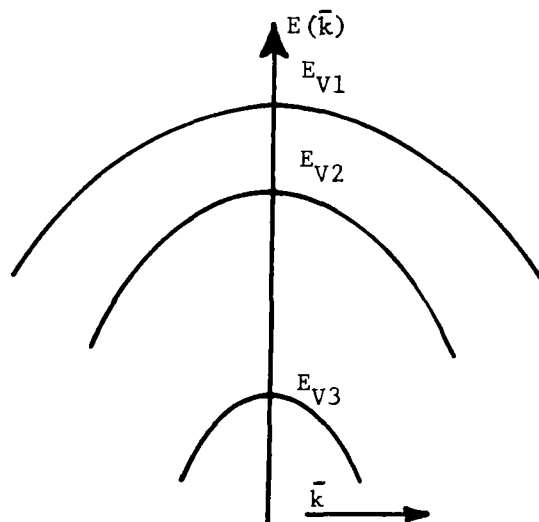
Figure 2. The Split Valence Bands of Silicon for a Compressional Stress (Ref. 5)
