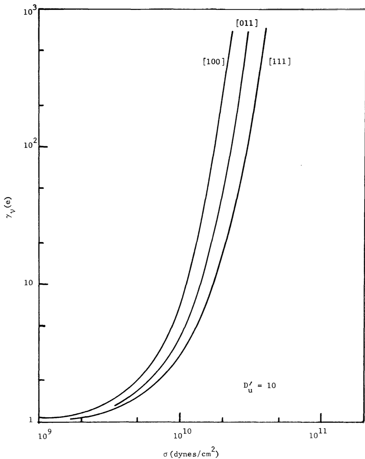
Figure 5. Ratio of Stressed to Unstressed Minority Carrier Density for a [100], [011] and [111] Uniaxial, Compressional Stress
