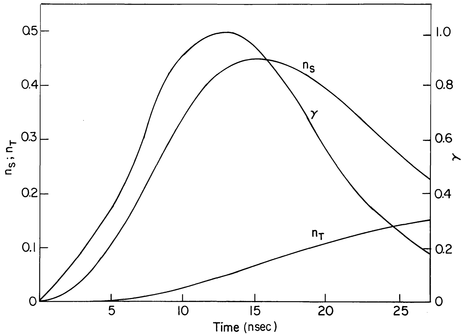
Fig. 16 Calculated Time Variations of the First Excited Singlet and Triplet Level Populations of Anthracene for a Pumping Pulse \gamma(t) . In Eq. (9) \tau_S = 4.9 \text{ nsec} , \eta = 0.1 , and \rho \approx 10^{-3} .
