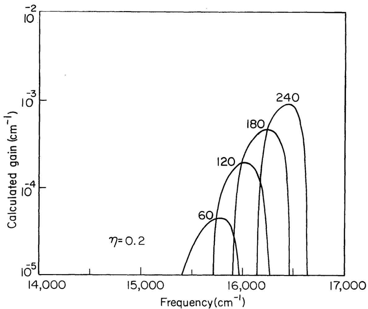
Fig. 20 Calculated Gain Curves for Rhodamine B at Various Times During Flashlamp Pumping (see Fig. 19). Intersystem Crossing Parameter \eta = 0.2
