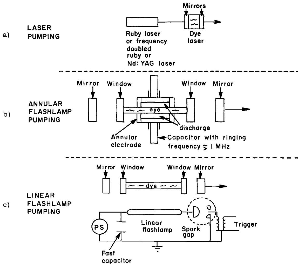
Fig. 3 Methods of Dye Laser Excitation
