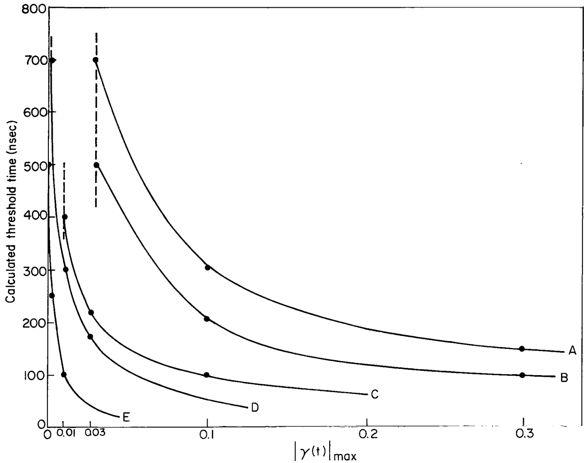
Fig. 13 Time at Threshold for Oscillation of Rhodamine 6G as a Function of Pumping Intensity |\gamma|_{\max} , where \gamma(t) is given in Fig. 8. The cavities used had broadband mirrors and estimated gains required for threshold as follows:
