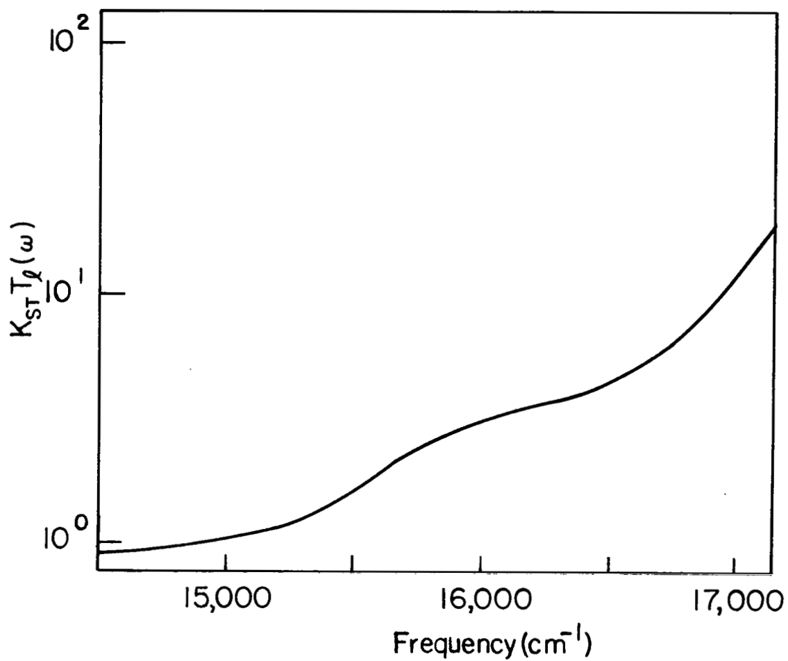
Fig. 23 k_{ST} T_l(\omega) vs \omega from Eq. (18) for Rhodamine B.
