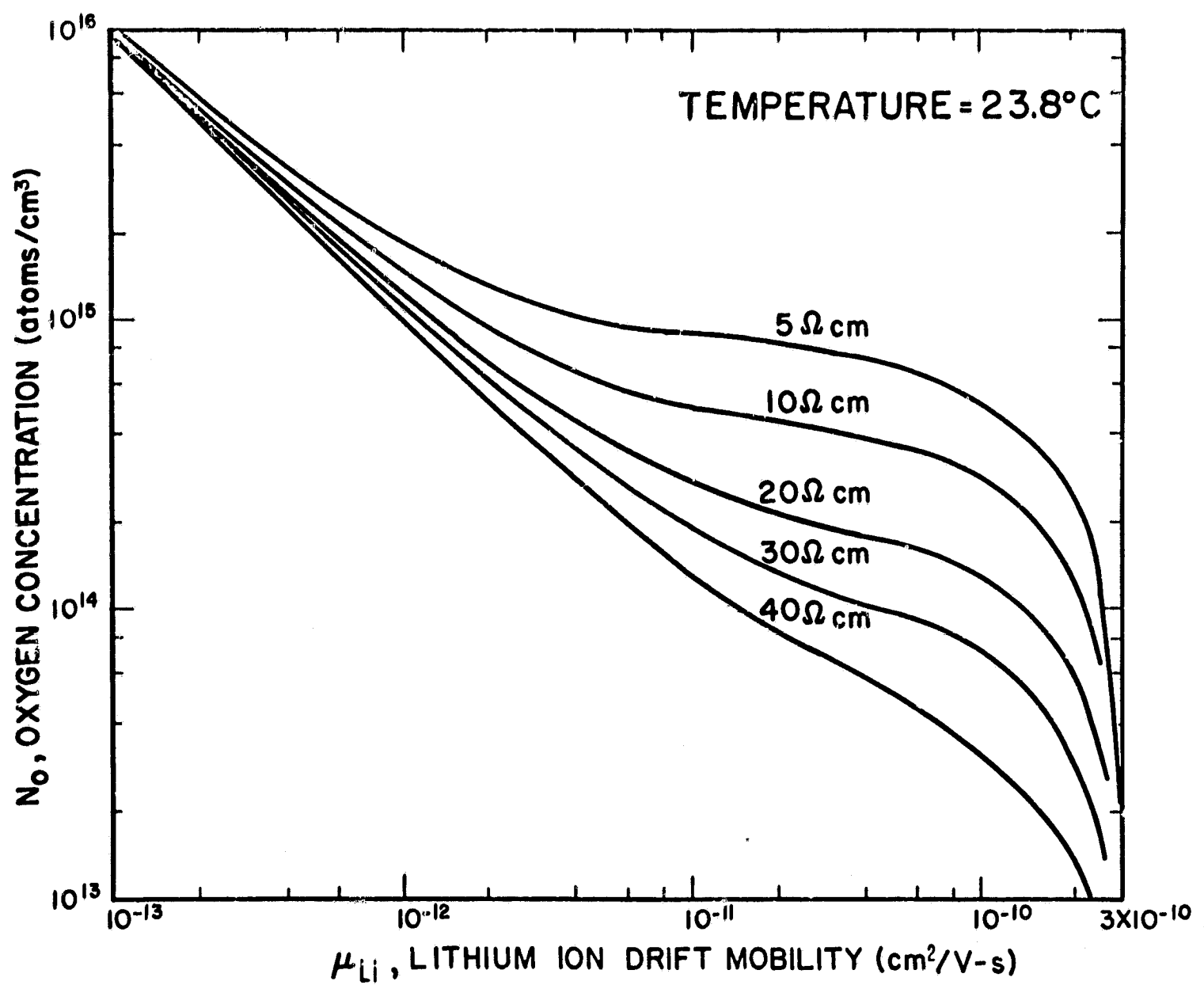
Fig. 2 Oxygen concentration, N_O , as a function of lithium ion drift mobility, \mu_{Li} , at 23.8°C for different specimen resistivities, from Eq. (4).
