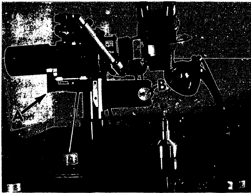
Fig. 3 Mechanical Wire Bond Pulling Machine
