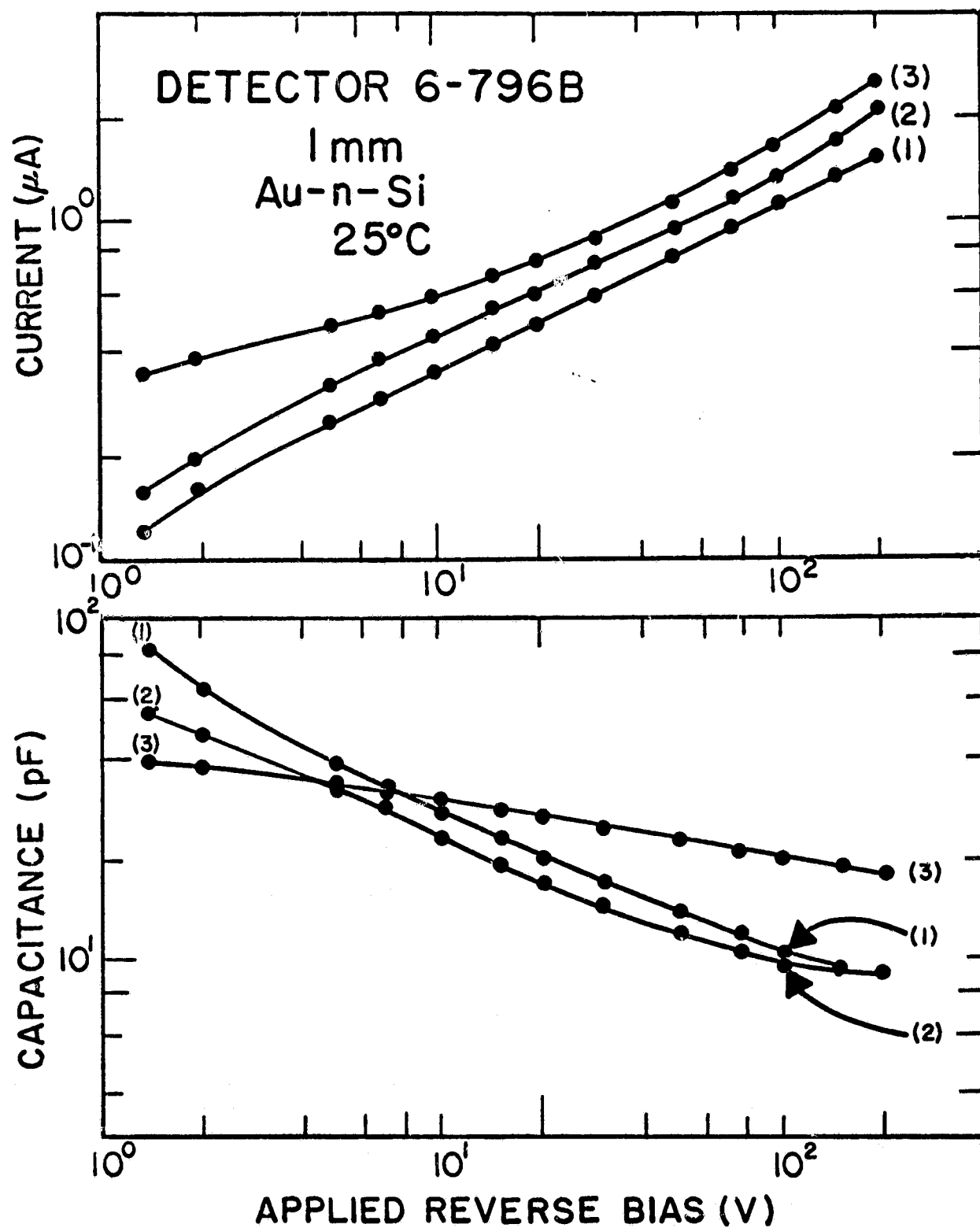
Fig. 7 Current- and capacitance-voltage characteristics of a 1-mm thick silicon surface-barrier detector before irradiation (1) and after damage by 10^{14} (2) and 10^{16} (3) 600-keV electrons/cm 2 incident on the rear contact.
