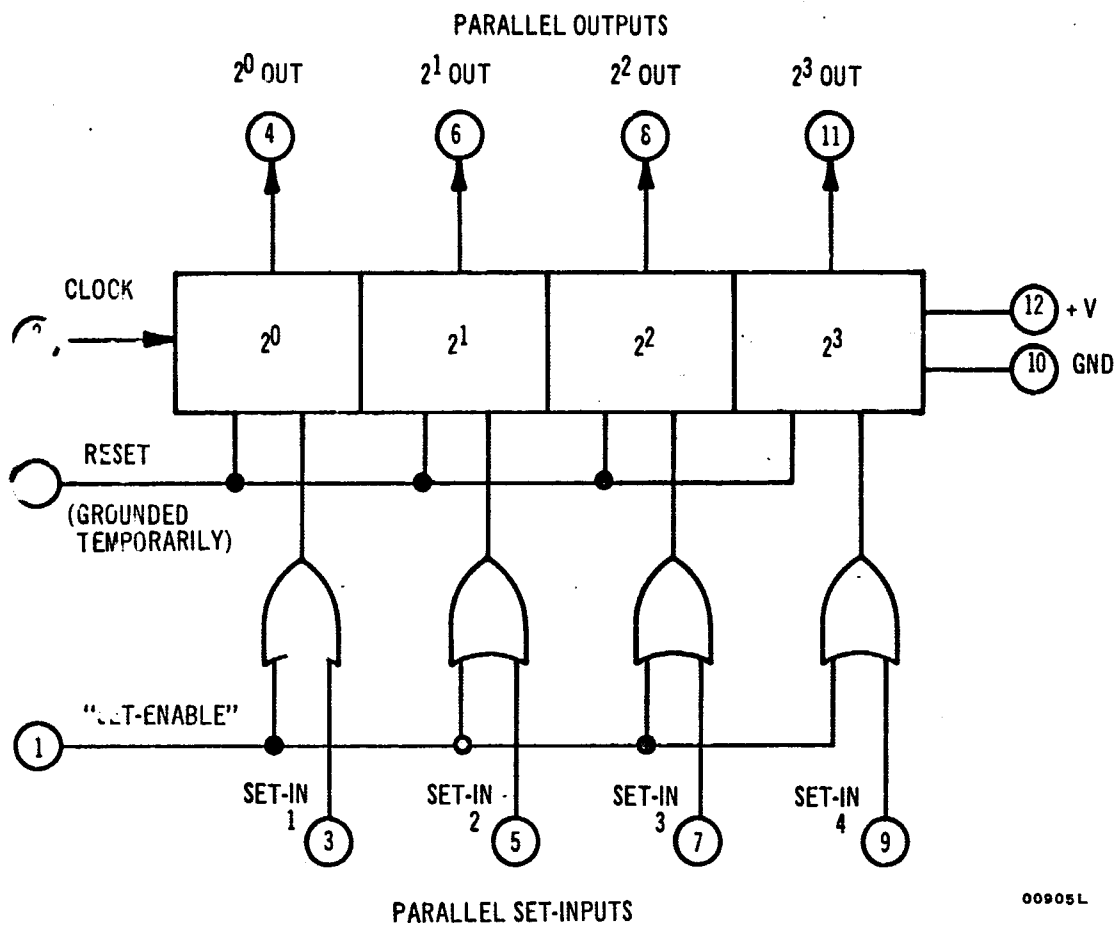
A. BLOCK DIAGRAM
