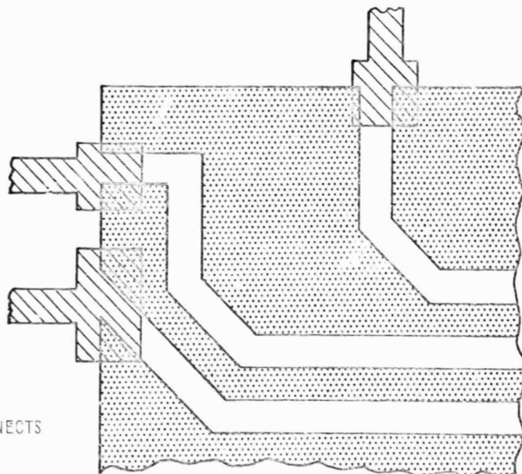
B. MISALIGNMENT OF 0.2 MIL ALONG X-AXIS AND 0.2 MIL ALONG Y-AXIS
