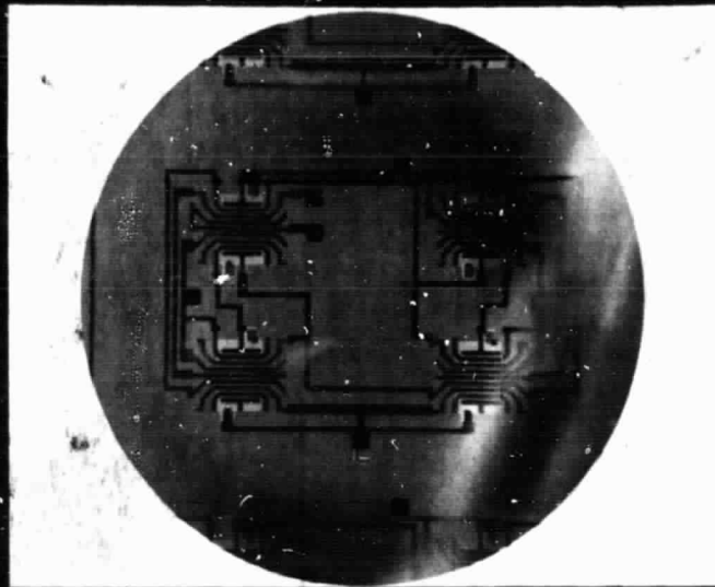
01238P Figure 7. Metalization Pattern of J-K Flip-Flop
