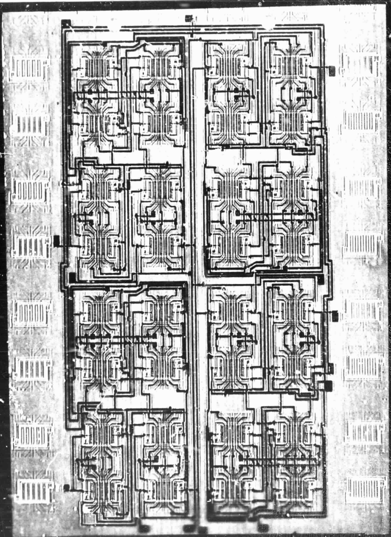
Figure 1. Layout Pattern of Four-Stage Counter
