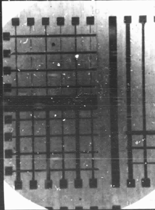
C. TWO-LEVEL METAL PATTERN
