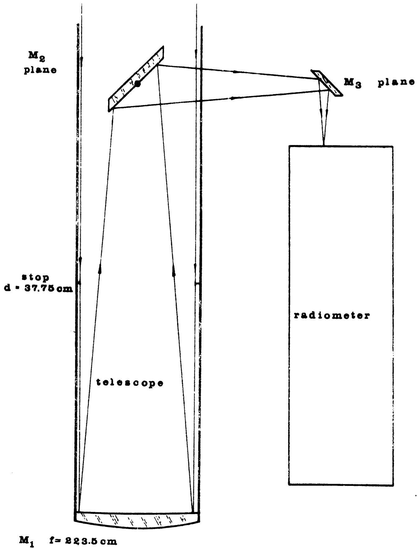
TELESCOPE OPTICS
