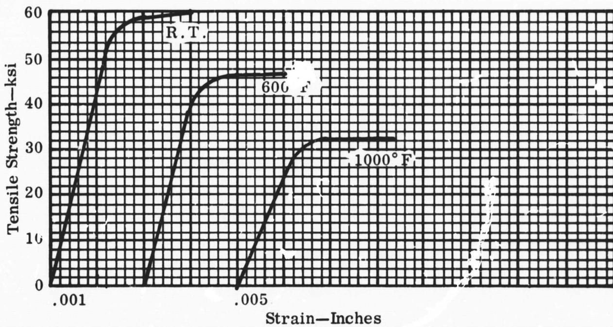
Figure 2-11. Cross-Rolled Beryllium Sheet Typical Stress Strain Curves (19)
