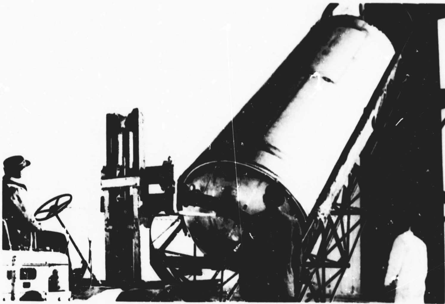
Figure 2-44. 7000 Gallon Tank, 8' Diameter x 24' Length, Produced from 0.025" Titanium Alloy Ti-6Al-4V ELI(38)
