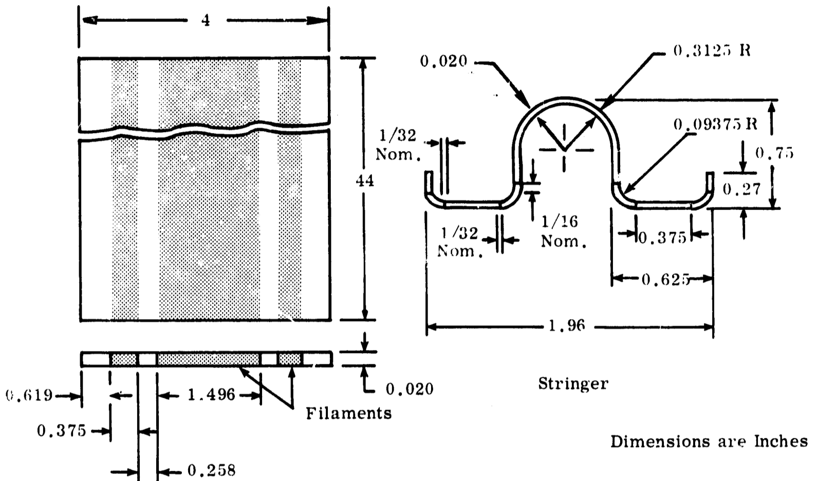
Figure 3-15. Selectively Placed Unidirectional Filament (101)
