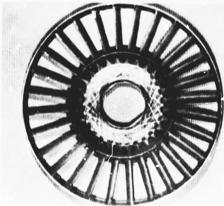
Figure 3-21. Prototype Glass-Boron/Epoxy First-Stage Compressor Disc (B1)
