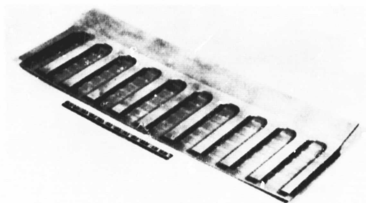
Figure 2-34. Completely Processed Subscale Y-Ring Segment (33)
