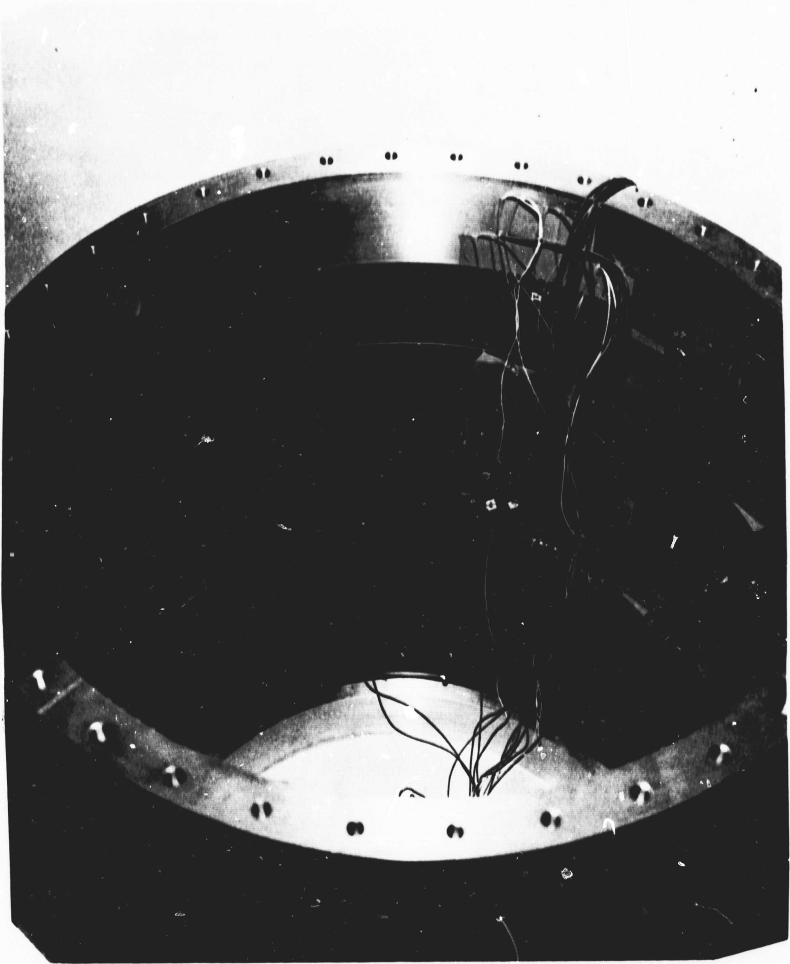
Figure 3-20. Rib Enforced Structure With Instrumentation (90)
