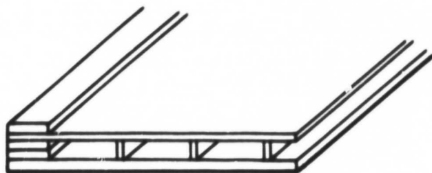
Figure 2-32. Fabrication Layup Design Used to Prepare Y-Ring Structure (33)
