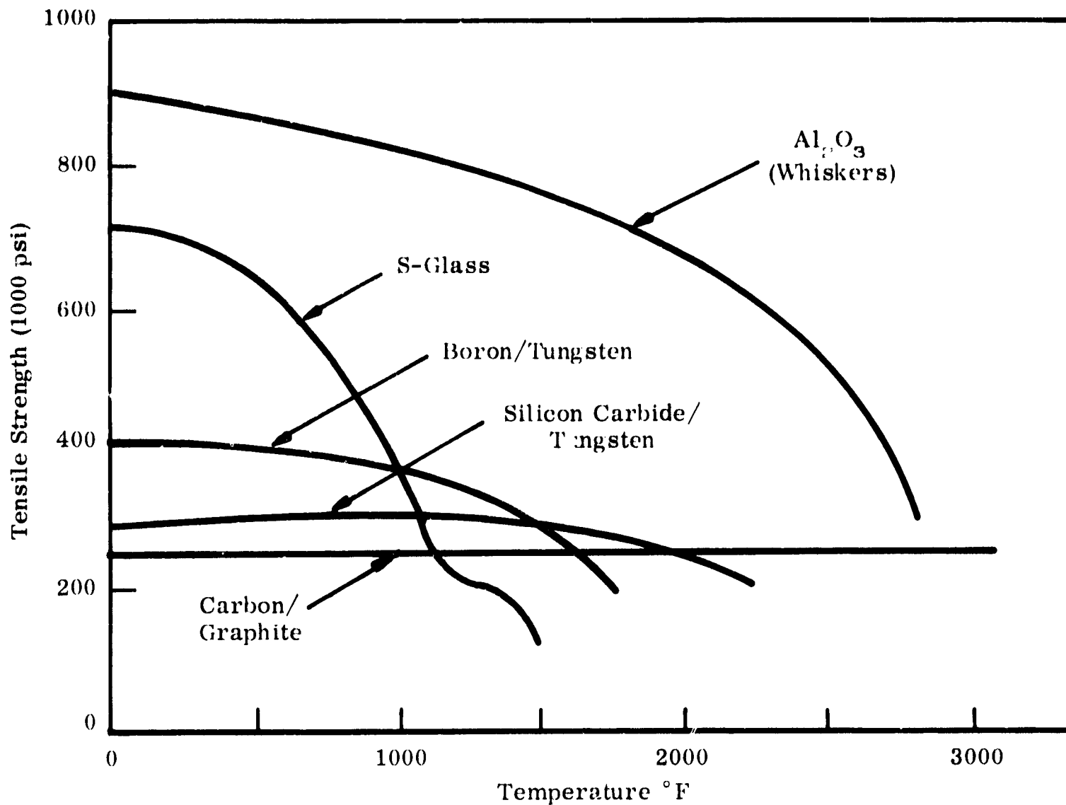
Figure 3-7. Strength Retention at Elevated Temperature of Various Commercially Available Fibers (49)
