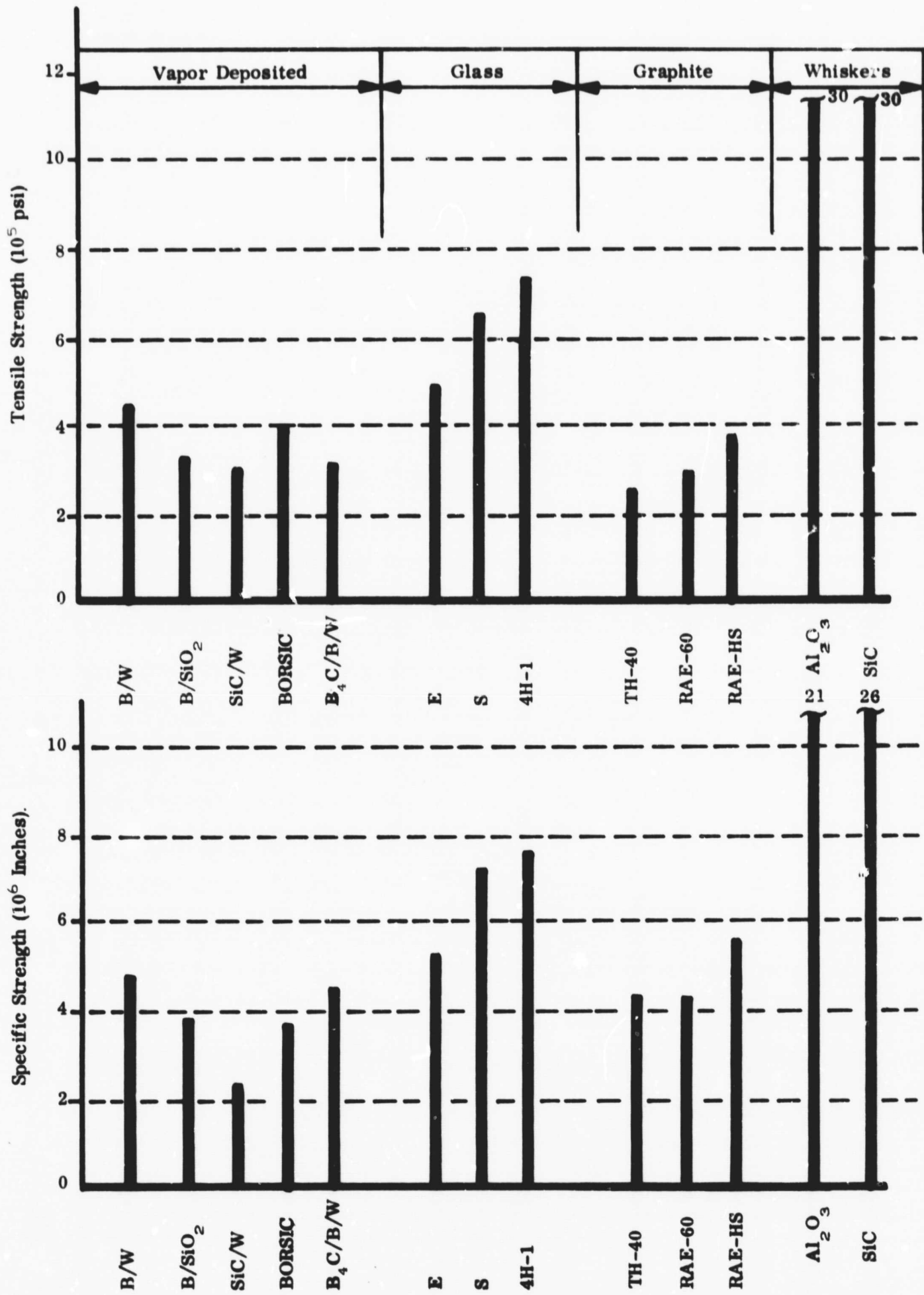
Figure 3-4. Strength Characteristics of Reinforcing Fibers (4, 50)
