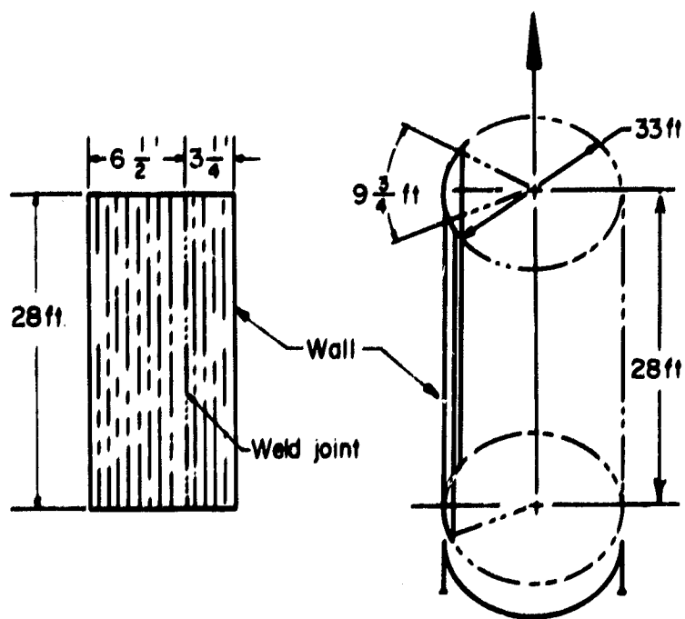
Figure 2-36. Final Production Panel (33)
