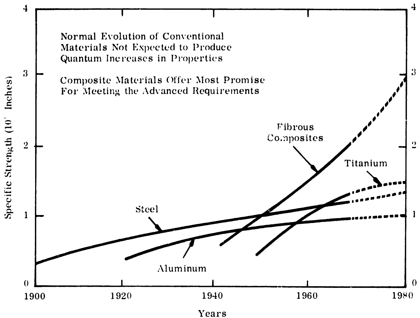
Figure 3-2. Specific Strengths (Strength-to-Weight Ratios) of Various Structural Materials over the Period 1900 to 1980 (115)
