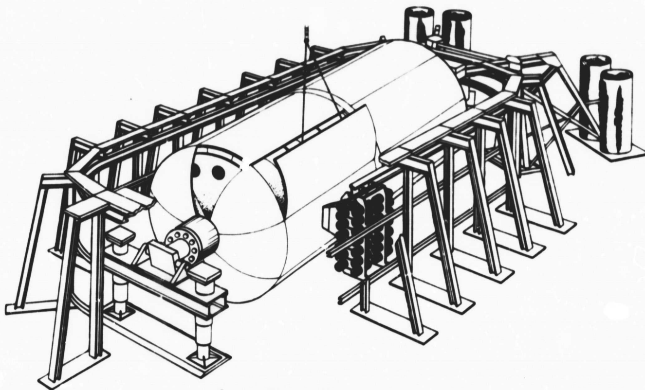
1 MANDREL ASSEMBLY
