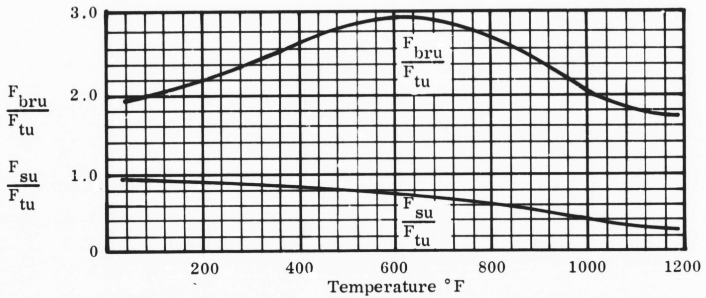
Figure 2-10. Cross-Rolled Beryllium Sheet Bearing and Shear Strength (19)
