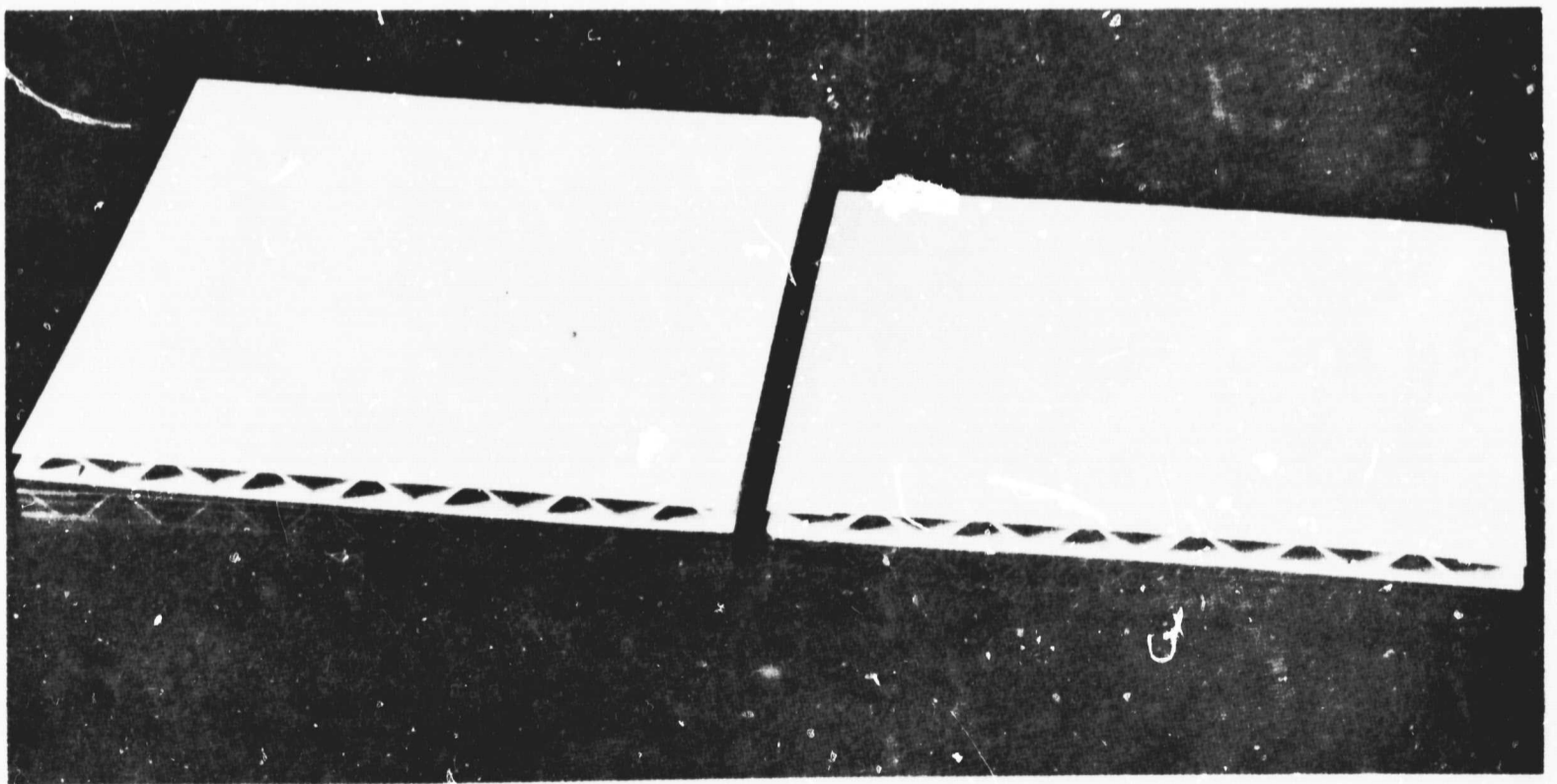
Figure 2-26. Photograph of Beryllium Panel 67-1 After Section and Leaching (27)
