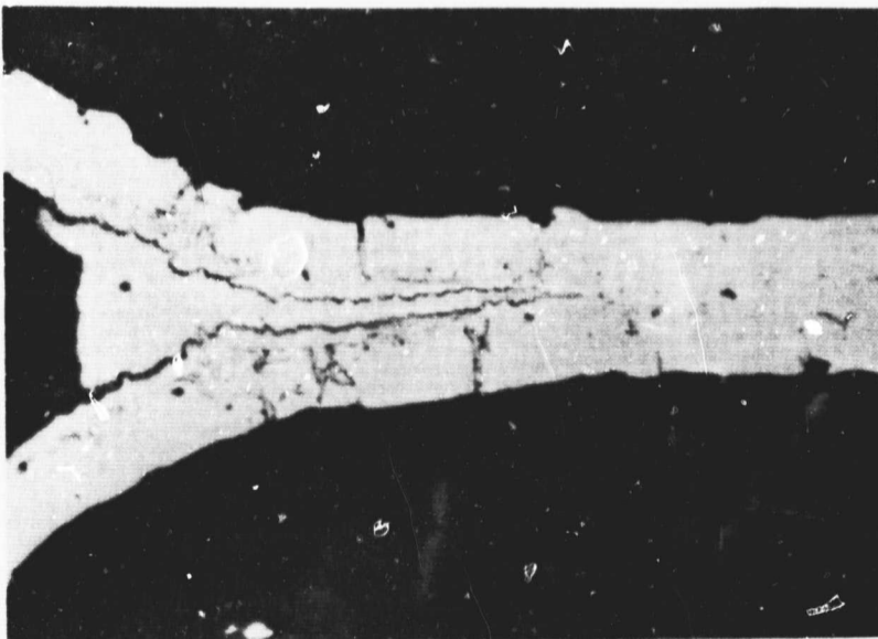
Figure 2-22. Honeycomb Sandwich Joints Using Beryllium Foils (25)
