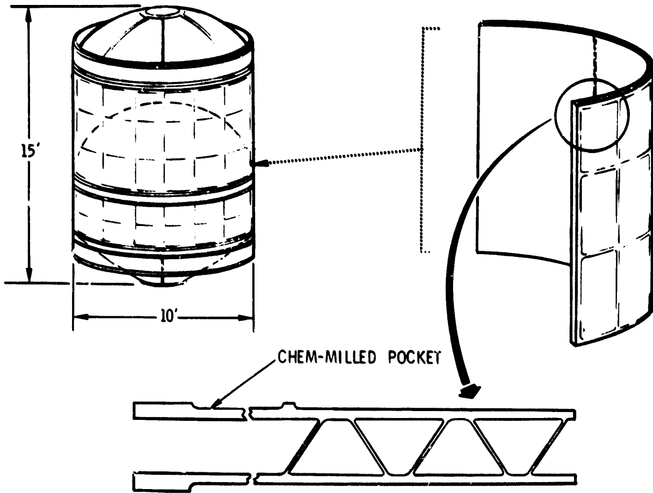
Figure 2-37. Titanium Conjugate Tankage Structure (33)
