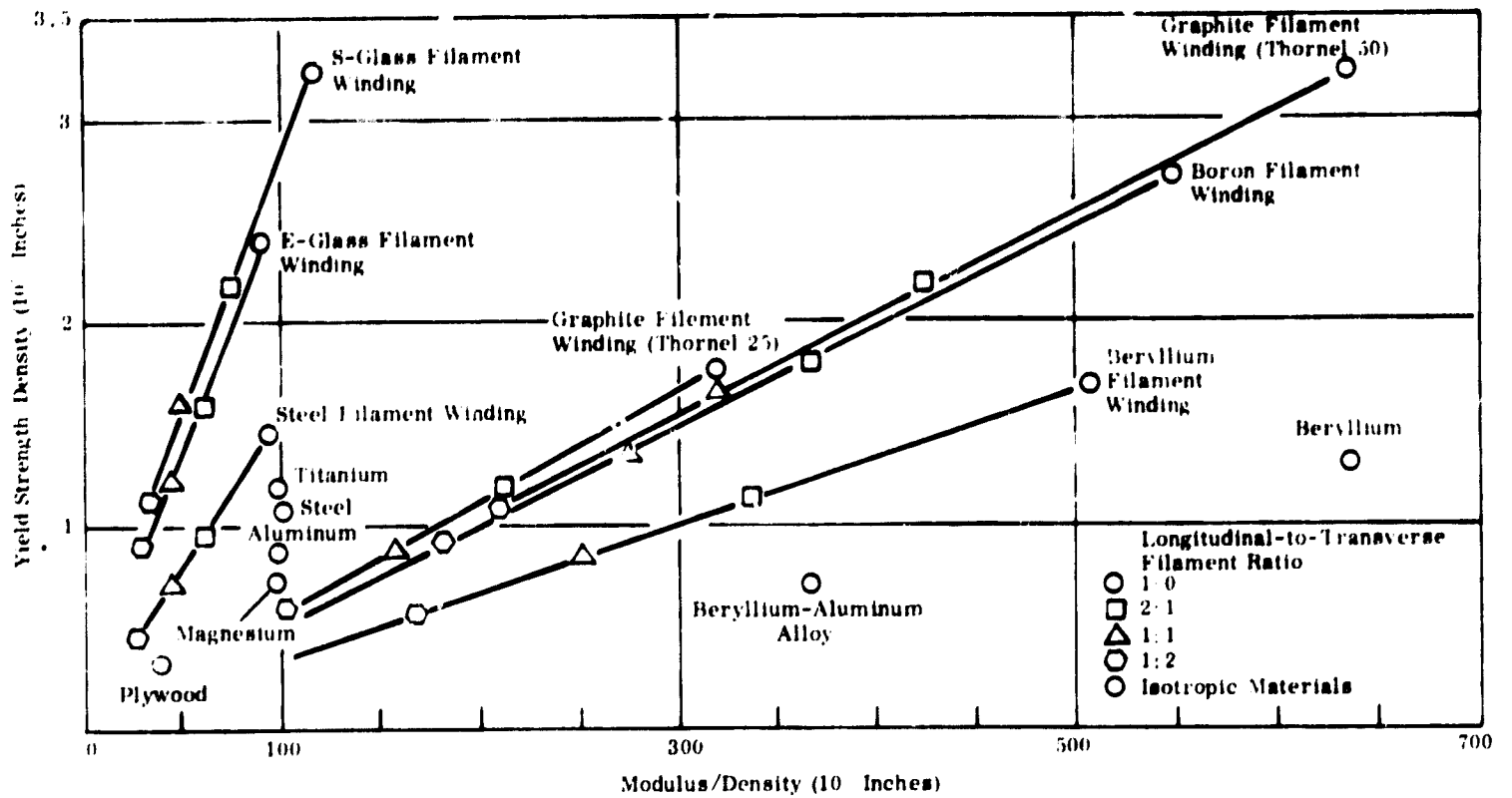
Figure 3-1. The Relative Structural Efficiency of Various Filament-Wound Composites Compared to some Conventional Isotropic Materials (114)
