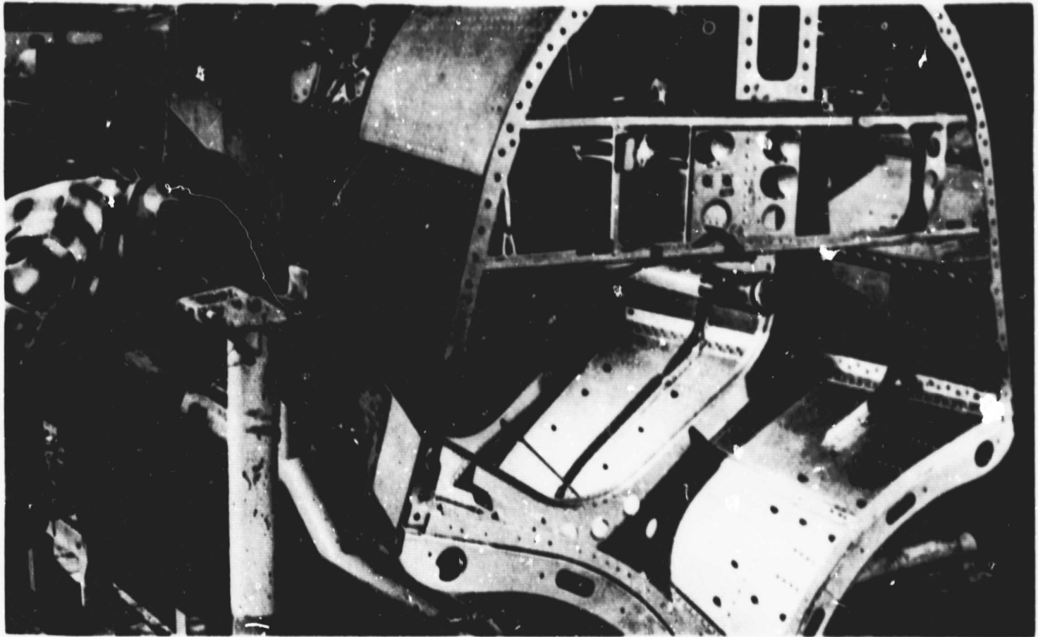
Figure 2-41. Aft Fuselage Sections. The tail assembly shown above is a titanium structure—the basic part of the aft fuselage section of the McDonnell F4C being assembled at Republic Aviation Corporation. Titanium comprises more than 25 percent of the flyweight of this portion of the aircraft, and 90 percent of it is load-bearing. (38)
