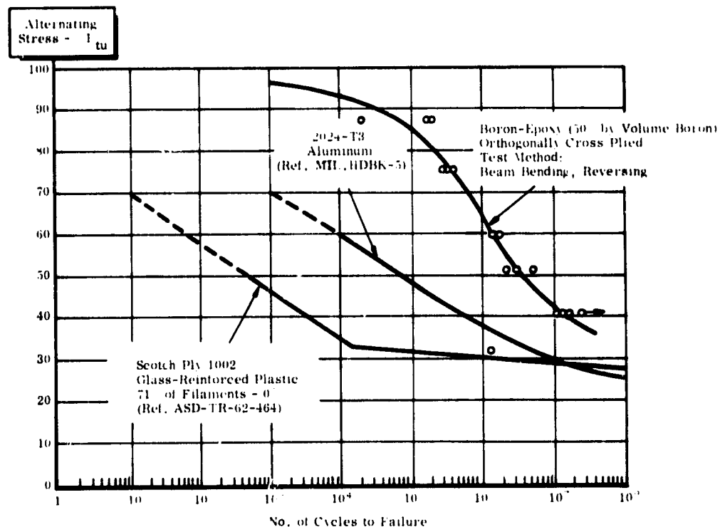
Figure 3-11. S-N Curves Comparing Fatigue Data of Boron-Epoxy Composites with Glass-Reinforced Plastic and 2024-T3 Aluminum (83)
