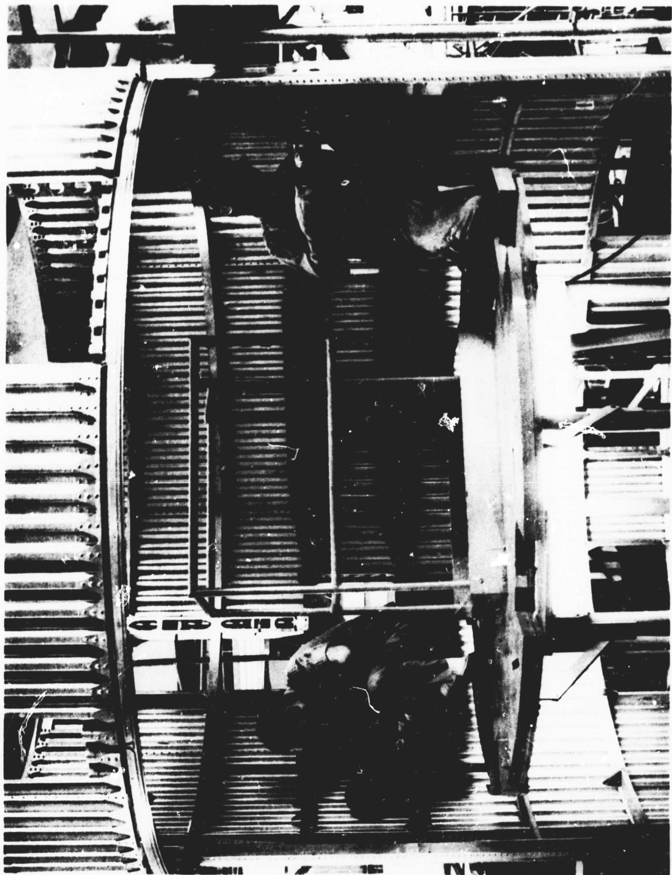
Figure 2-19. MOL Use of Beryllium for Rigidity (118)
