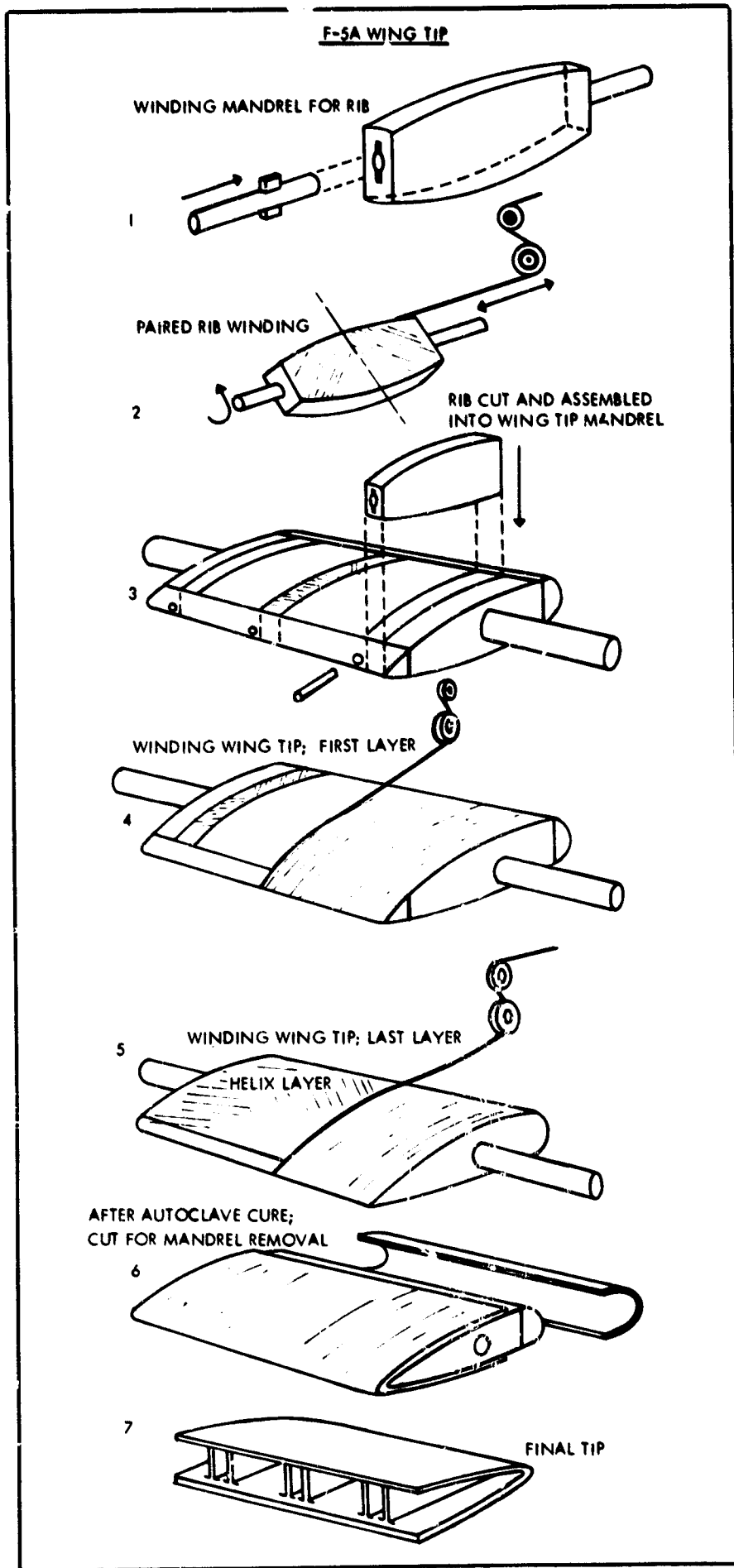
Figure 3-25. Procedures for F-5A Wing Tip Fabrication (93)
