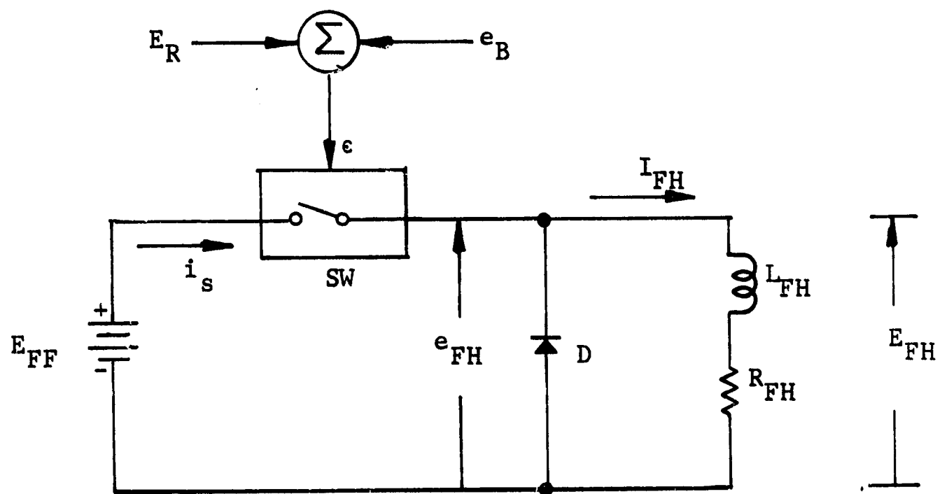
SWITCHING REGULATOR
