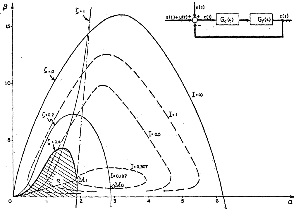
Fig. 1. Squared-error minimization in the parameter plane.
