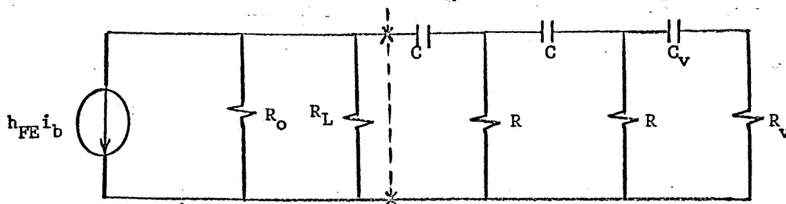
Transistor phase shift equivalent circuit
