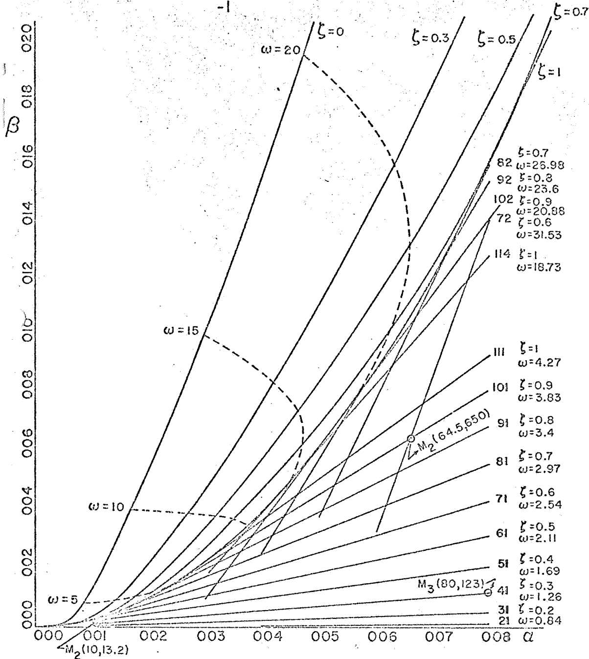
FIG.2 SINGULAR LINES IN THE PARAMETER PLANE FOR FIG.1 G_1 = \frac{k}{s^2} .
