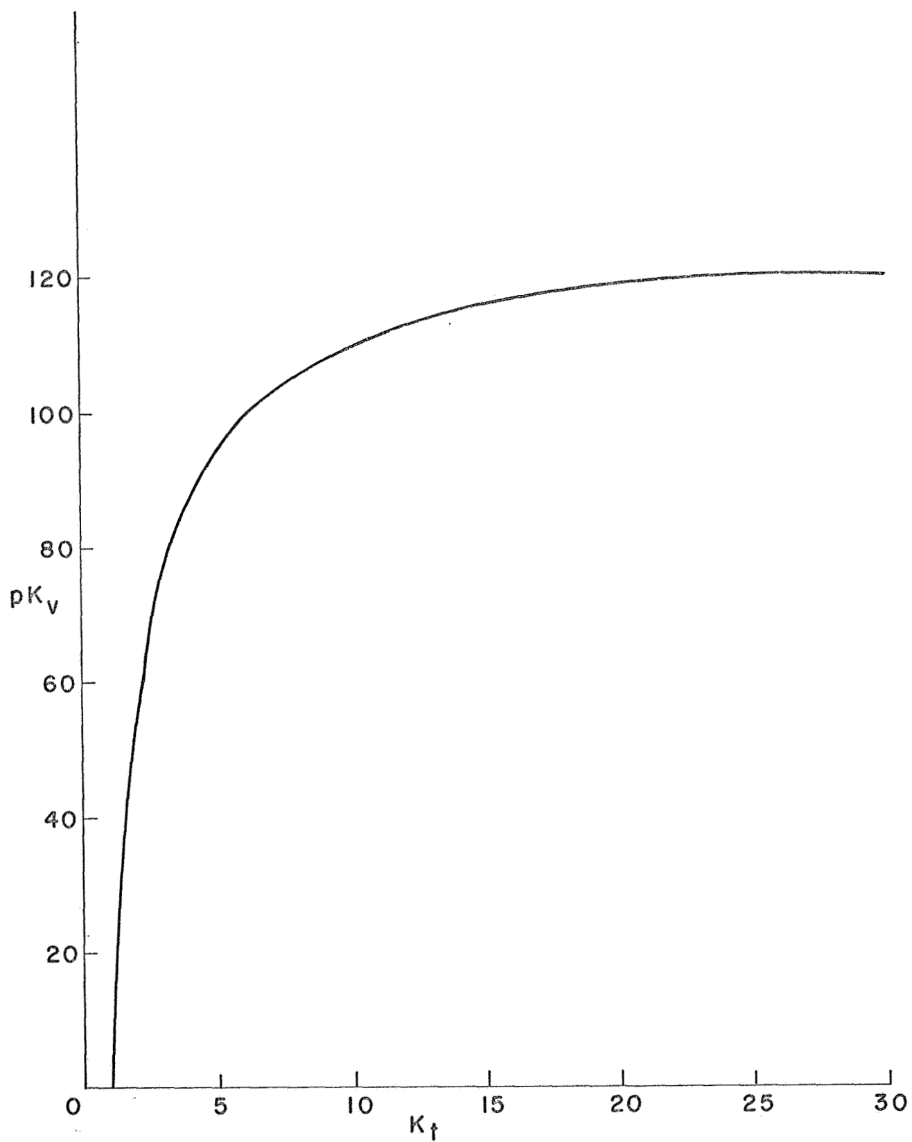
Fig. 7a. Plot of Constraint on K_v , normalized coordinates
