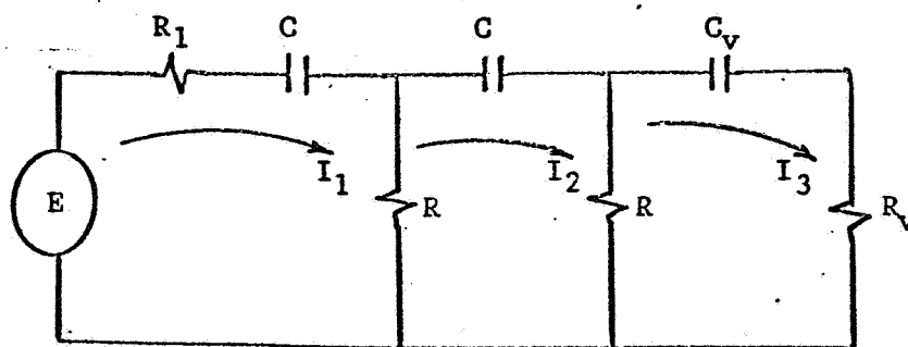
Transistor phase shift equivalent circuit
