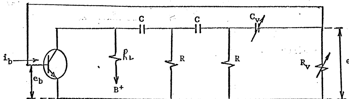
Transistor phase shift oscillator
