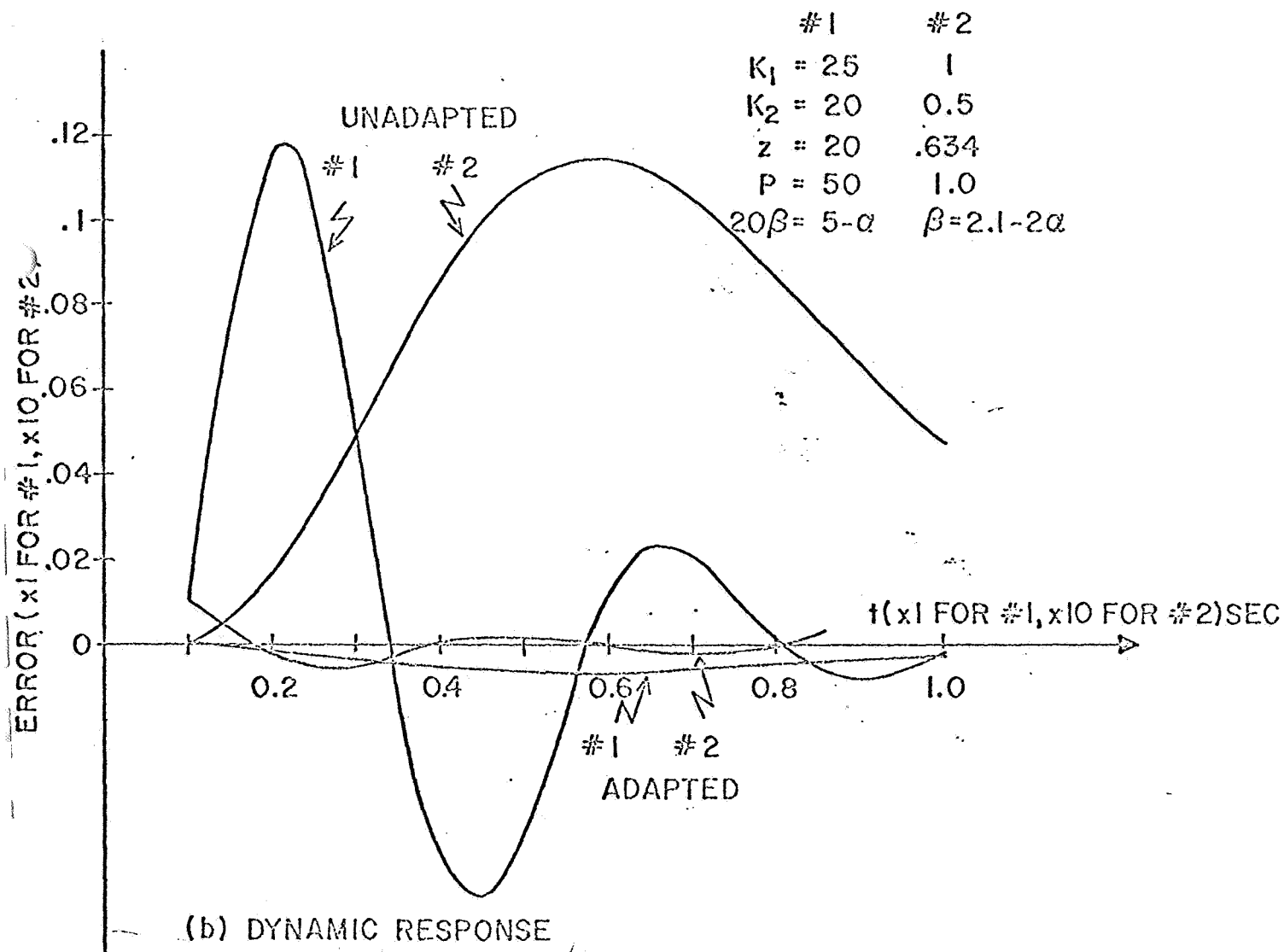
FIG.8 SELF-ADAPTATION WITH FEEDBACK GAIN.
