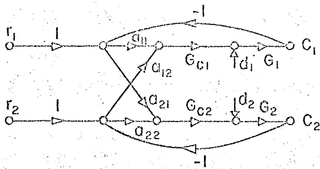
FIG.1 FLOWGRAPH OF A LINEAR MULTIVARIABLE SYSTEM.
