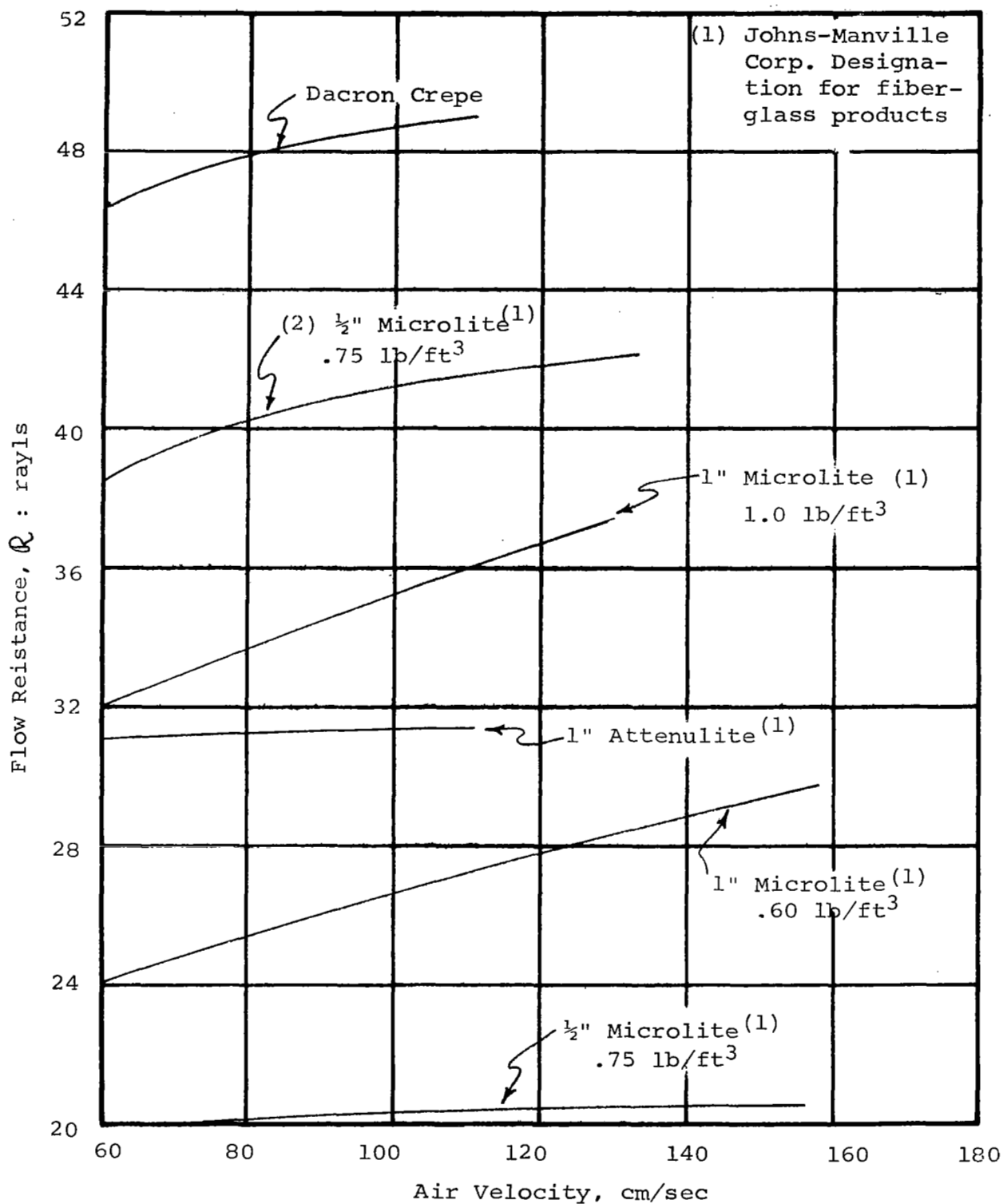
FIGURE 11 - FLOW RESISTANCE OF CANDIDATE ABSORBER MATERIALS
