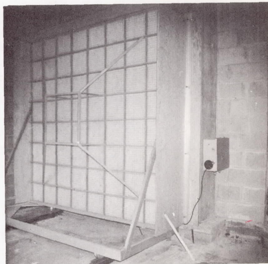
External view of moving absorber
