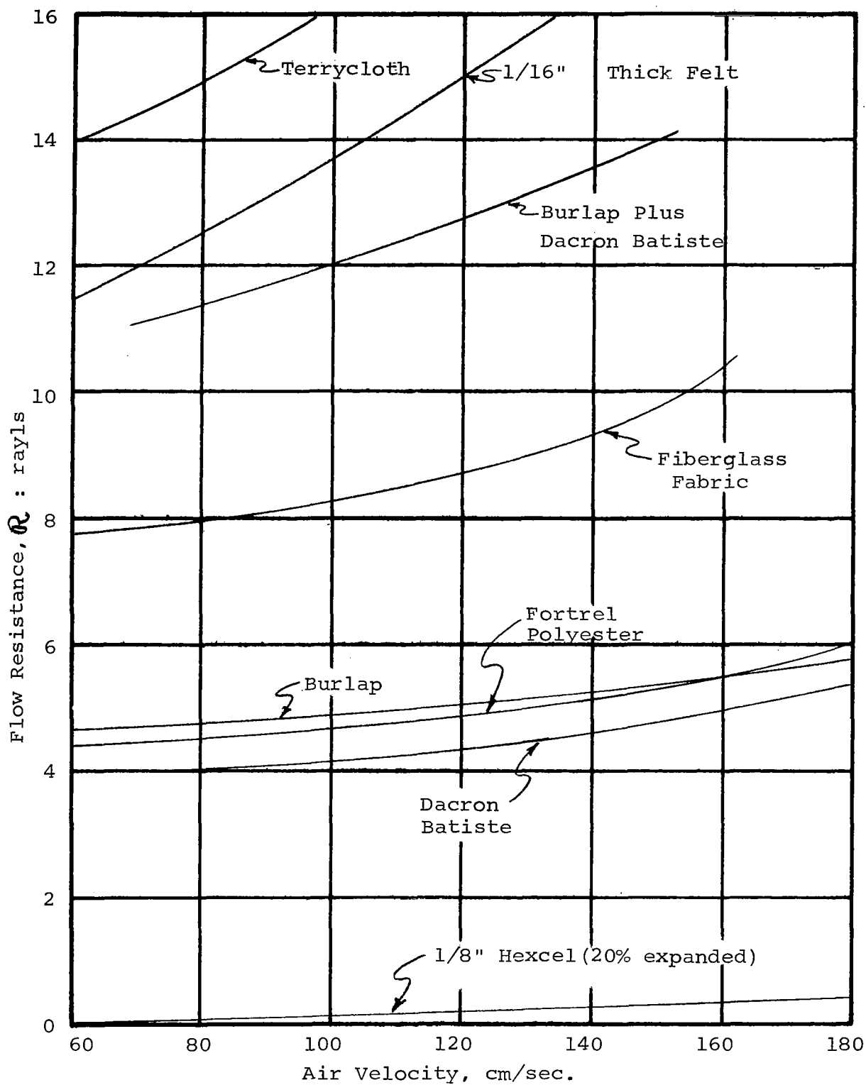
FIGURE 10 - FLOW RESISTANCE OF CANDIDATE ABSORBER MATERIALS
