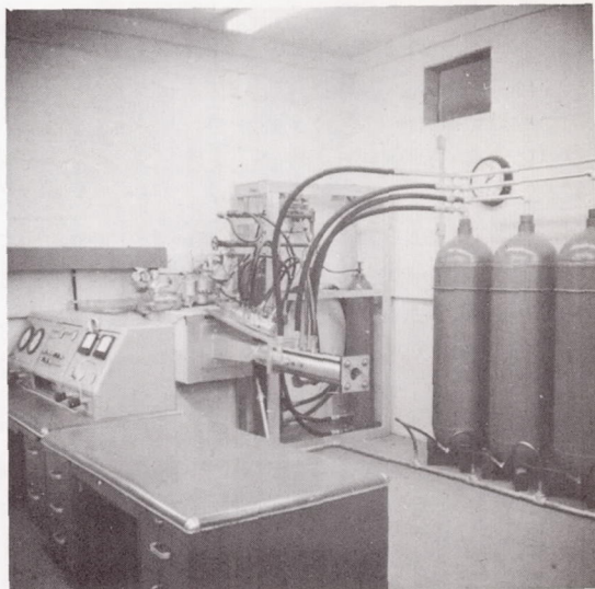
Internal View of Control Room
