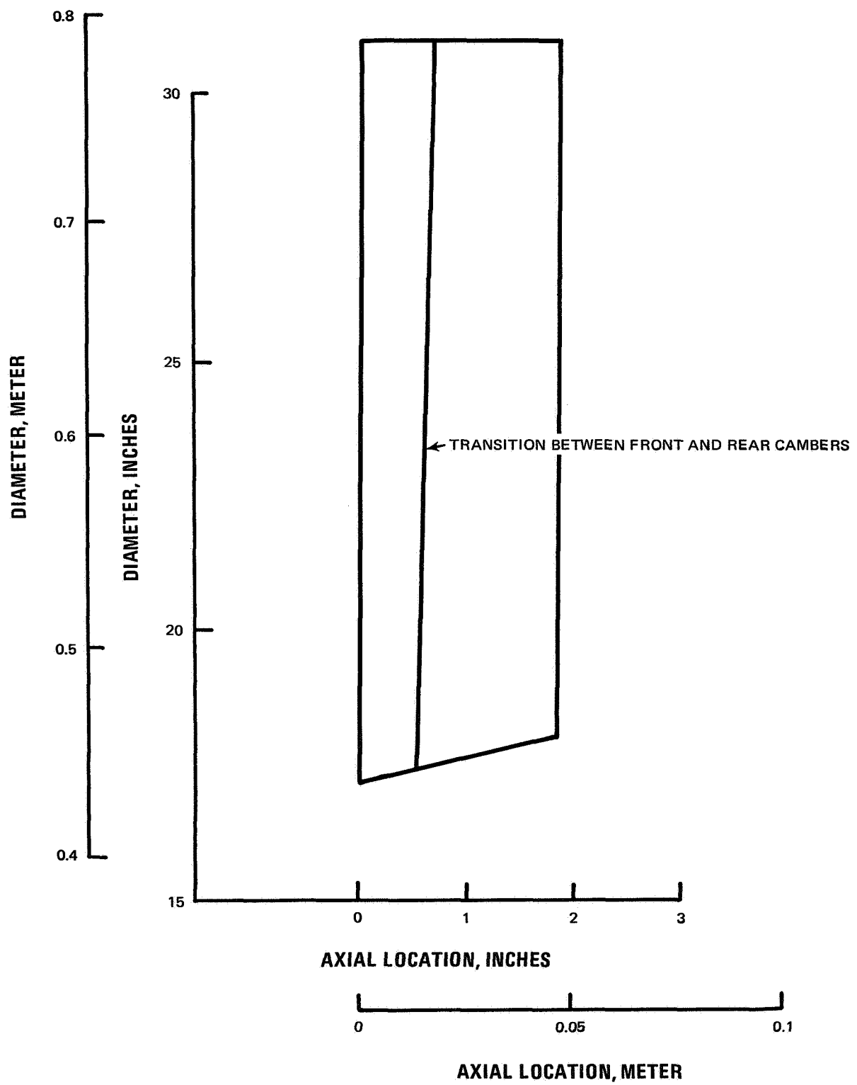
Figure 23 Stator Axial Projection
