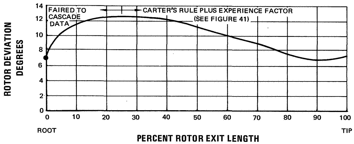
Figure 19 Rotor Spanwise Deviation on Conical Surface
