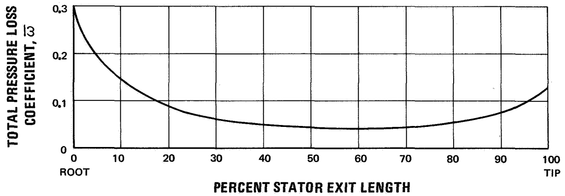
Figure 5 Stator Spanwise Loss
