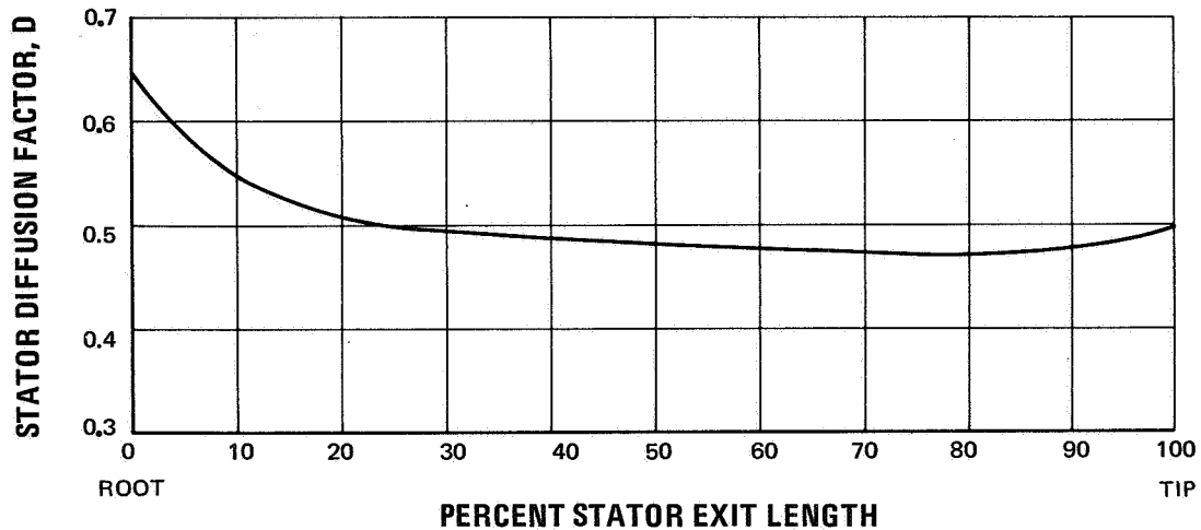
Figure 11 Stator Diffusion Factor
