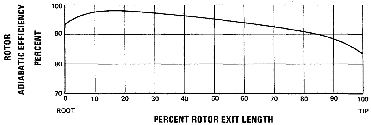
Figure 4 Rotor Spanwise Adiabatic Efficiency
