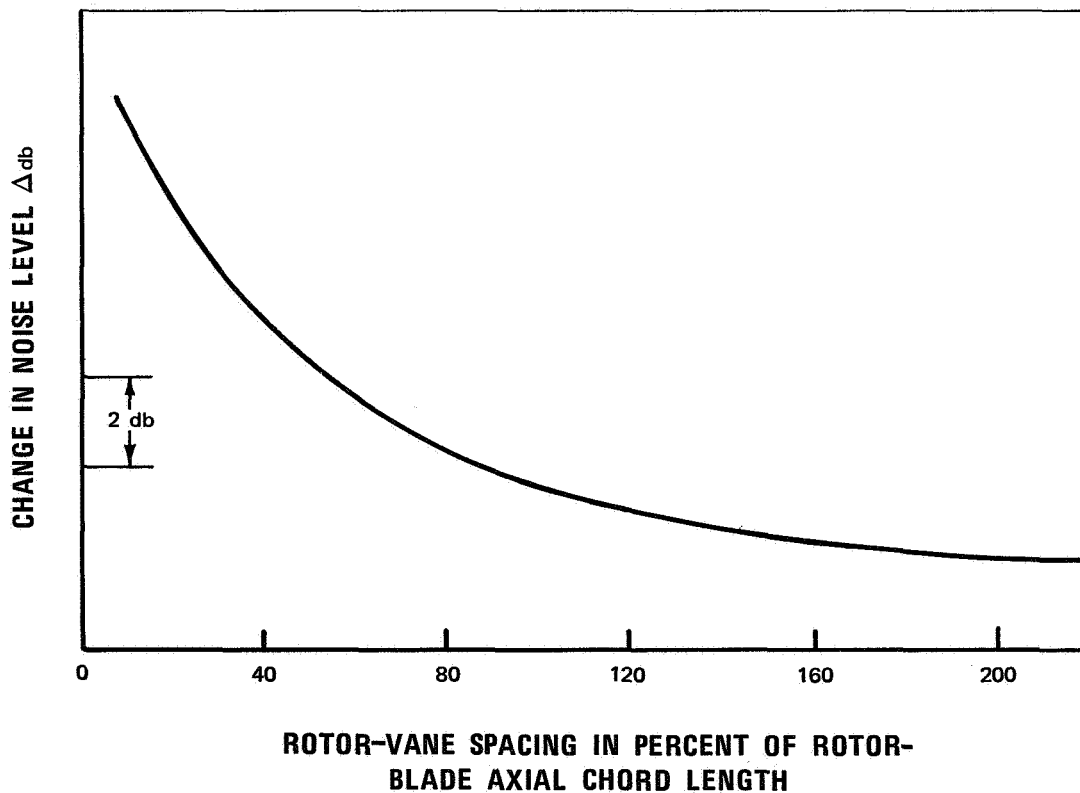
Figure 1 Effect of Rotor-Stator Spacing on Fan Fundamental Blade-Passing Frequency Noise Level
