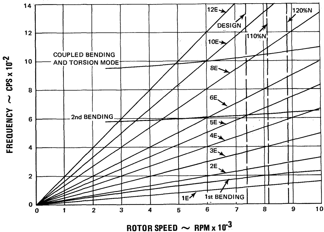
Figure 29 Blade and Disc Resonance Diagram
