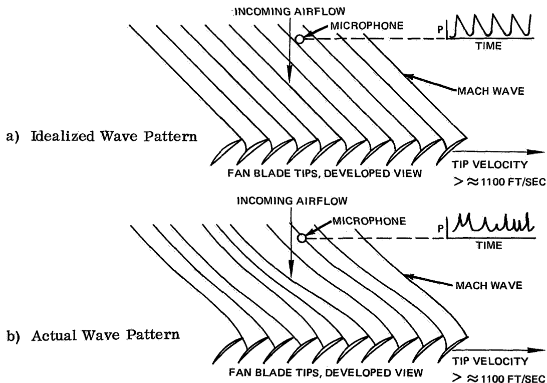
Figure 2 Supersonic Fan Blade Tip Noise
