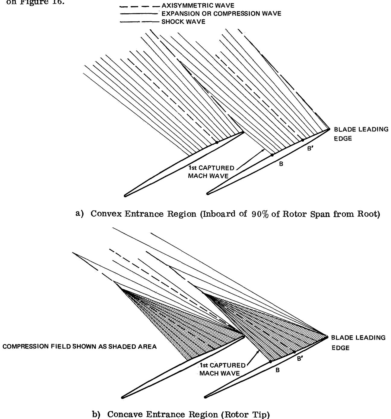
Figure 39 Wave Pattern for Super-Critical Operation of Curved-Blade Entrance Regions
