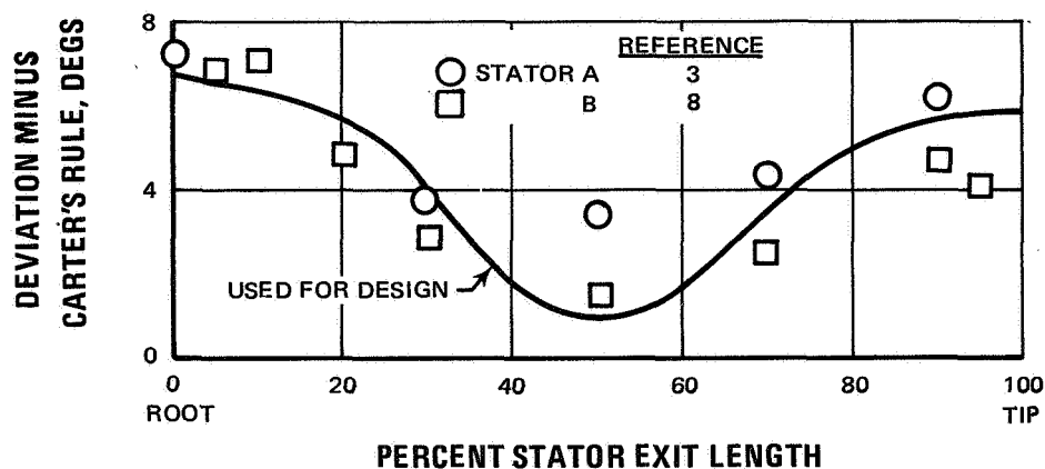
Figure 43 Modification to Carter's Rule Deviation Used for Stator
