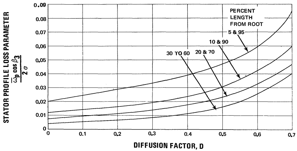
Figure 36 Stator Profile Loss Parameter as Function of Diffusion Factor
