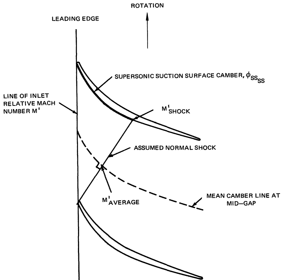
Figure 34 Location of Assumed Normal Shock for Loss Model
