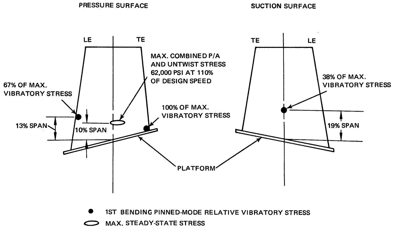
Figure 30 Maximum Combined P/A and Untwist, and Relative Vibratory Stresses
