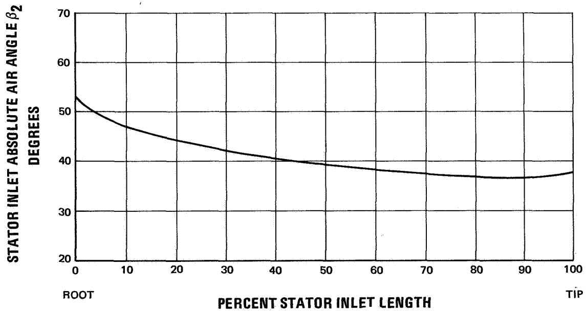
Figure 10 Stator-Inlet Absolute Air Angle Profile
