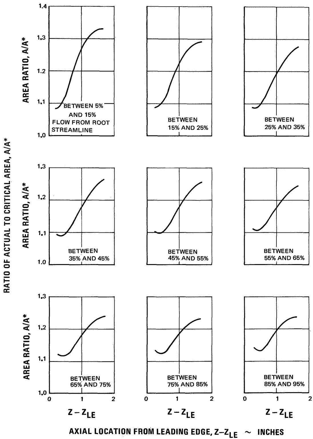
Figure 24 Stator A/A^* Profile
