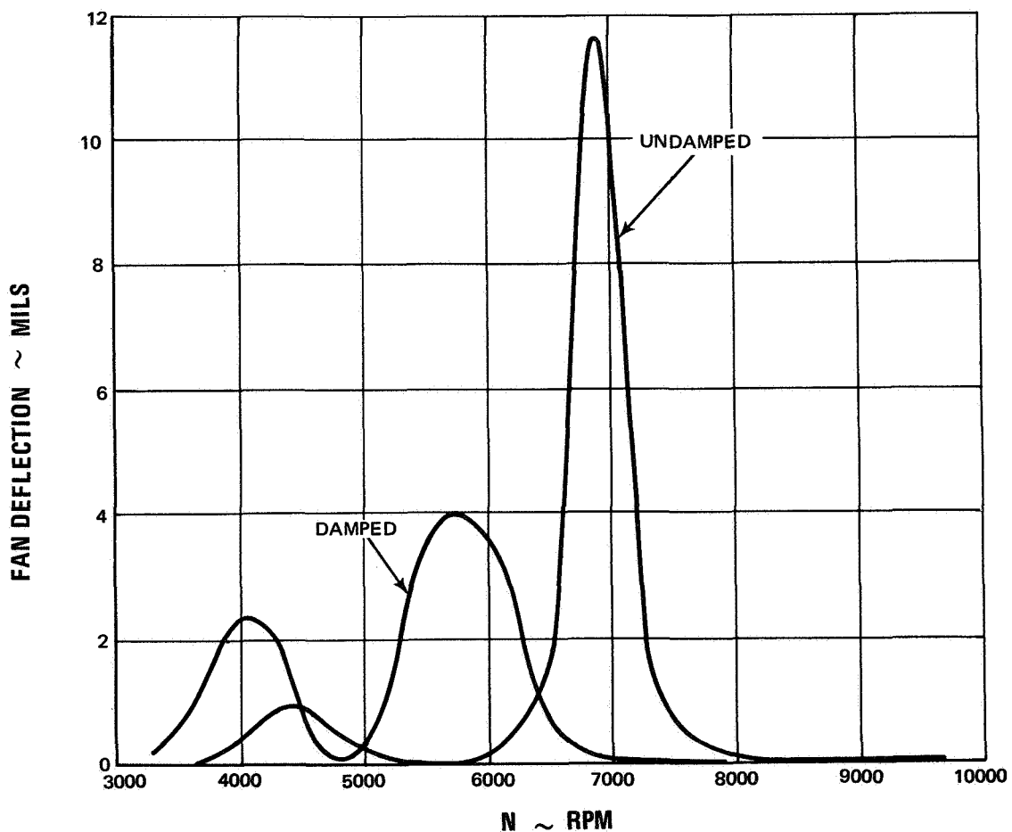
Figure 32 Fan Rig Vibration Amplitude with 1 1/2 oz-in. Unbalance in Fan
