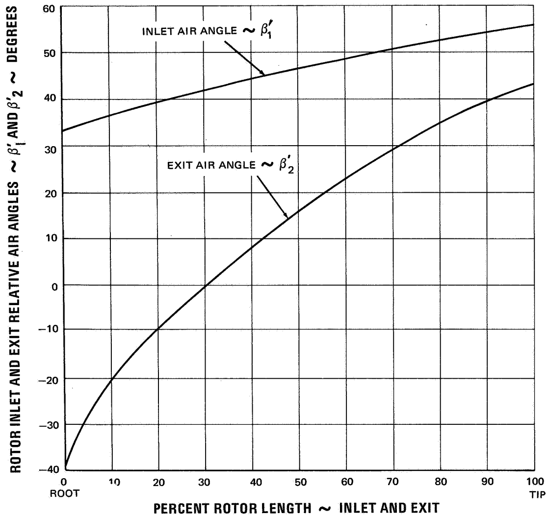
Figure 7 Rotor Inlet and Exit Relative Air Angle Profiles
