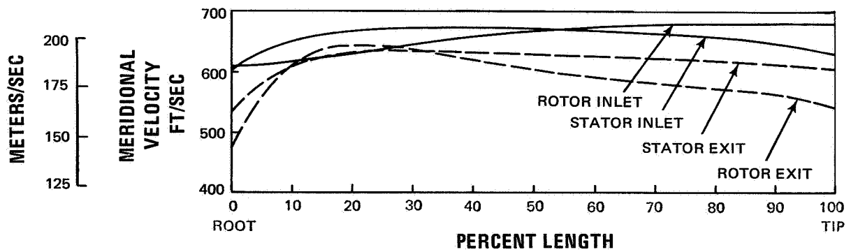
Figure 8 Rotor and Stator Inlet and Exit Velocity Profiles
