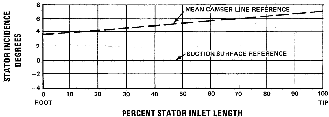
Figure 22 Stator Incidence Referenced to Mean Camber Line and Suction Surface at Leading Edge
