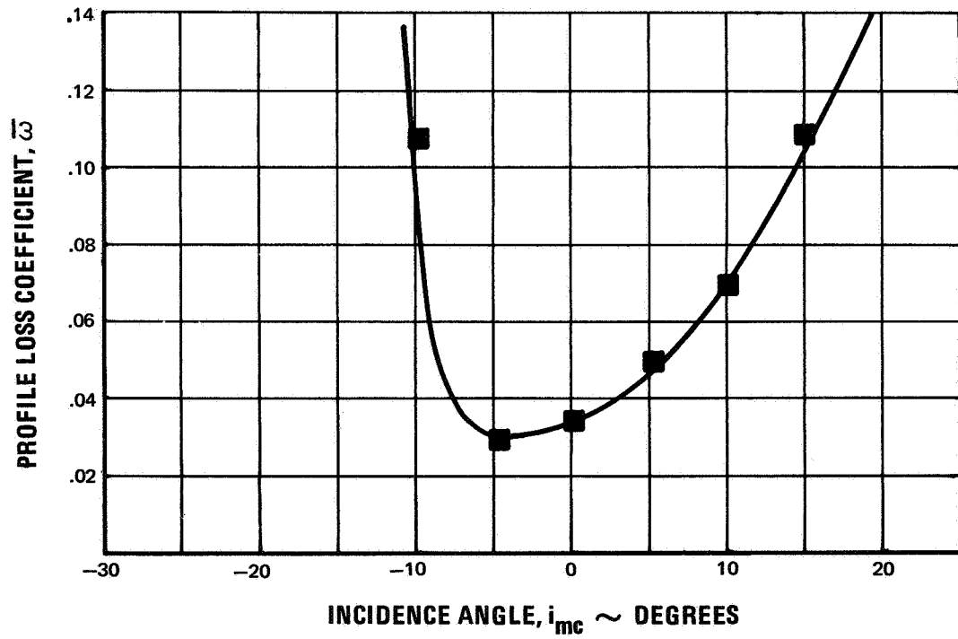
Figure 17 Two-Dimensional Cascade Data
