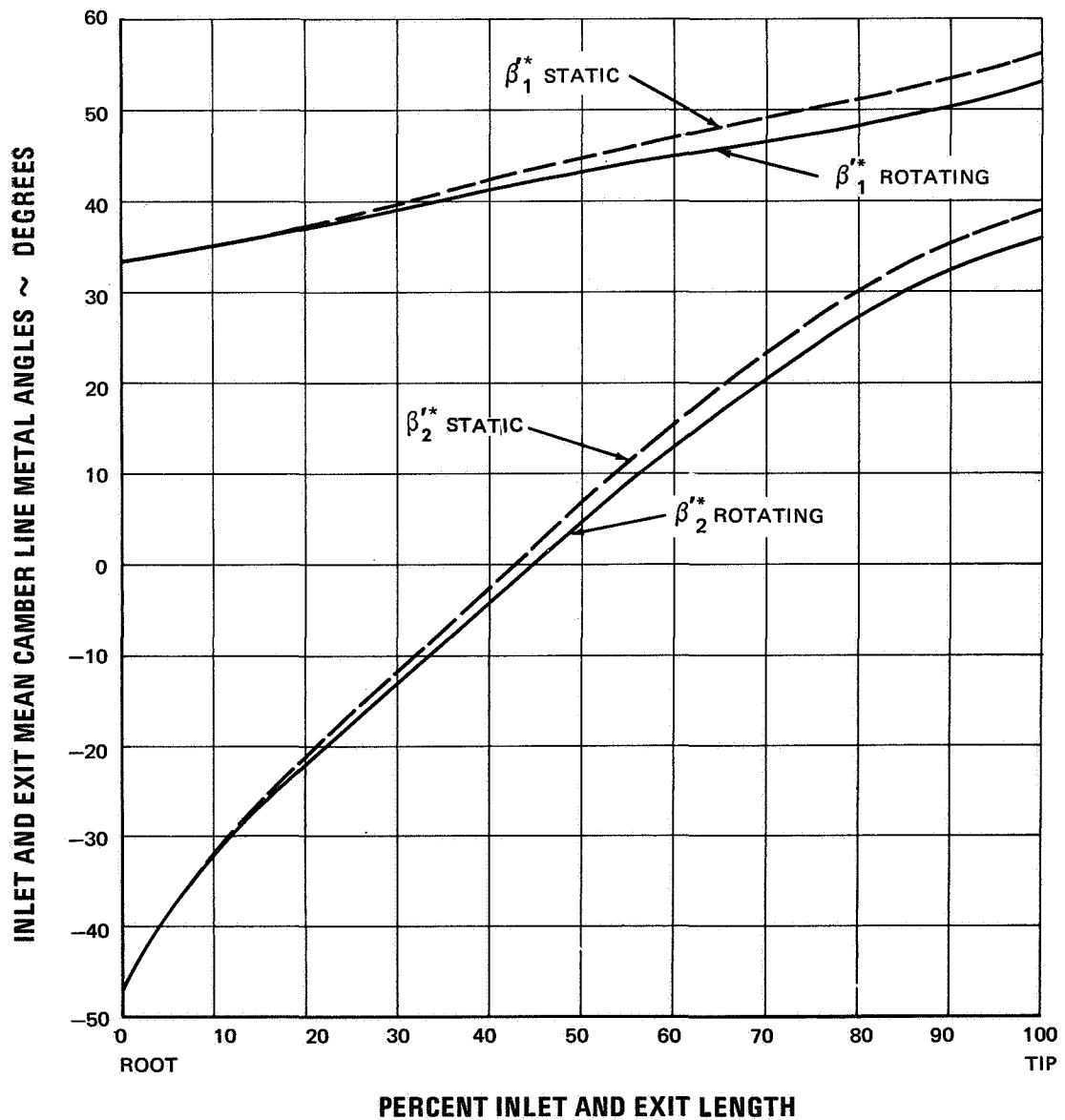
Figure 20 Rotor Spanwise Variation of Inlet and Exit Mean Camber Line Metal Angles on Conical Surface Including Untwist Effect
