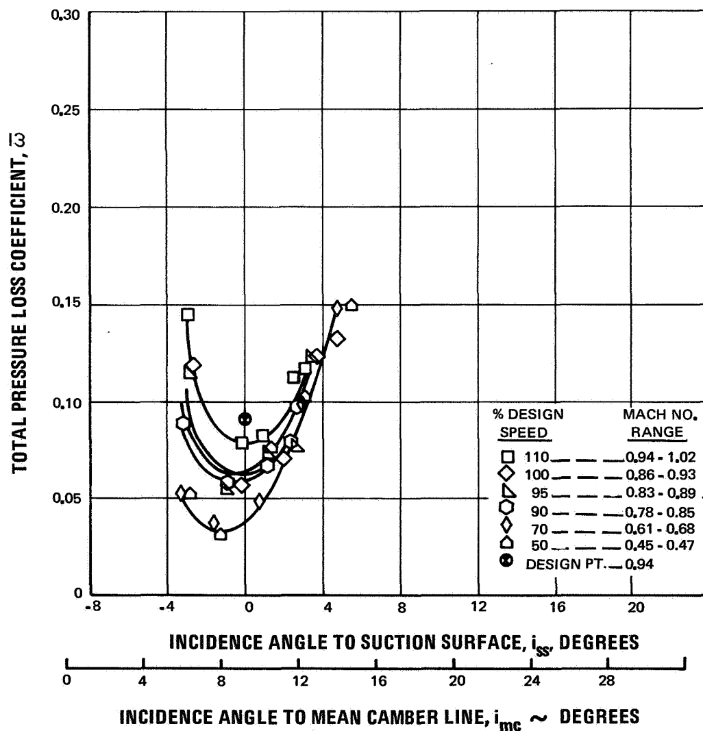
Figure 38 Typical Stator Loss Bucket at 50 Percent Span from Reference 3
