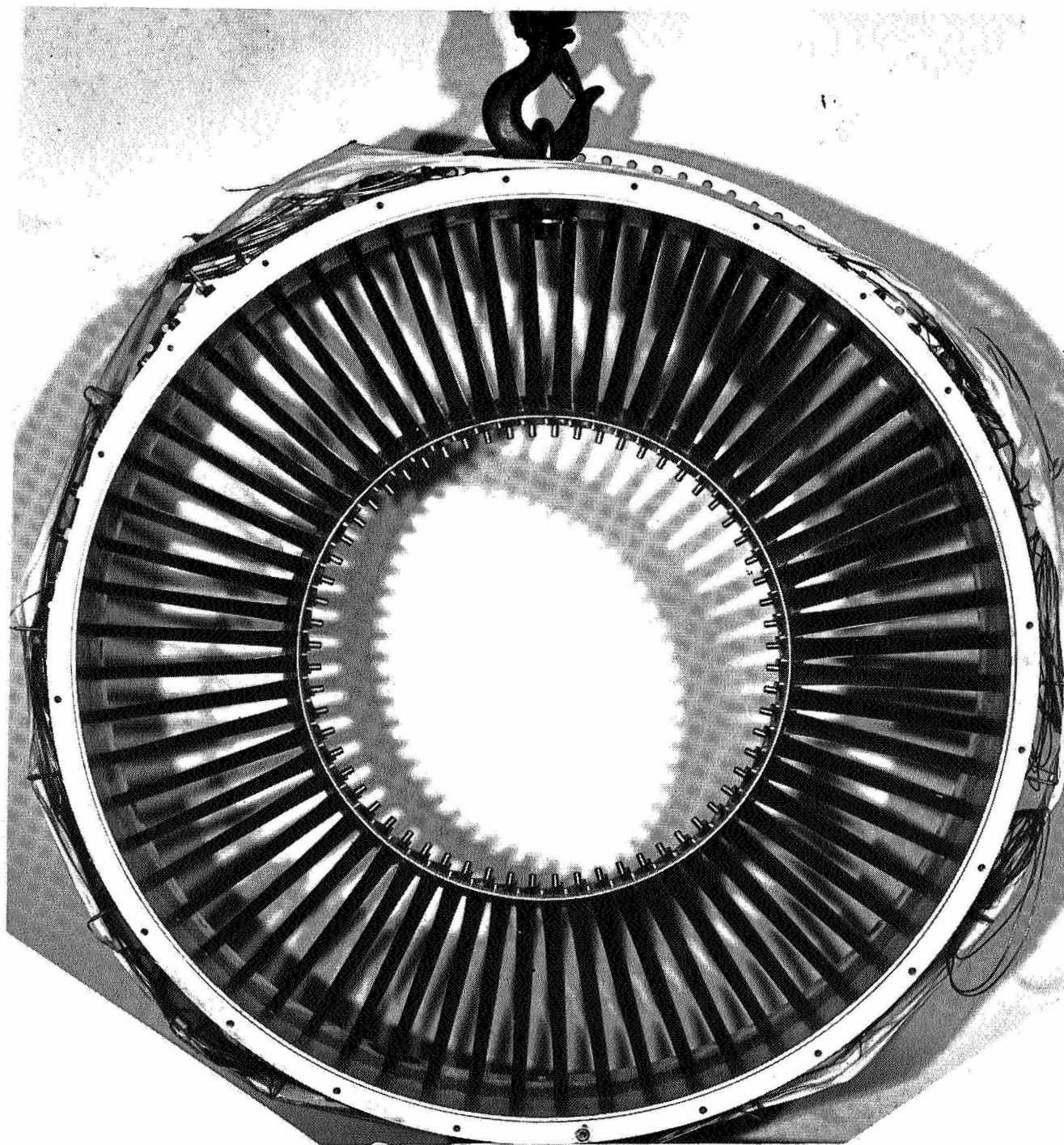
Figure 21 Assembly View of Stator Looking at Stator Leading Edge
