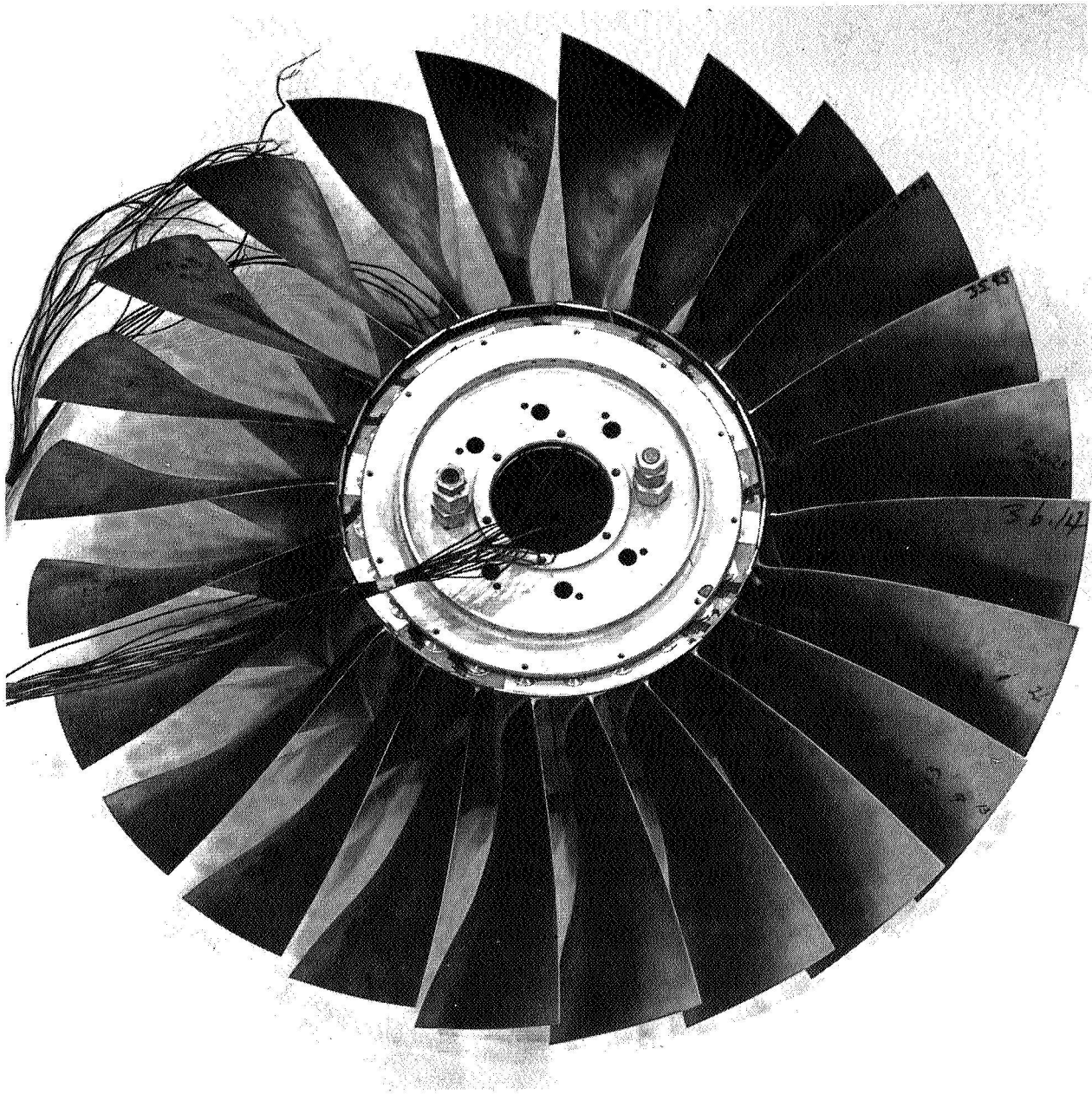
Figure 14 Rotor Assembly Looking into Rotor in Flow Direction
