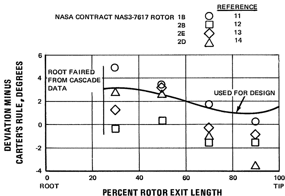
Figure 42 Modification to Carter's Rule Deviation Used for Rotor
