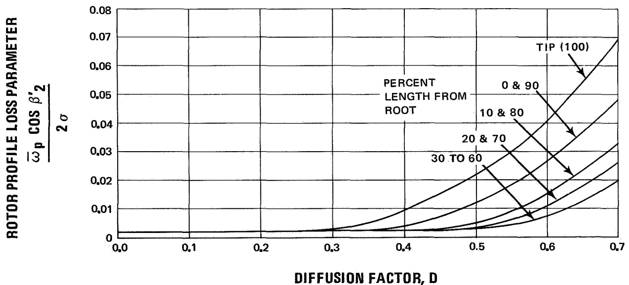
Figure 35 Rotor Profile Loss Parameter as Function of Diffusion Factor
