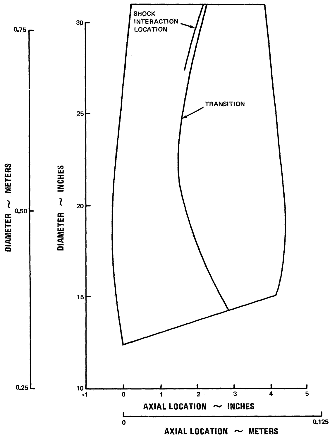
Figure 15 Rotor Axial Projection
