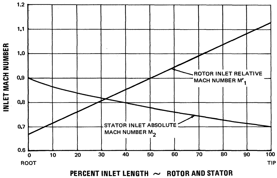
Figure 9 Rotor and Stator Inlet Mach Number Profiles
