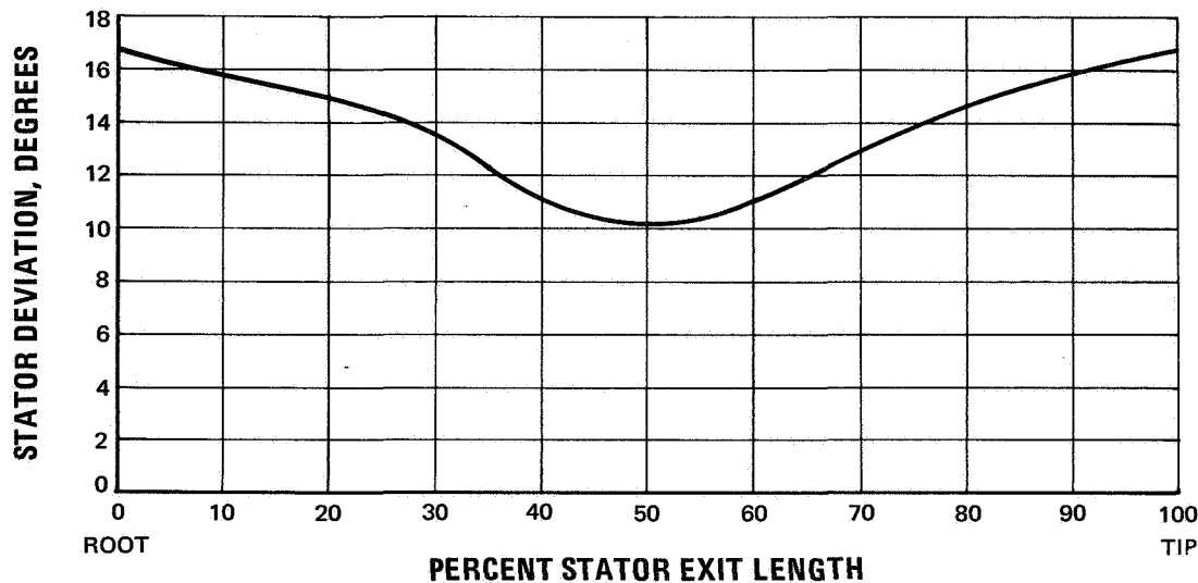
Figure 25 Stator Spanwise Deviation on Conical Surface
