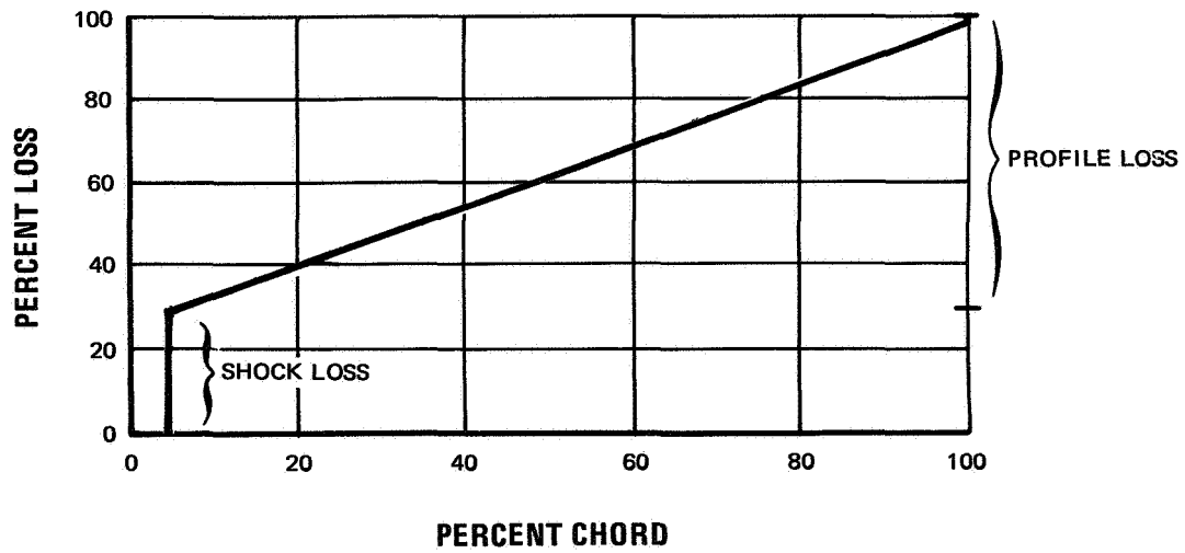
Figure 41 Loss Distribution through Channel
