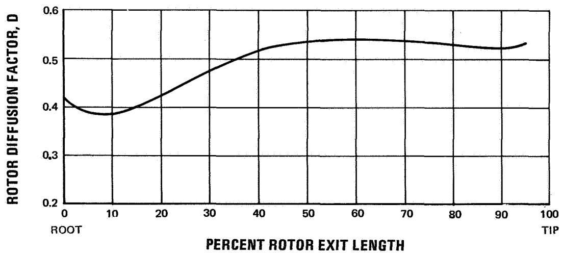
Figure 6 Rotor Diffusion Factor
