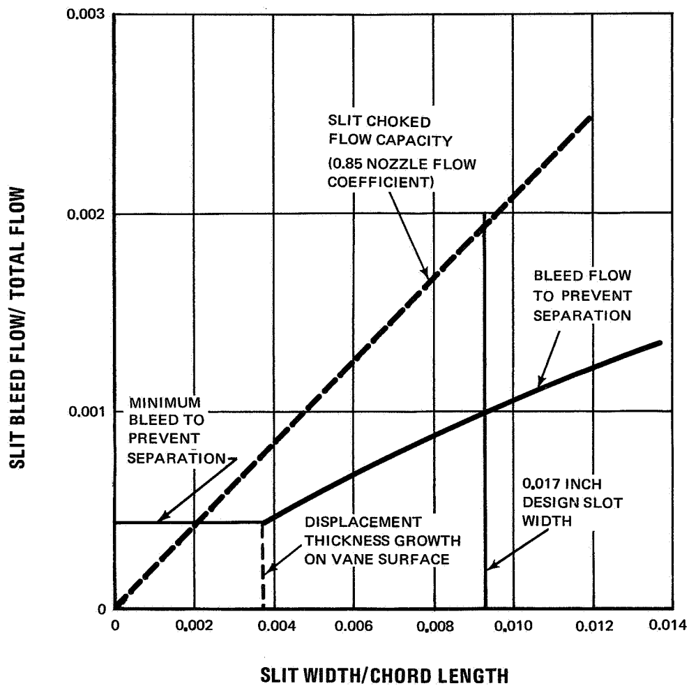
Figure 27 Calculated Minimum Bleed Flow Requirements to Prevent Corner Separation at Root of Stator with Aspect Ratio of 3.67 and Root Solidity of 2.169
