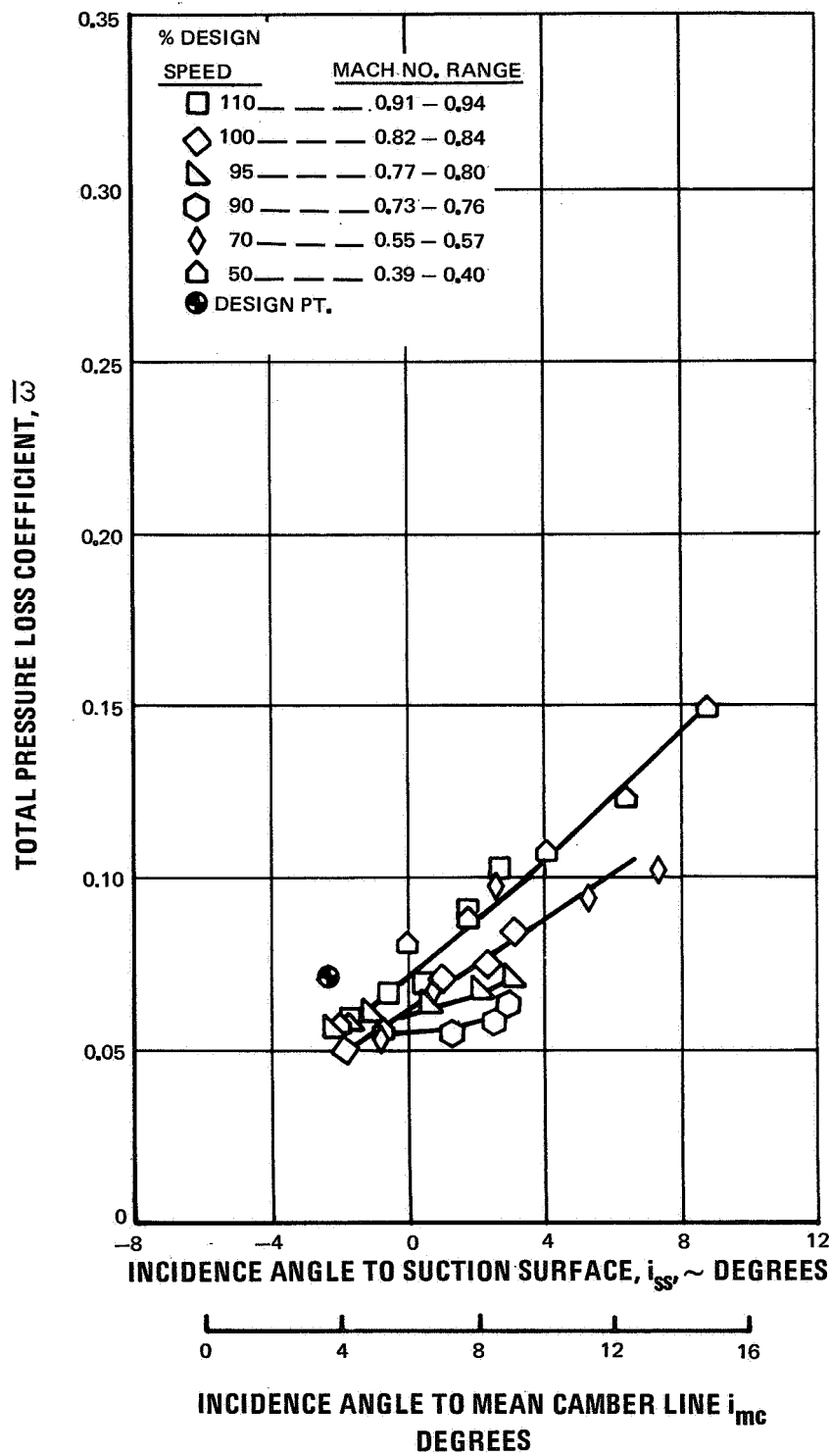
Figure 37 Typical Rotor Loss Bucket at 50 Percent Span from Reference 3.
