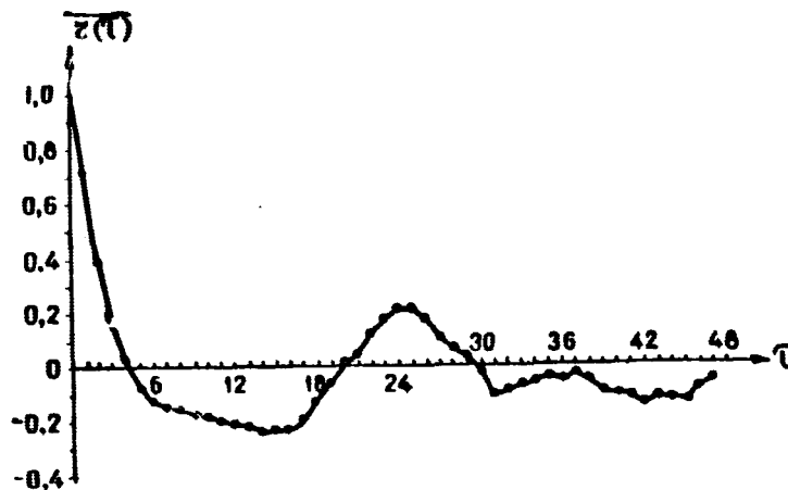
Fig. 4. The dependence of the auto-correlation function of a random component upon the \tau interval, expressed in hours.
