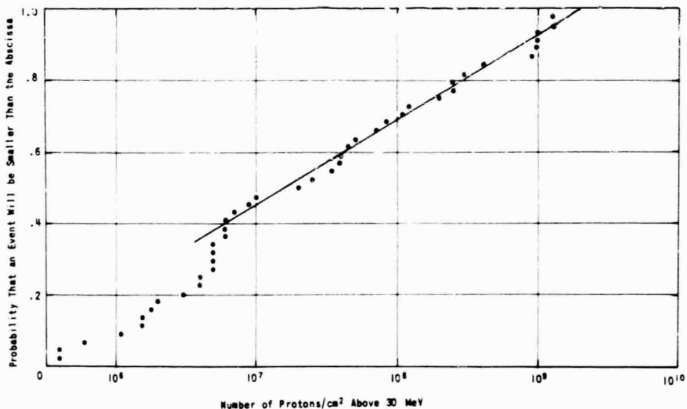
FIGURE ID4 - SIZE DISTRIBUTION OF SOLAR PARTICLE EVENTS OF THE 19TH SOLAR CYCLE IN TERMS OF \log N (> 30 \text{ MeV}) VS PROBABILITY THAT AN EVENT WILL BE LESS THAN THE ABSCISSA
