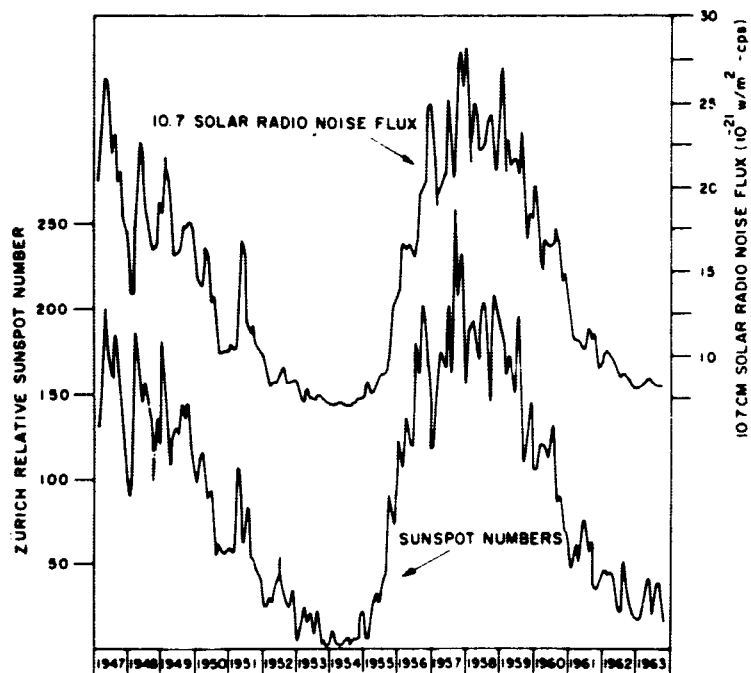
FIGURE 1A7 - UPPER CURVE: MONTHLY MEANS OF 10.7-CM SOLAR RADIO-NOISE FLUX RECORDED BY COVINGTON AT NATIONAL RESEARCH COUNCIL, OTTAWA, CANADA (UNITS ARE 10^{-21} WATTS/M 2 -CPS). LOWER CURVE: MONTHLY MEANS OF THE ZURICH RELATIVE SUNSPOT NUMBERS FROM 1947 TO 1963 (FROM JOHNSON, 1965)
