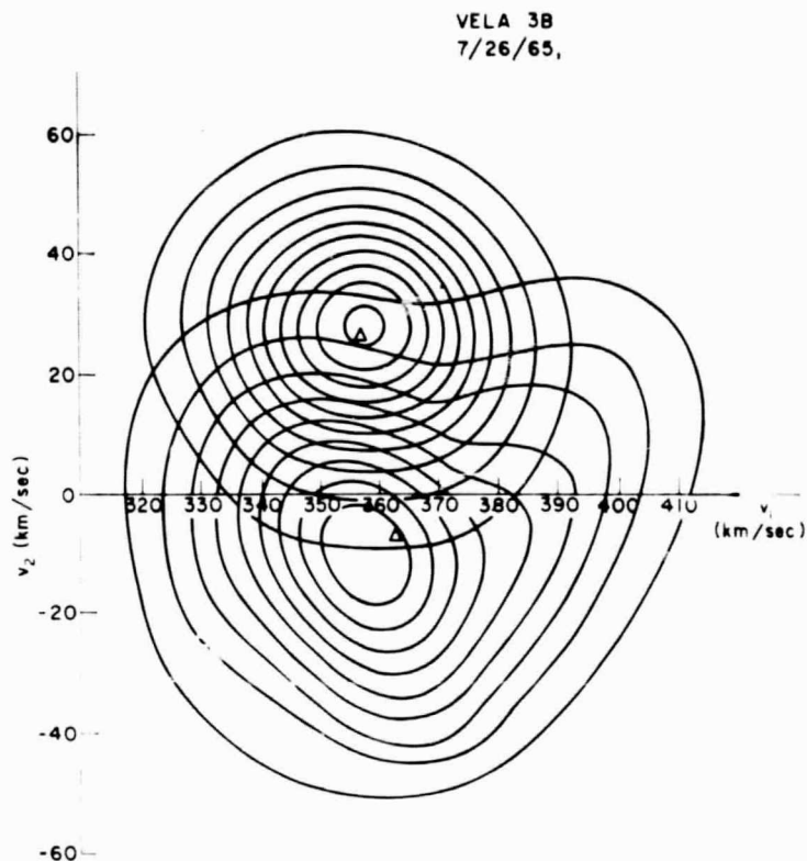
FIGURE IC2 - PROTON VELOCITY CONTOUR MAPPINGS. UPPER CONTOURS - FROM OBSERVATIONS ON VELA 3B ON 7/26/65; LOWER CONTOURS - 8/4/65. THE CONTOURS ARE PROJECTIONS ONTO THE V_1, V_2 PLANE OF CONTOUR LINES FOR f(V_1, V_2) = 1/10, 2/10, \dots TIMES f_{MAX} , WHERE f(V_1, V_2) IS THE TWO-DIMENSIONAL DISTRIBUTION FUNCTION. THE SMALL TRIANGLES INDICATE MEAN VELOCITY. DEVIATION FROM CIRCULAR CONTOURS INDICATES ANISOTROPY (AFTER HUNDHAUSEN ET AL., 1967)
