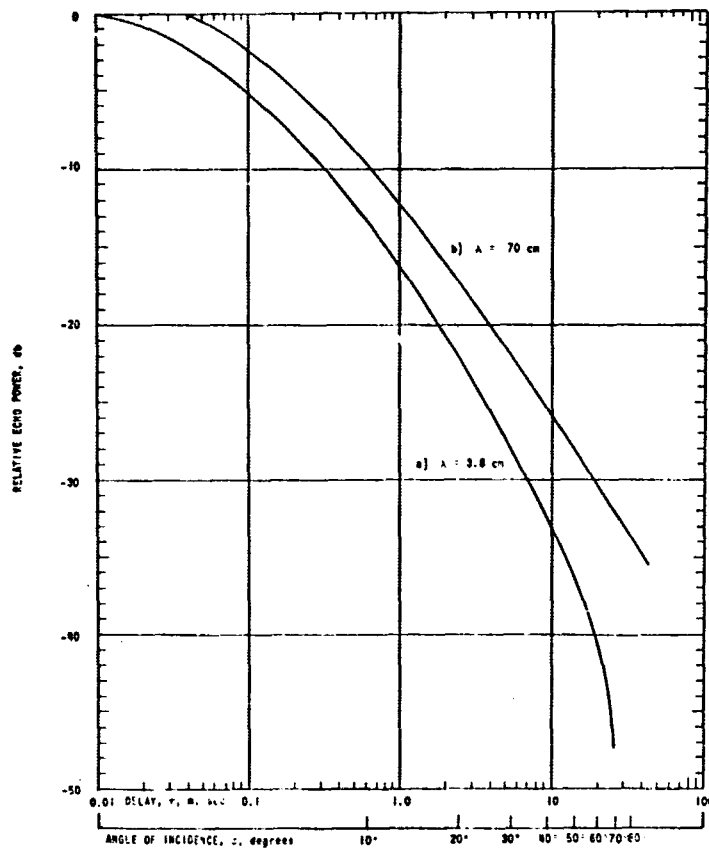
FIGURE IIIB3 - THE MEAN RADAR ANGULAR POWER SPECTRUM OF VENUS AT 3.8 CM AND 70 CM WAVELENGTHS. THE ABCISSA IS LABELLED IN TERMS OF BOTH TIME DELAY AND ANGLE OF INCIDENCE. THE NORMALIZATION OF EACH CURVE IS ARBITRARY (PETTEGILL ET AL., 1967)
