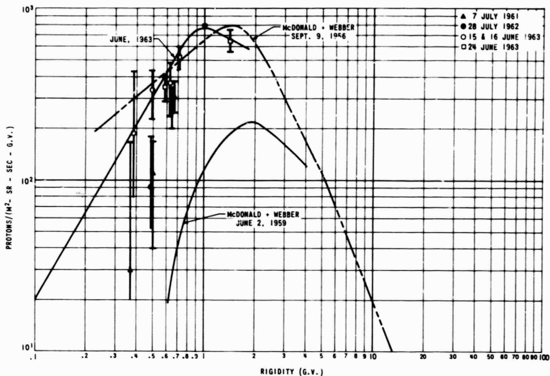
FIGURE 1E1 - GALACTIC COSMIC RAY PROTON DIFFERENTIAL ENERGY SPECTRA AT SOLAR MINIMUM AND MAXIMUM
