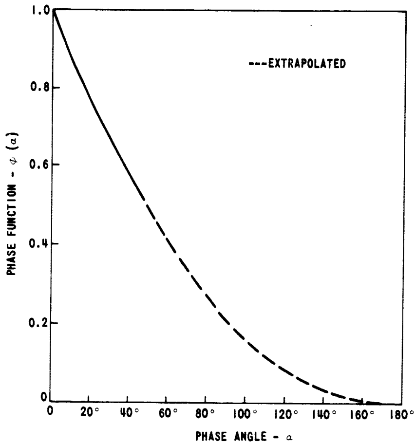
FIGURE 11A3 - VISUAL PHASE FUNCTION OF MARS
