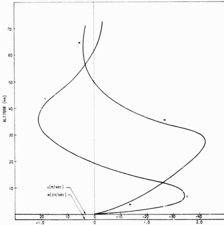
FIGURE IIIC6. - COMPUTED HORIZONTAL AND VERTICAL (U AND W) WIND VELOCITIES FOR VENUS (AFTER OHRING ET AL., 1965).
