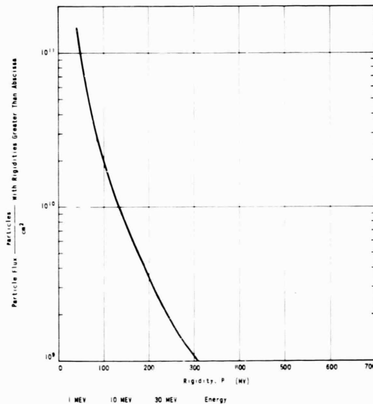
FIGURE ID2 - NEPSAP MODEL SOLAR COSMIC RAY EVENT (FROM NASA SEQ15-001-1, 1965)
