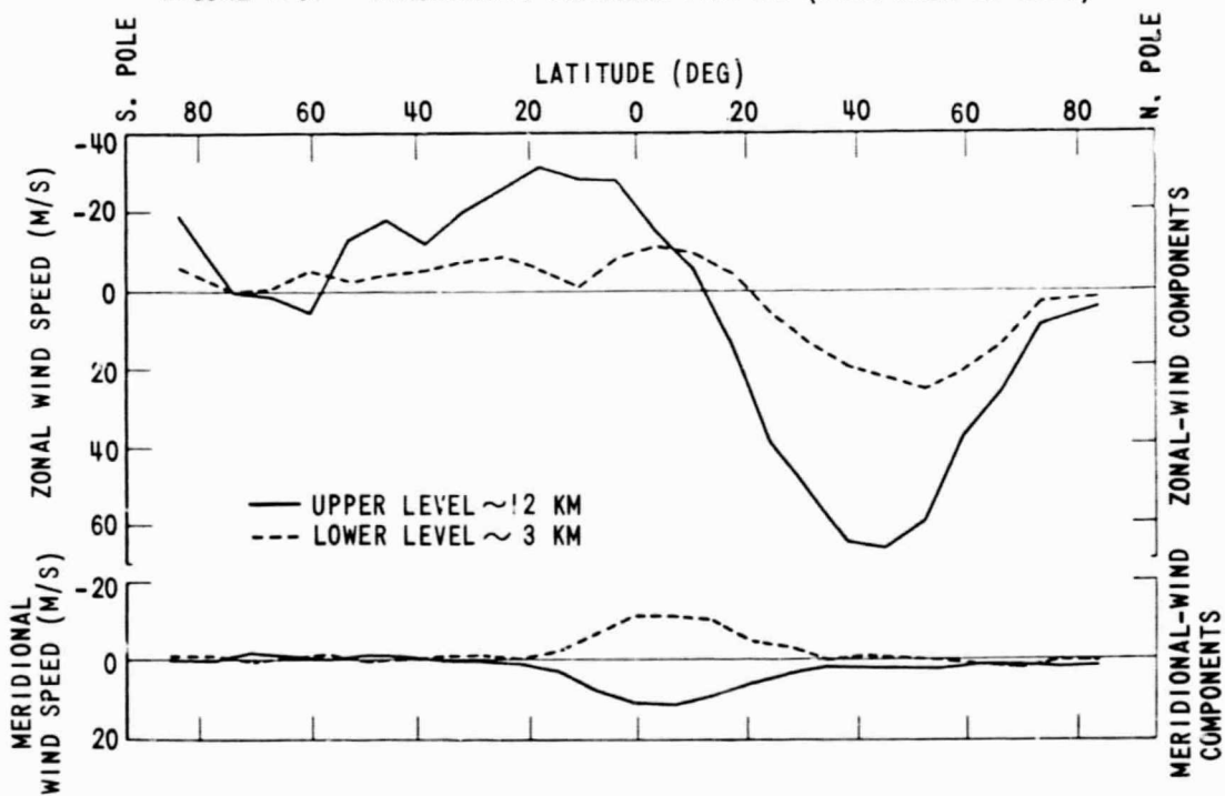
FIGURE 11C4 - MEAN ZONAL AND MERIDIONAL WIND PROFILES FOR MARS. POSITIVE ZONAL WINDS ARE FROM THE WEST; POSITIVE MERIDIONAL WINDS ARE FROM THE SOUTH. (AFTER LEOVY AND MINTZ, 1966)
