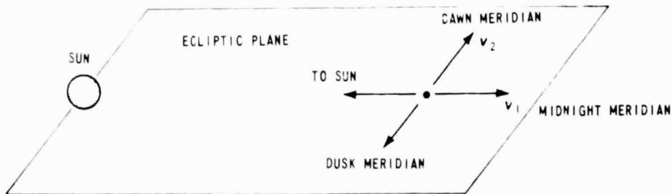
FIGURE IC1 - THE SOLAR ECLIPTIC COORDINATE SYSTEM. V_1 AND V_2 ARE IN THE DIRECTION OF RANDOM VELOCITY COMPONENTS IN THIS SYSTEM
