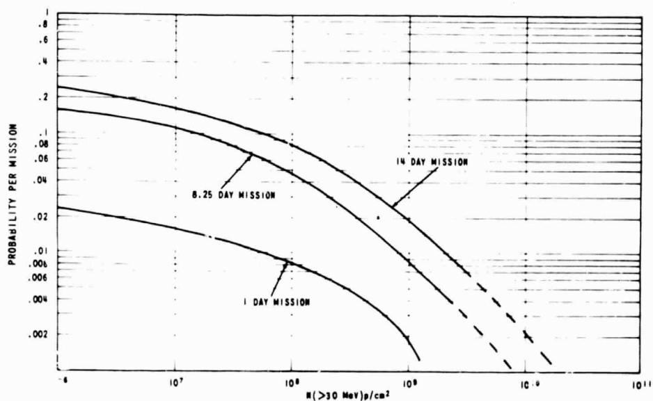
FIGURE ID6 - PROBABILITY PER MISSION OF AN OCCURRENCE OF A SOLAR COSMIC RAY EVENT HAVING AN INTENSITY GREATER THAN N PARTICLES/CM 2 OF ENERGY GREATER THAN 30 MeV
