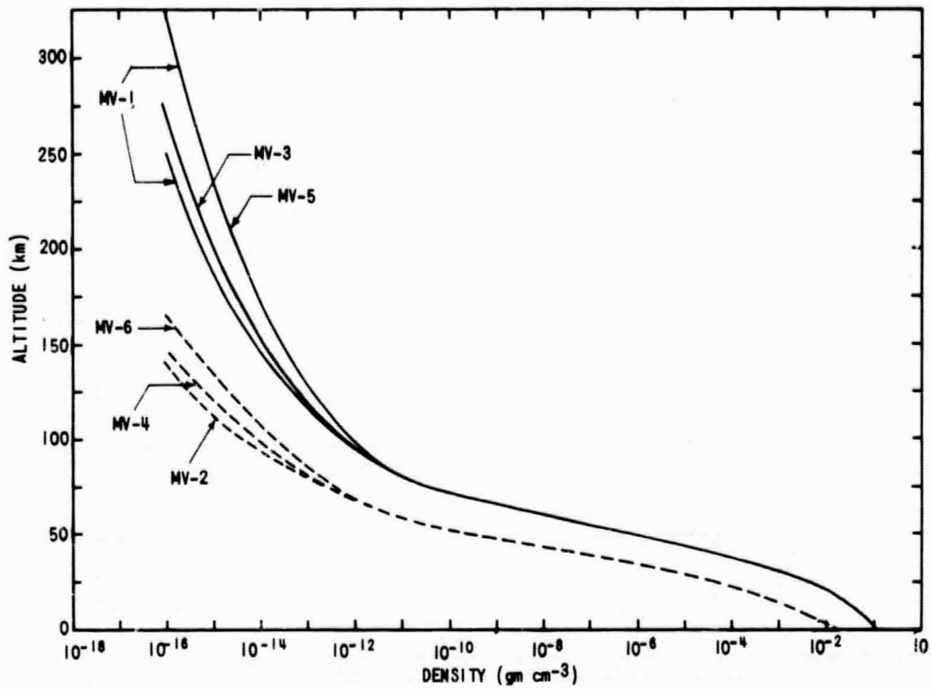
FIGURE IIIC3. - ATMOSPHERIC DENSITY PROFILE OF VENUS (MODELS MV-1 - MV-6 FROM NASA, 1968)
