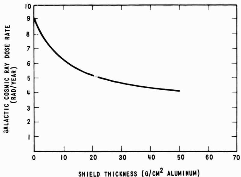
FIGURE 1E2 - DOSES RESULTING FROM GALACTIC COSMIC RAYS AS A FUNCTION OF SHIELD THICKNESS
