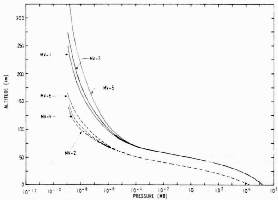
FIGURE IIIC2. - ATMOSPHERIC PRESSURE PROFILE OF VENUS (MODELS MV-1 THROUGH MV-6 FROM NASA, 1968)
