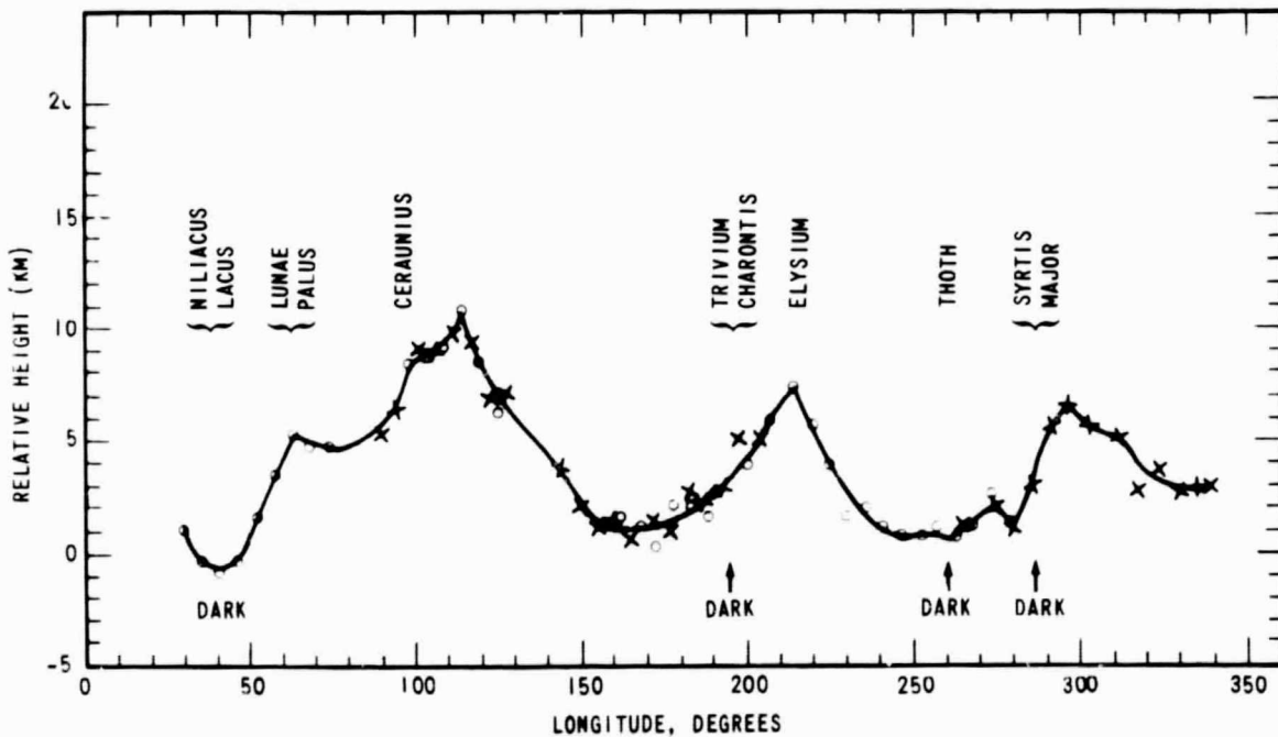
FIGURE IIB4 - MARTIAN HEIGHT PROFILE AT 21^{\circ} N LATITUDE OBTAINED FROM VERTICAL INCIDENCE RADAR RANGING AT 3.8 CM WAVELENGTH. SOME SURFACE FEATURES AND OPTICALLY DARK REGIONS AT 21^{\circ} N ARE LISTED (AFTER PETTENGILL, 1967)
