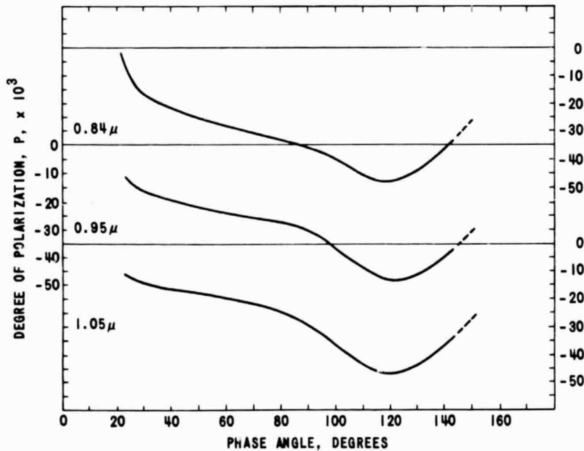
FIGURE IIIA3 - POLARIZATION CURVES OF VENUS IN THE INFRARED 0.8\mu - UPPER RIGHT SCALE; 0.95\mu - LEFT SCALE, 1.05\mu - LOWER RIGHT SCALE. (AFTER DOLLFUS, 1966)
