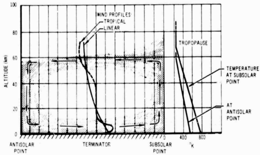
FIGURE IIIC5. - SUGGESTED CIRCULATION IN THE ATMOSPHERE OF VENUS (AFTER KOENIG ET AL., 1967)
