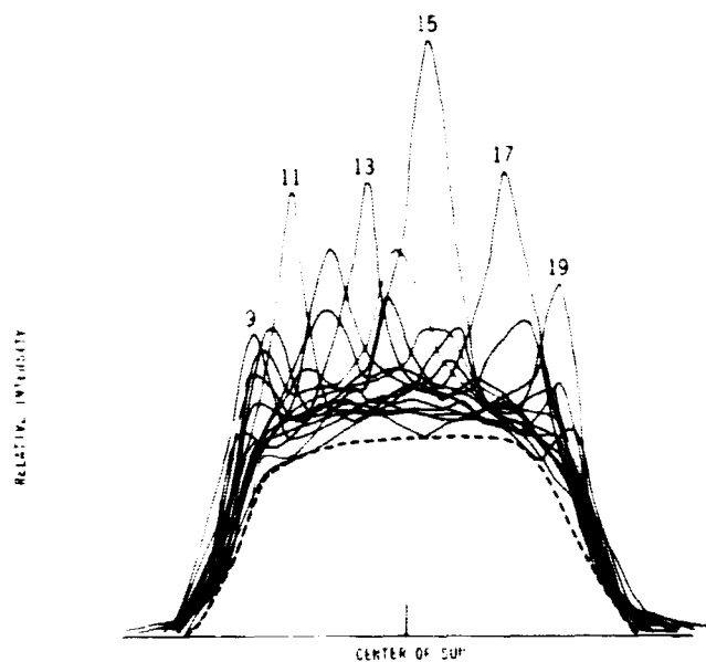
FIGURE 1A8 - MOTION OF ACTIVE CENTERS ACROSS THE DISK OF THE SUN. SUPERPOSITION OF 15 SOLAR INTERFEROGRAMS TAKEN ON 3 CM AT 2-DAY INTERVALS AT NAMCAY (FROM STEINBERG AND LEQUEUX, 1963)
