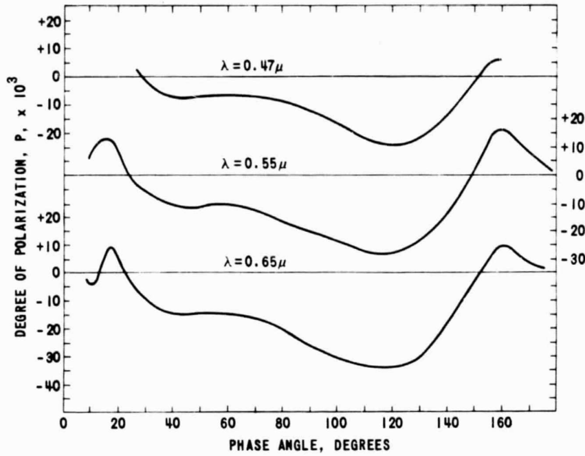
FIGURE IIIA2 - VISUAL POLARIZATION CURVES OF VENUS .47\mu - UPPER LEFT SCALE, .55\mu - RIGHT SCALE, .65\mu - LOWER LEFT SCALE. OBSERVATIONS REFER TO A REGION NEAR THE EQUATOR, MIDWAY BETWEEN LIMB AND TERMINATOR (AFTER DOLLFUS, 1966)
