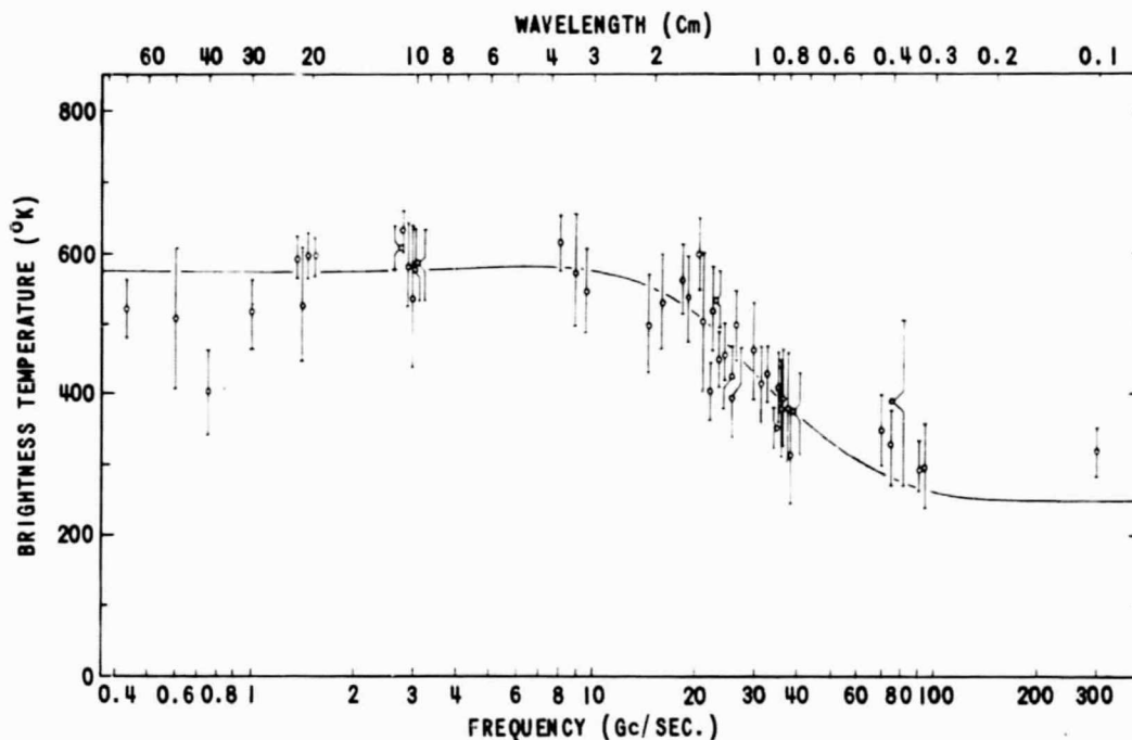
FIGURE 111A5 - THE OBSERVED MICROWAVE BRIGHTNESS TEMPERATURE OF VENUS (AFTER HO ET AL., 1966)
