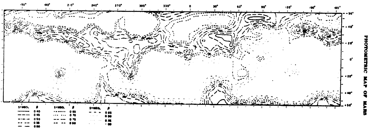
FIGURE 11A4 - CONTOUR MAP OF EQUAL RELATIVE BRIGHTNESS \beta FOR THE PLANET MARS. THE MAP WAS MADE AT A RESOLUTION OF ABOUT 600 KM (APPROX. 10°)
