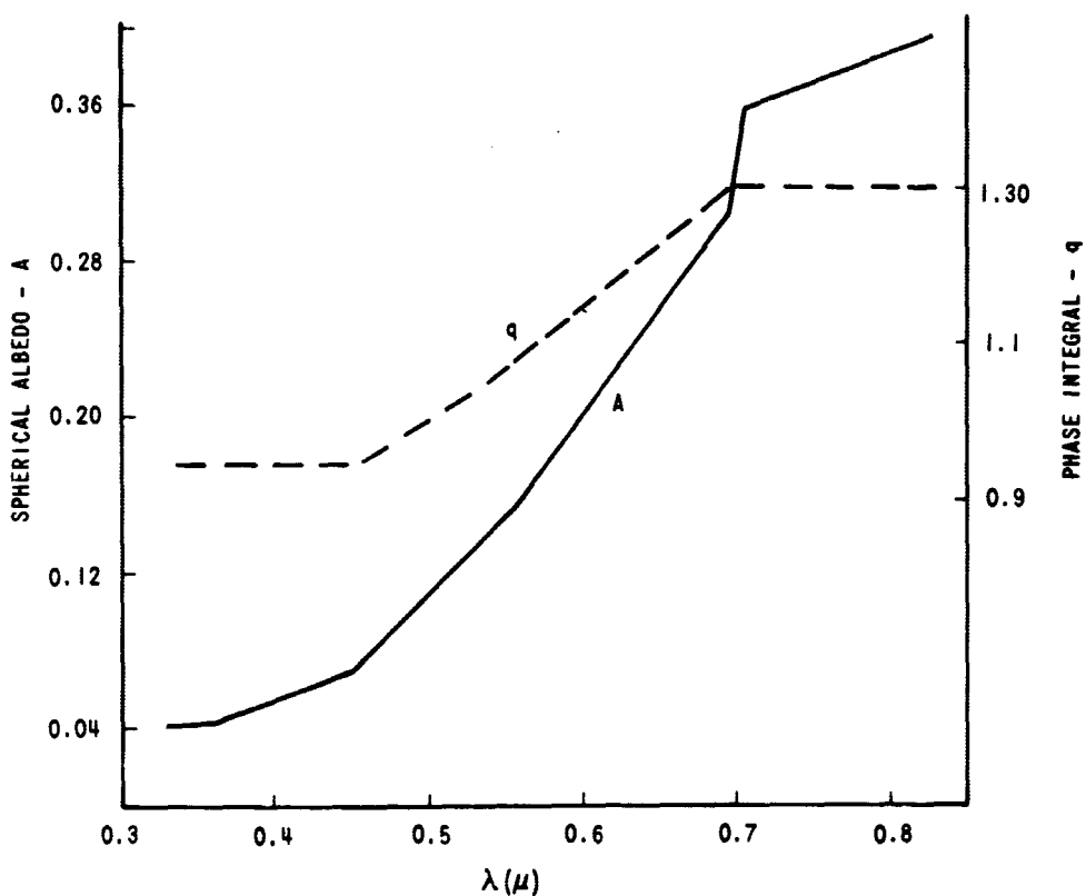
FIGURE IIA2 - SPECTRAL VARIATION OF PHASE INTEGRAL q AND SPHERICAL ALBEDO A (AFTER DE VAUCOULEURS)
