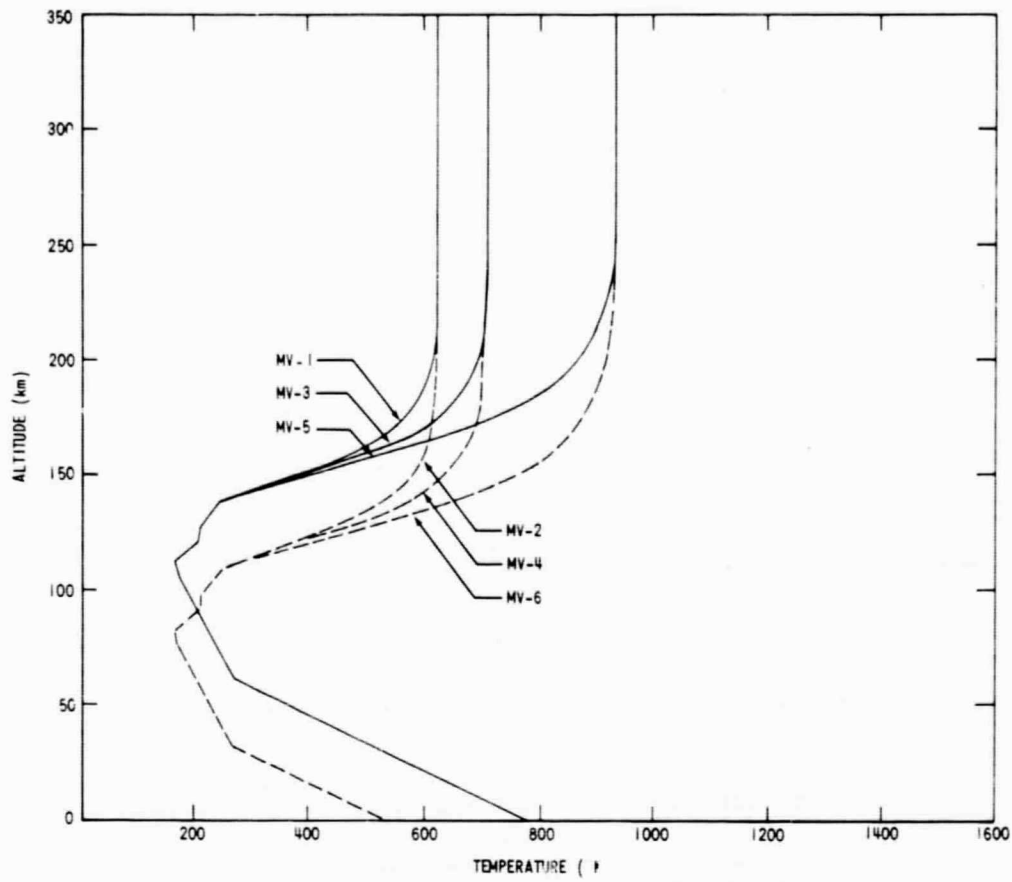
FIGURE IIIC1. - ATMOSPHERIC TEMPERATURE PROFILE OF VENUS (AFTER NASA, 1968)
