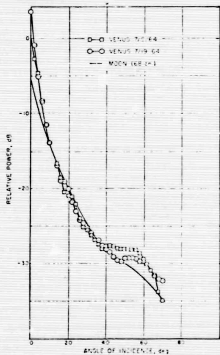
FIGURE 11IB2 - P(\phi) , BACKSCATTERING FUNCTION OF VENUS, COMPUTED FROM SPECTRA AS SHOWN IN FIGURE 11IB1. THE SMOOTH CURVE IS FOR THE MOON ALL THREE CURVES HAVE BEEN SHIFTED TO MATCH AT 10^\circ .
