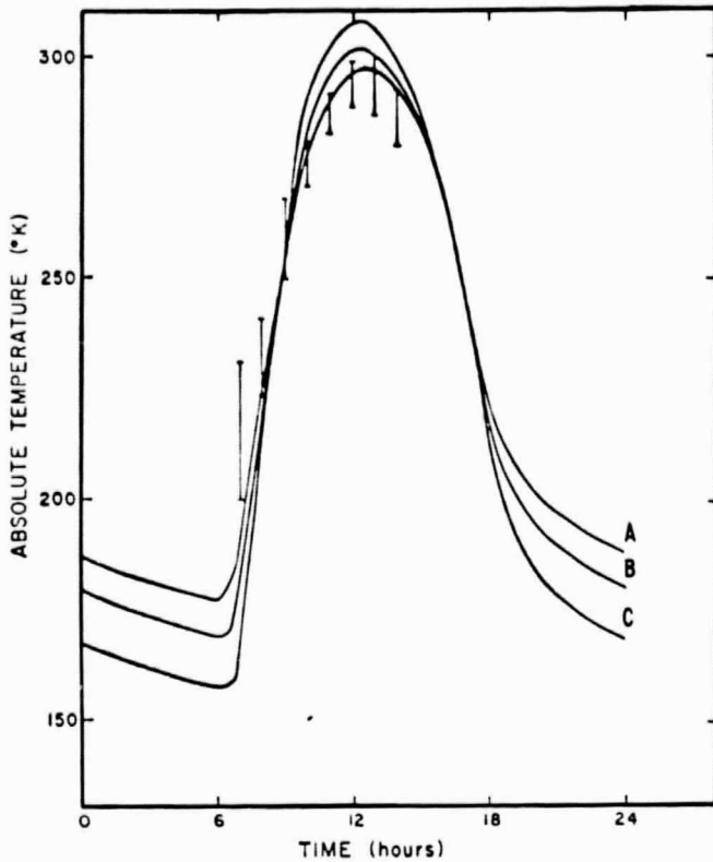
FIGURE IIB3 - DIURNAL VARIATION OF SURFACE TEMPERATURE IN THE EQUATORIAL REGION OF MARS. VERTICAL BARS- SINTON AND STRONG'S OBSERVATIONS. ASSUMED VALUES OF (KPC)^{\frac{1}{2}} : CURVE A-0.0055, CURVE B-0.0042, CURVE C-0.003
