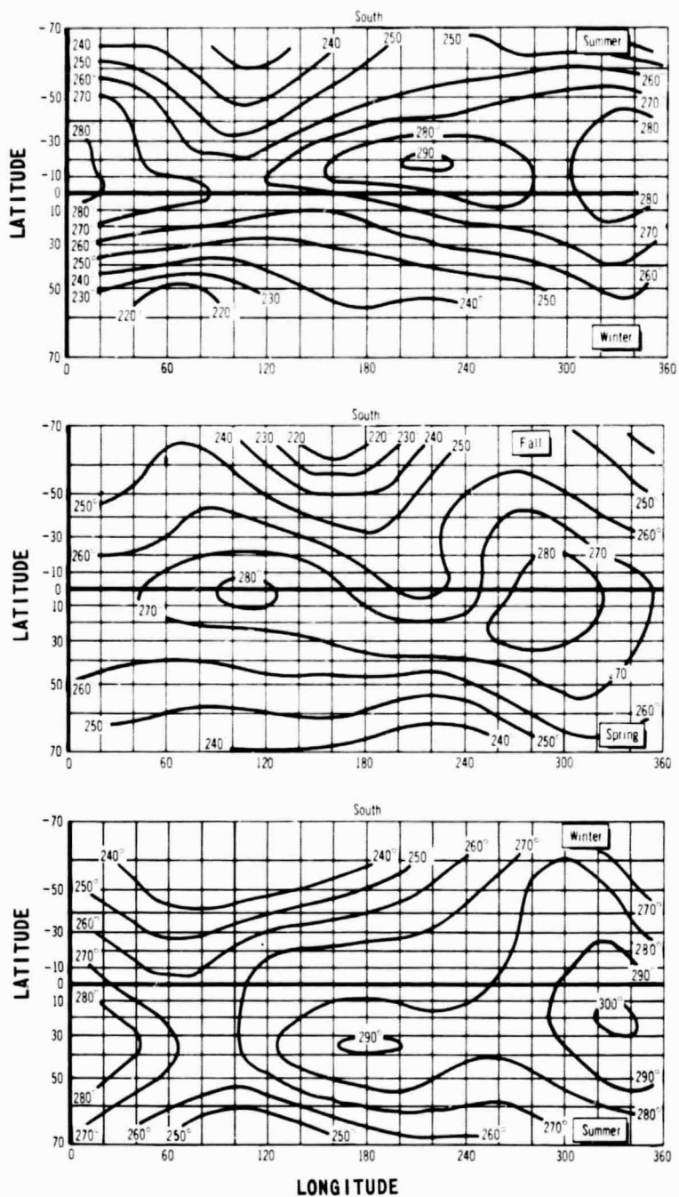
FIGURE IIB2 - AVERAGE MARTIAN ISOOTHERMS. (AFTER GIFFORD, 1952)
