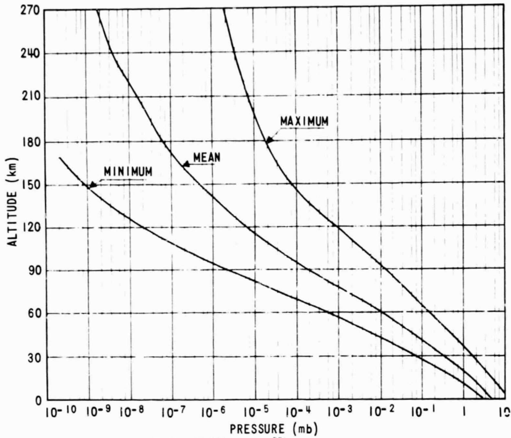
FIGURE 11C3 - ATMOSPHERIC PRESSURE PROFILE (FROM NASA SP-0010)
