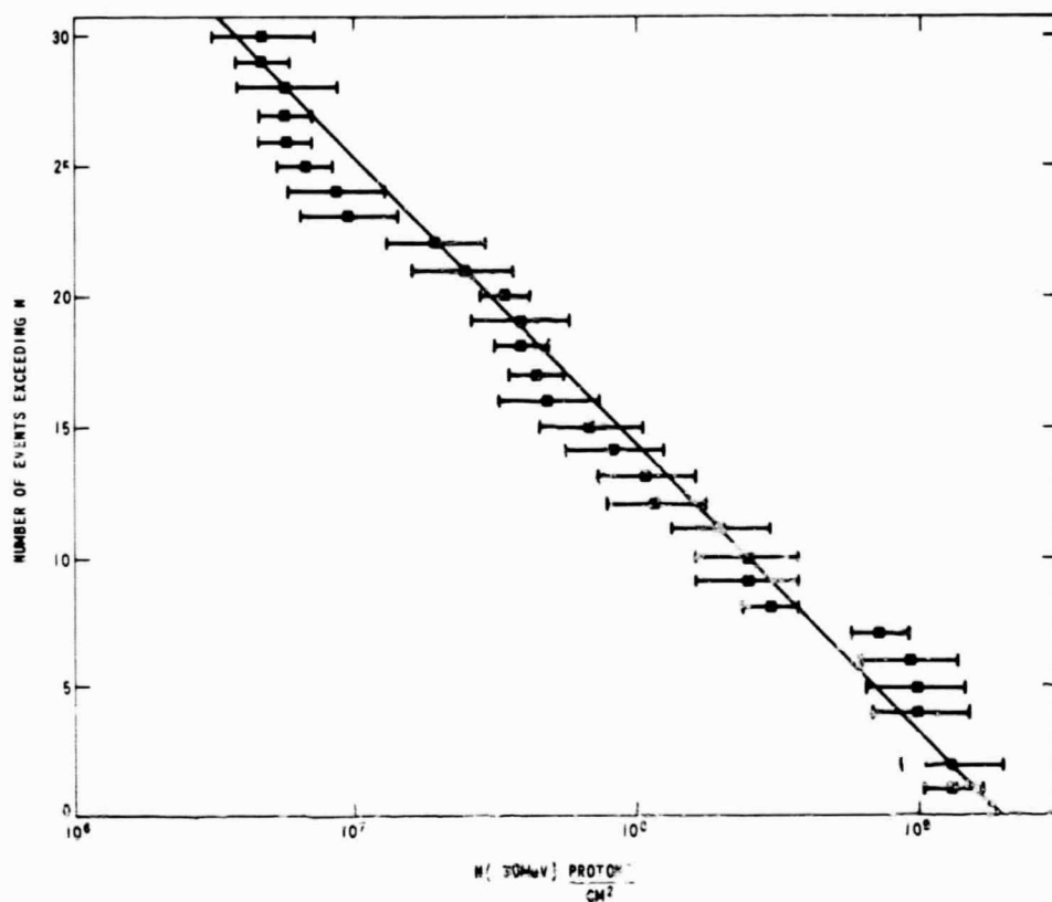
FIGURE ID3 - INTEGRAL FLUX DISTRIBUTION (FROM HILBERG, 1965)
