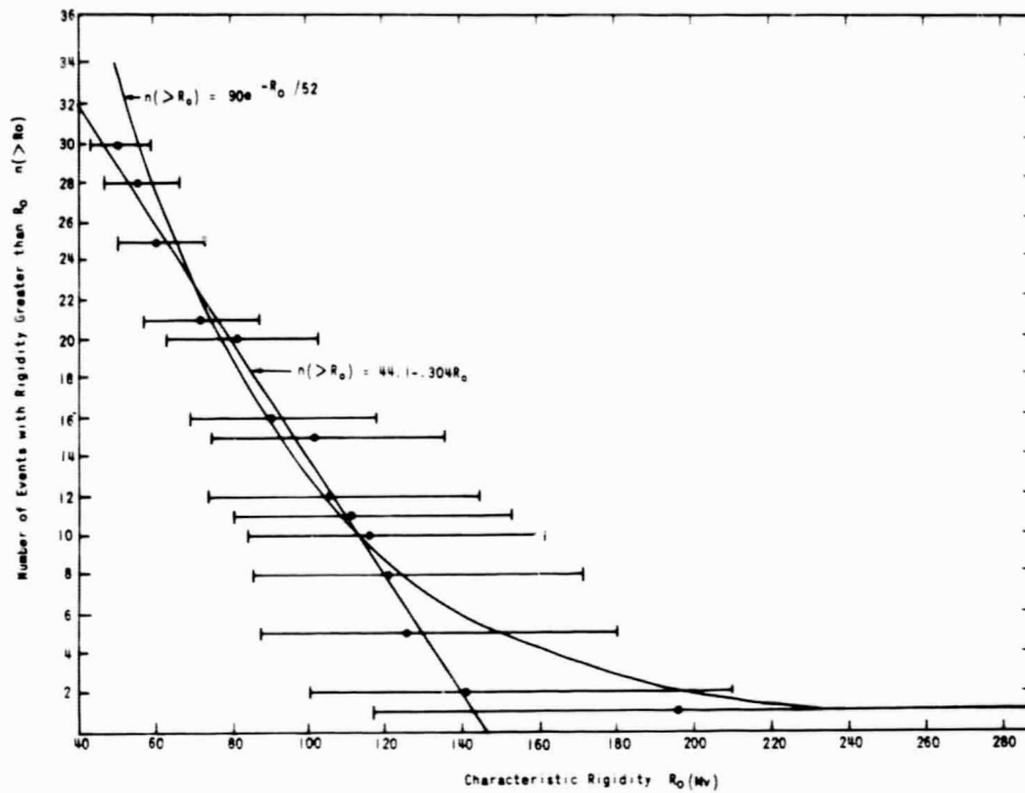
FIGURE ID1 - DISTRIBUTION OF CHARACTERISTIC RIGIDITY (FROM HILBERG, 1965)
