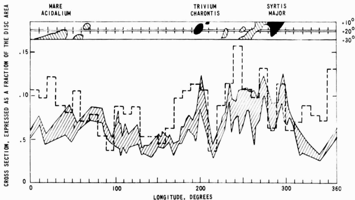
FIGURE IIA6 - VARIATION OF THE RADAR CROSS SECTION OF MARS AT 70 CM (SHADED REGION) AND AT 12.5 CM WAVELENGTH (DOTTED LINE), DURING THE 1965 OPPOSITION, AS A FUNCTION OF THE CENTRAL MERIDIAN OF THE VISIBLE DISC. THE STRIP MAP AT THE TOP OF THE FIGURE SHOWS THE PRINCIPAL OPTICAL FEATURES OF MARS NEAR THE SUB-RADAR LATITUDE OF 20°N (AFTER PETTENGILL AND EVANS, 1967)
