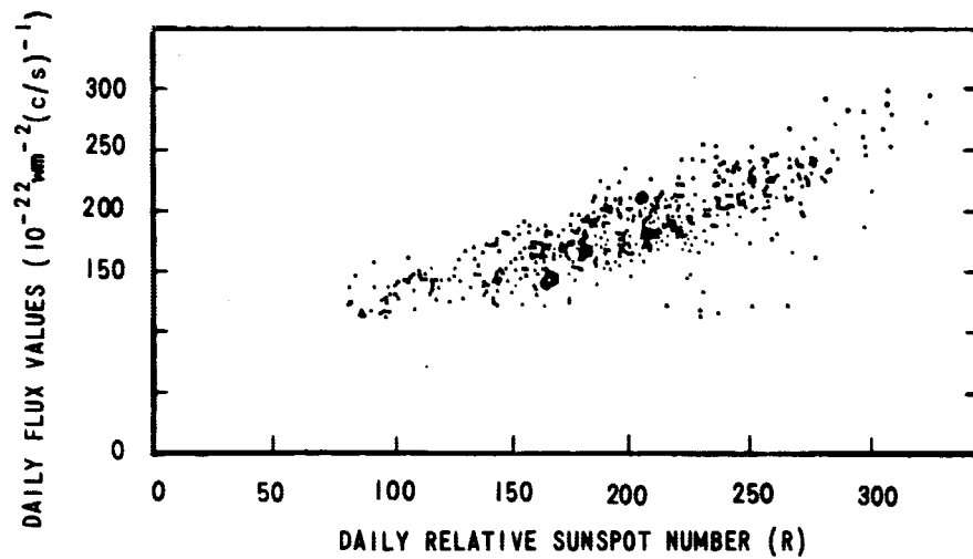
FIGURE 1A6 - RELATION BETWEEN FLUX DENSITY AT 10.7 CM AND THE SUNSPOT NUMBER FOR THE IGY PERIOD (FROM SMERD, 1964)
