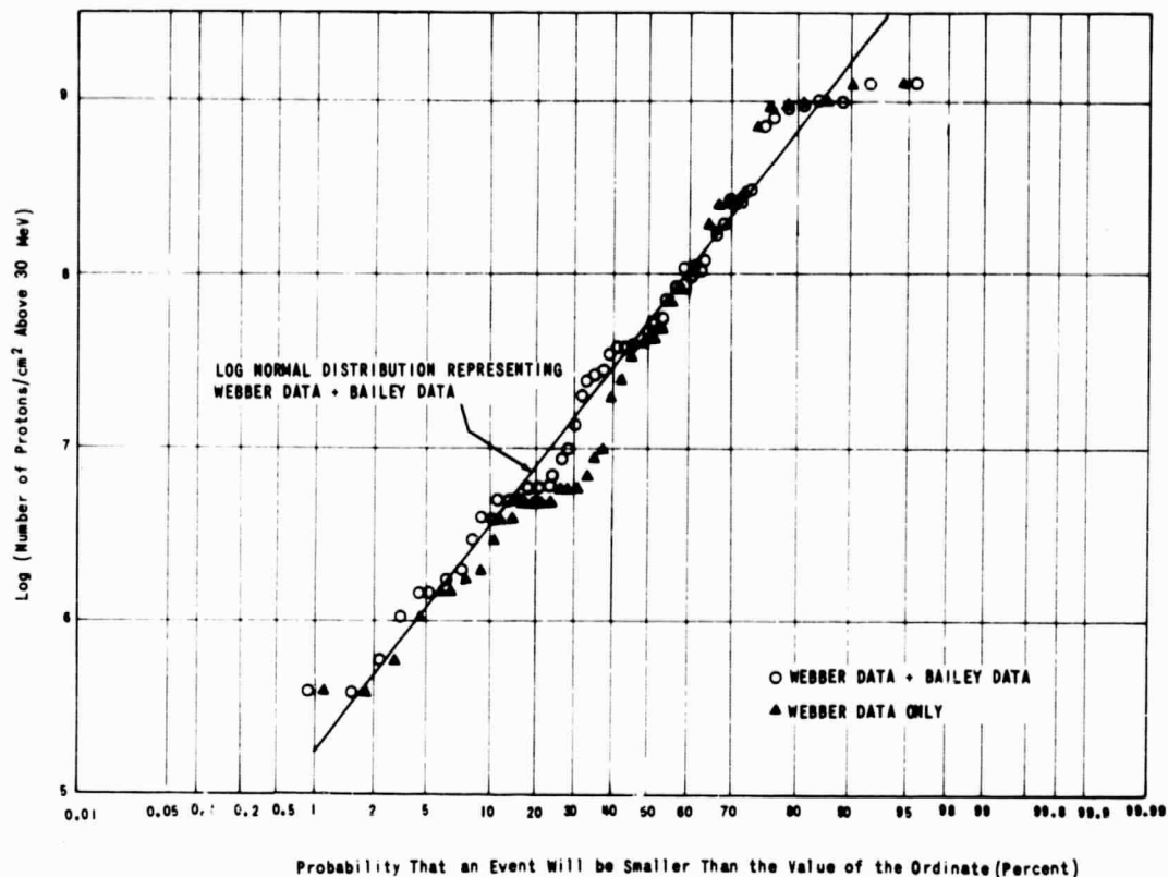
FIGURE ID5 - SIZE DISTRIBUTION OF SOLAR PARTICLE EVENTS OF 19TH SOLAR CYCLE ON NORMAL PROBABILITY PAPER (FROM MODISETTE, 1965)
