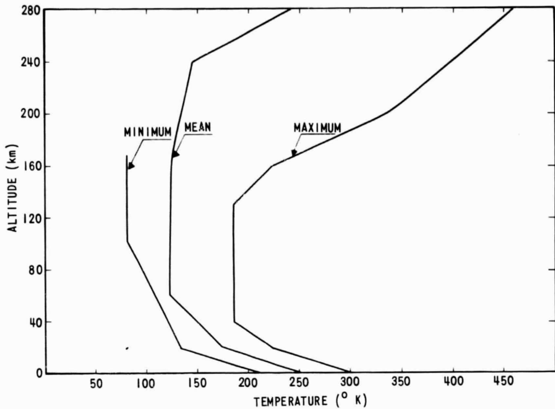
FIGURE IIC1 - ATMOSPHERIC TEMPERATURE PROFILE OF MARS (FROM NASA SP-8010)
