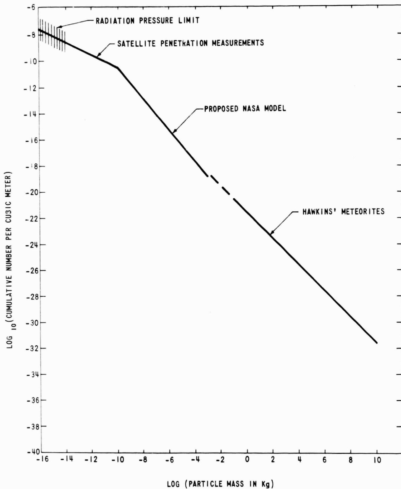
FIGURE IF1 - MASS DISTRIBUTION OF METEORIODS. CUMULATIVE NUMBER OF PARTICLES PER CUBIC METER OF SPACE HAVING A MASS m Kg OR GREATER AT A DISTANCE FROM THE SUN OF 1 AU
