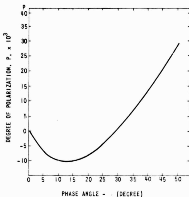
FIGURE IIA5 - AVERAGE POLARIZATION CURVE OF LIGHT REGIONS ON MARS (AFTER DOLLFUS, 1964)
