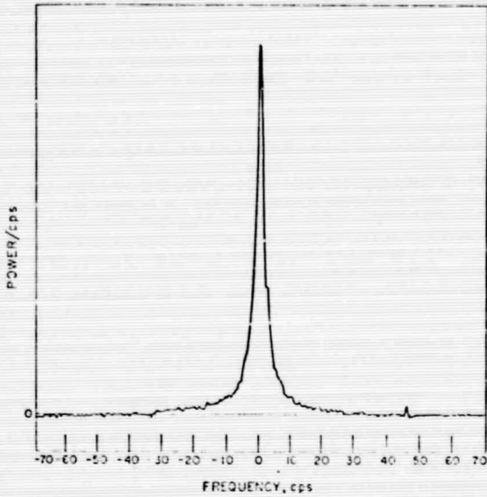
FIGURE 11IB1 - CW RADAR SPECTRUM OF VENUS FOR JULY 19, 1964. THE SPIKE AT +46 CPS IS A FREQUENCY CALIBRATION MARK. (FROM CARPENTER, 1966).
