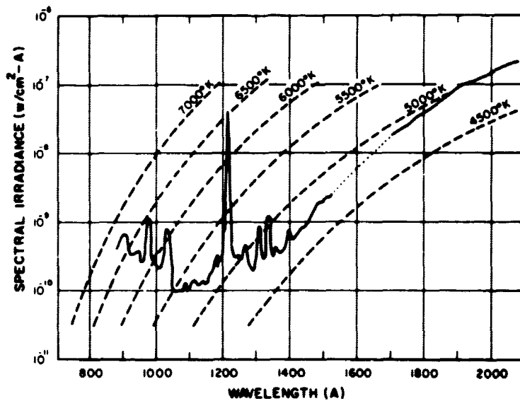
FIGURE IA4 - SOLAR ULTRAVIOLET IRRADIANCE AT 1 AU BETWEEN 700 AND 2100 Å (FROM JOHNSON, 1965)
