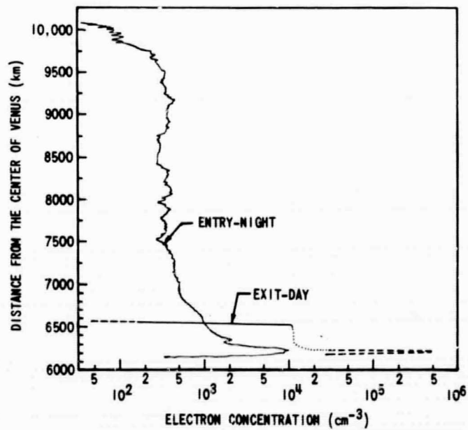
FIGURE IIIC4 - IONOSPHERIC ELECTRON PROFILES OF VENUS (AFTER MARINER STANFORD GROUP, 1967)
