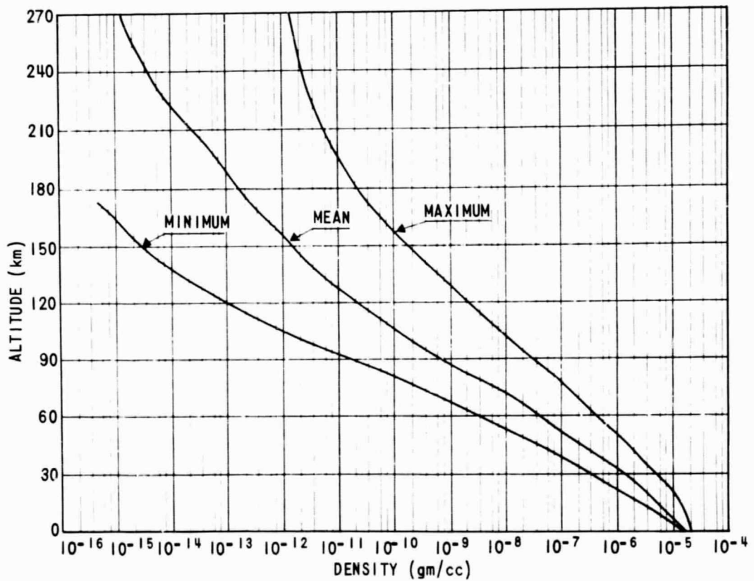
FIGURE IIC2 - ATMOSPHERIC DENSITY PROFILE OF MARS (FROM NASA SP-8010)
