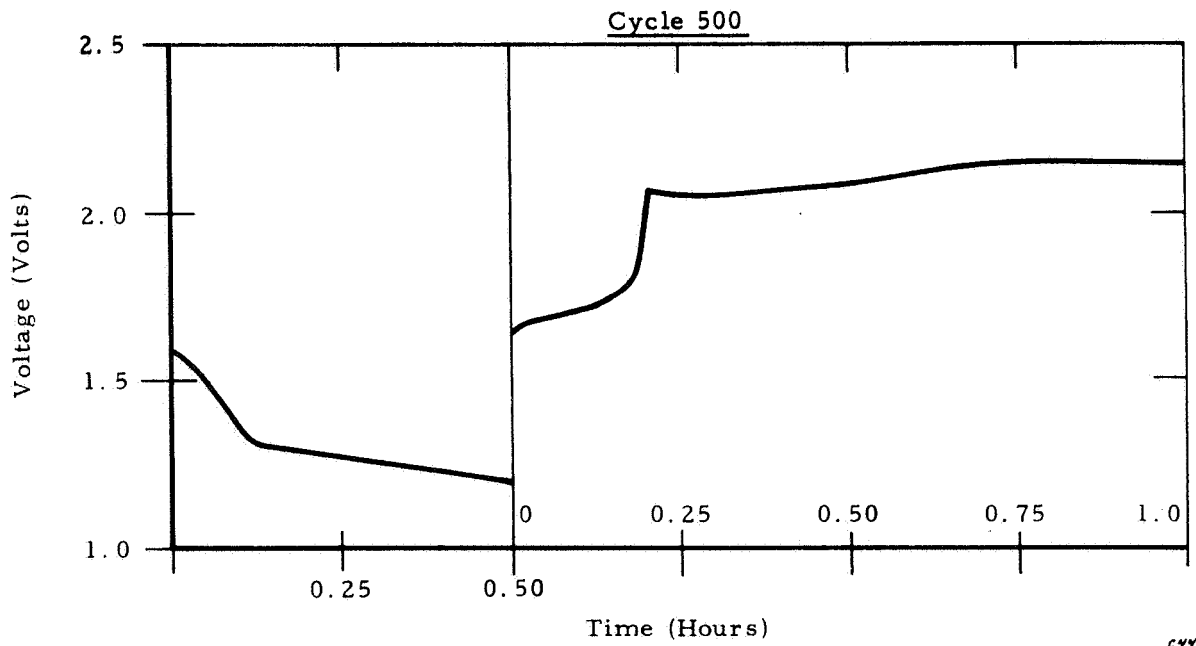
Figure 43. Group C (Pressure Gauge) Typical Cell
