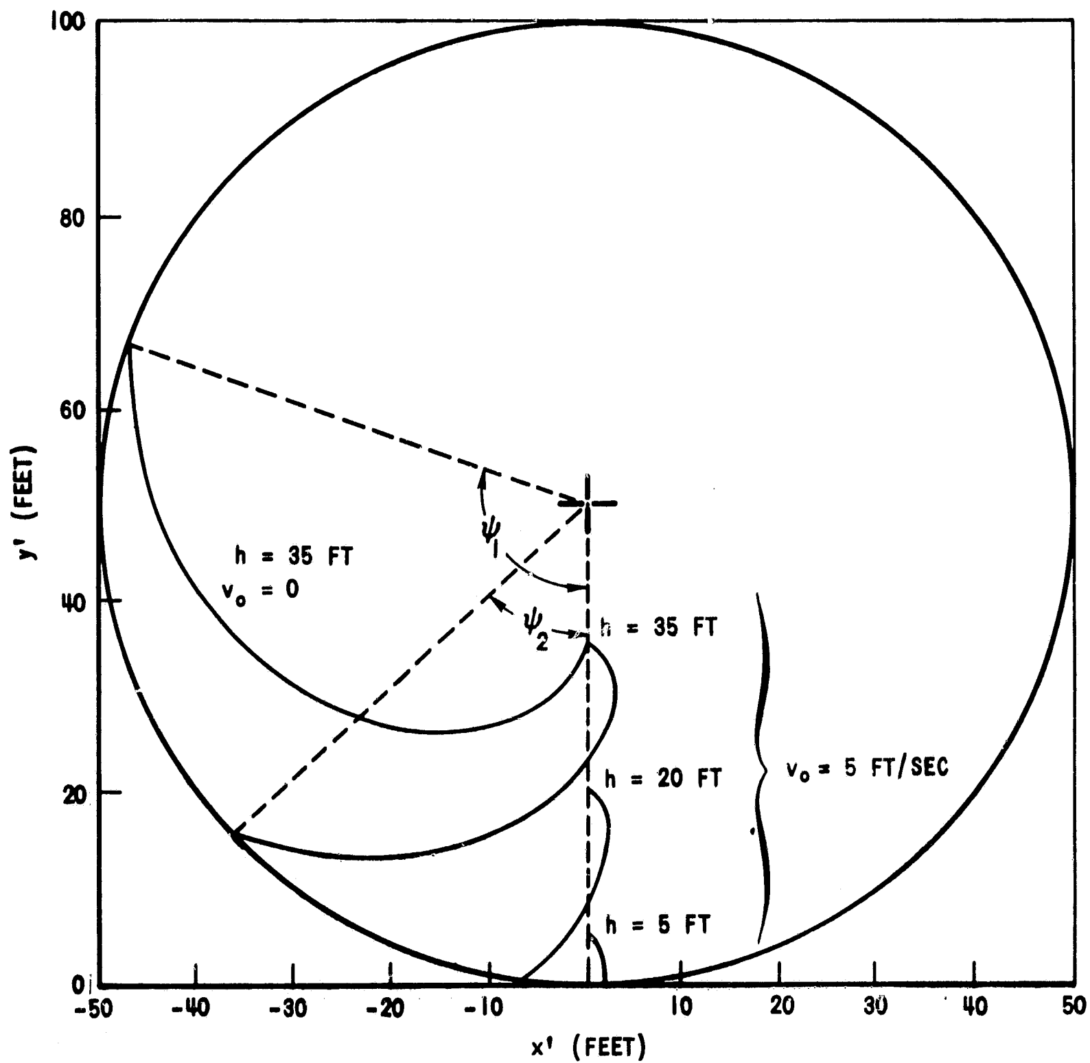
FIGURE 5 - THE EFFECT OF h ON PARTICLE TRAJECTORIES, FOR \alpha = 0 , v_0 = 0 , 5 FEET/SEC
