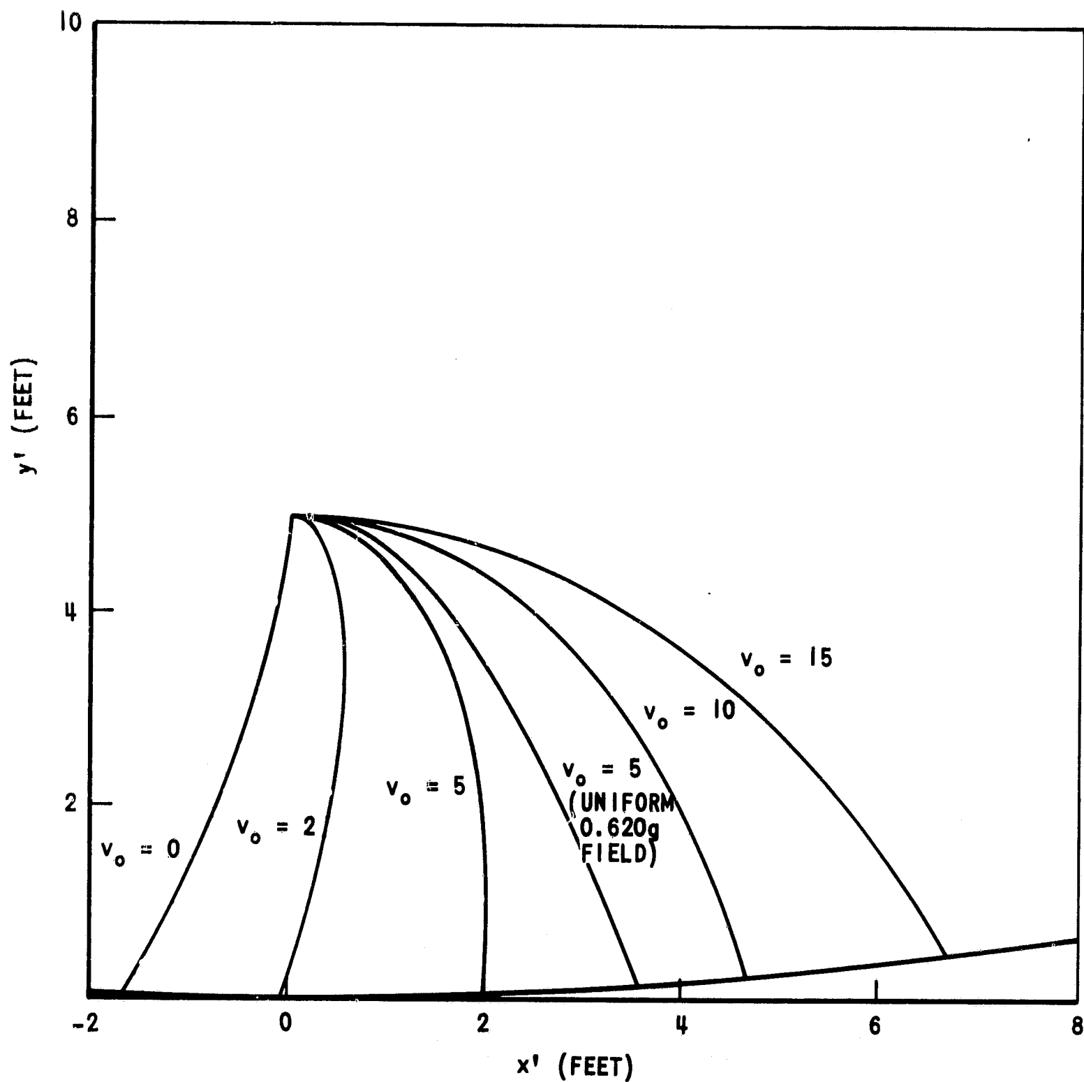
FIGURE 4 - THE EFFECT OF v_o ON PARTICLE TRAJECTORIES FOR \alpha = 0 , h = 5 FEET
