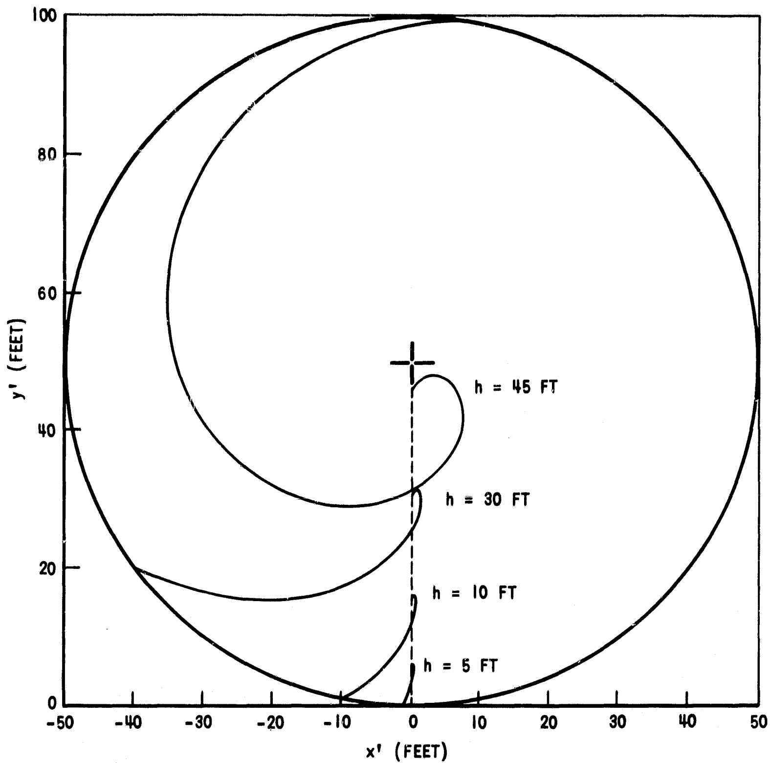
FIGURE 9 - THE EFFECT OF h ON PARTICLE TRAJECTORIES FOR \alpha = 90^\circ , v_o = 5 FT/SEC
