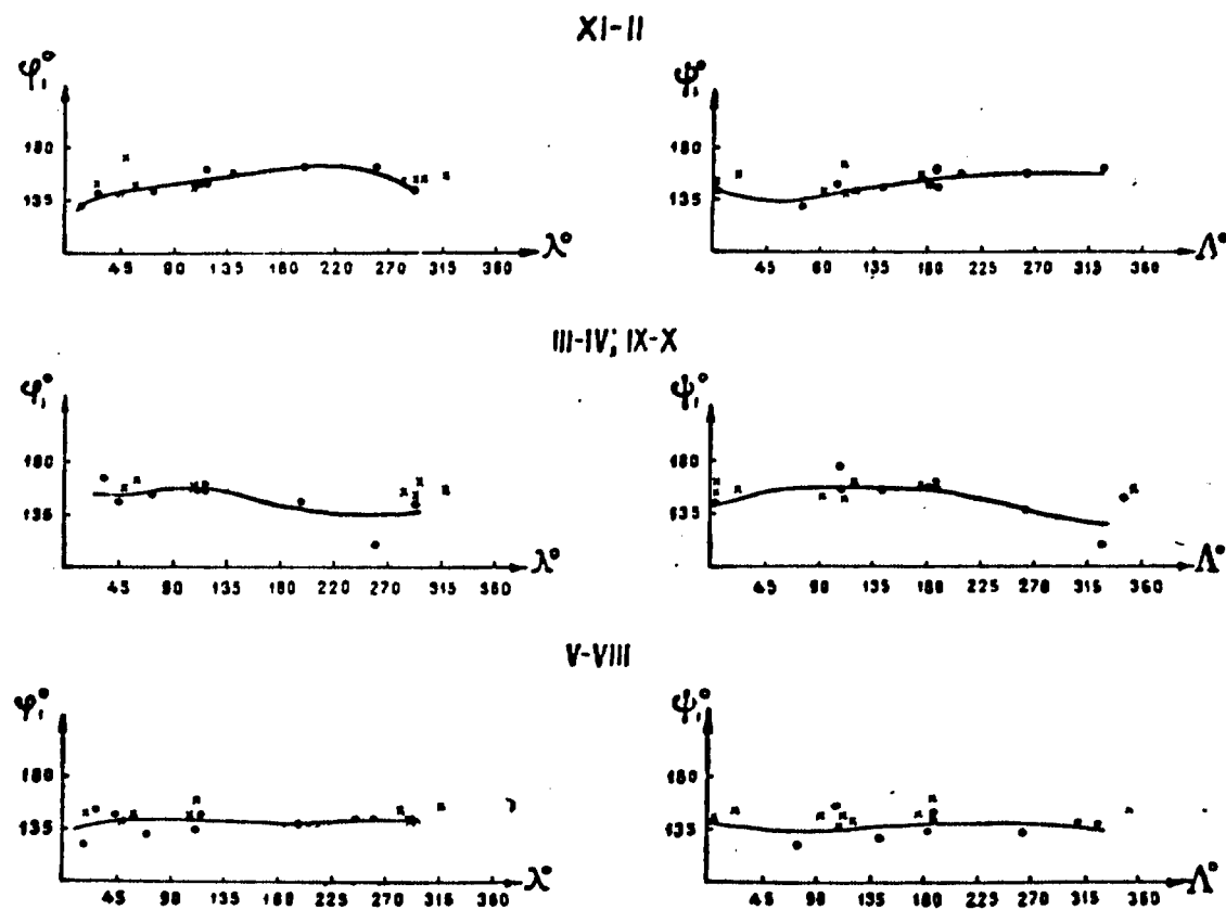
Fig. 6. Longitudinal variations of the maximum phase of the first harmonic Sq ( \delta' F ) by stations located toward the pole away from the focus, during the XI-II; III-IV; IX-X; V-VIII, 1933 seasons
