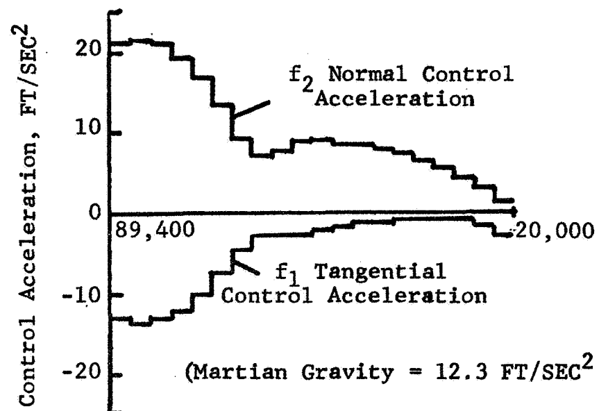
FIGURE 4 Control Accelerations vs. Altitude
