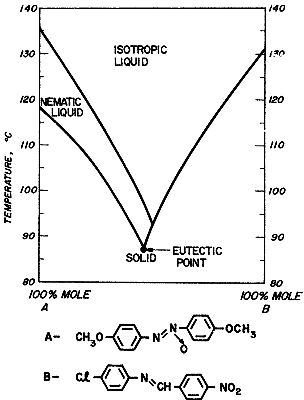
Figure 7. Phase diagram of binary mixture of nematic compound with non-mesomorphic compound.
