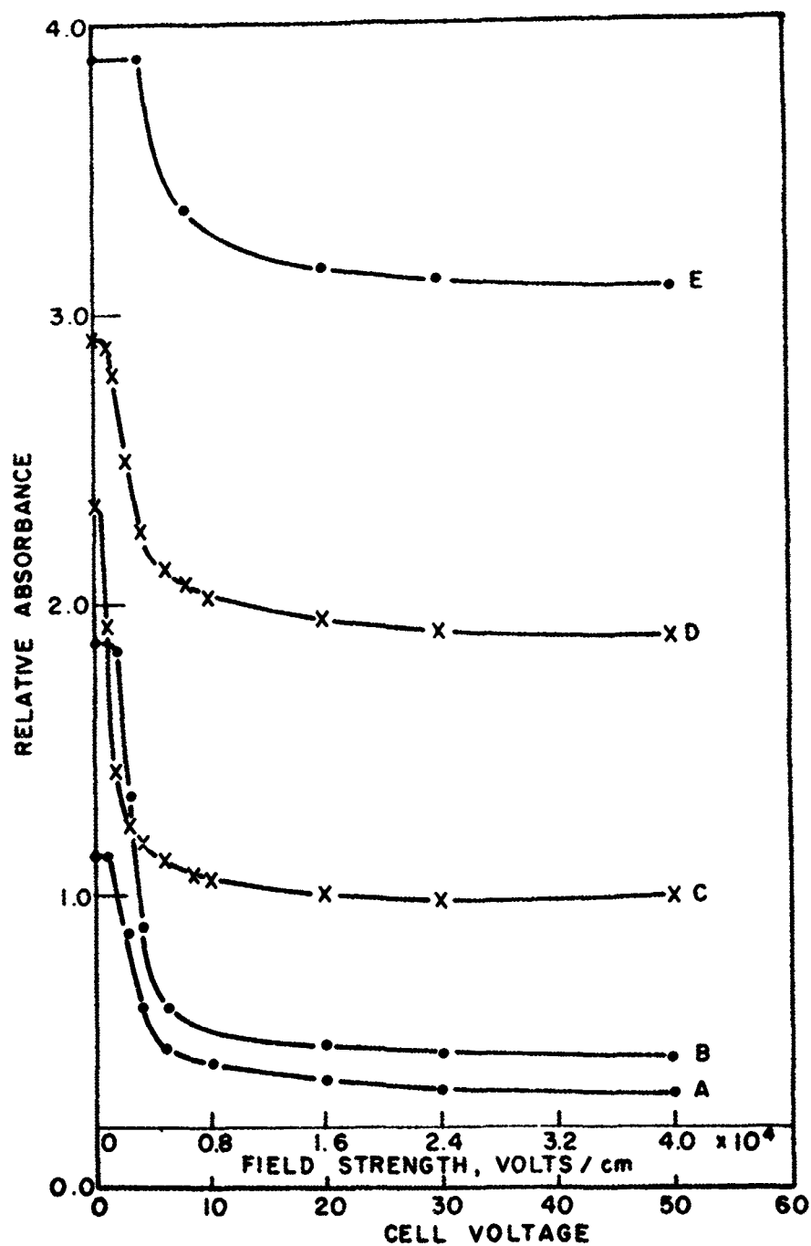
Figure 14. Changes in absorbance as a function of field strength for mixtures of PEBAB-RT and A - 0.5%, B - 1.0%, C - 1.5%, D - 2.5% and E - 5.0% of indophenol blue (cell thickness 12.5 microns).
