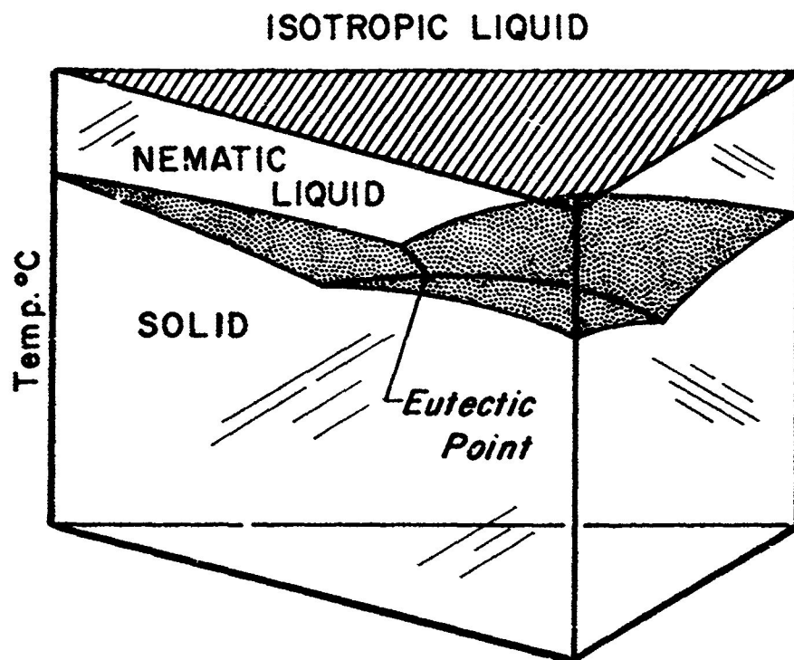
Figure 10. Phase diagram of a ternary PABAB mixture.
